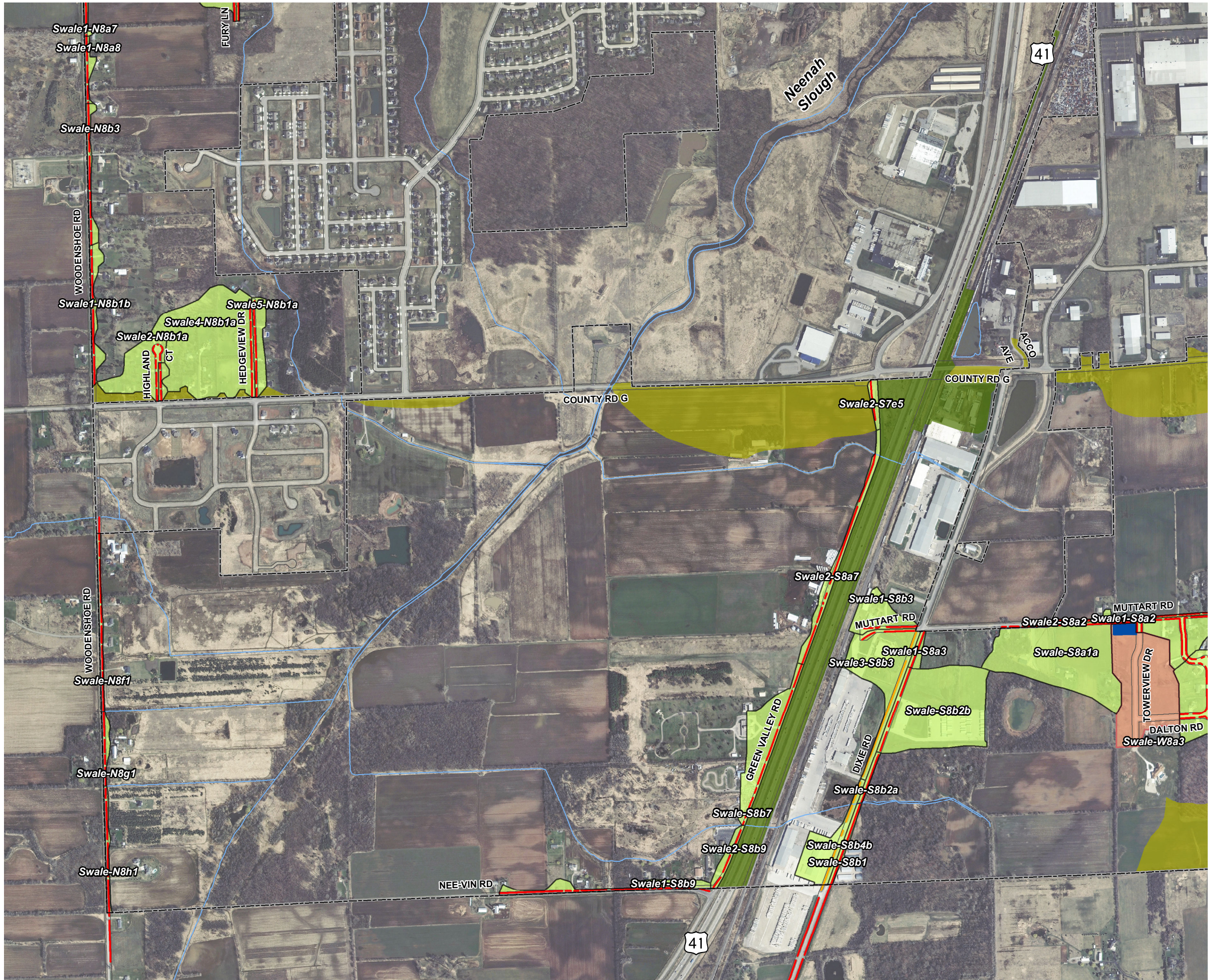
FIGURE I-8c SWALE CATEGORIES STORMWATER MANAGEMENT PLAN TOWN OF NEENAH WINNEBAGO COUNTY, WISCONSIN
