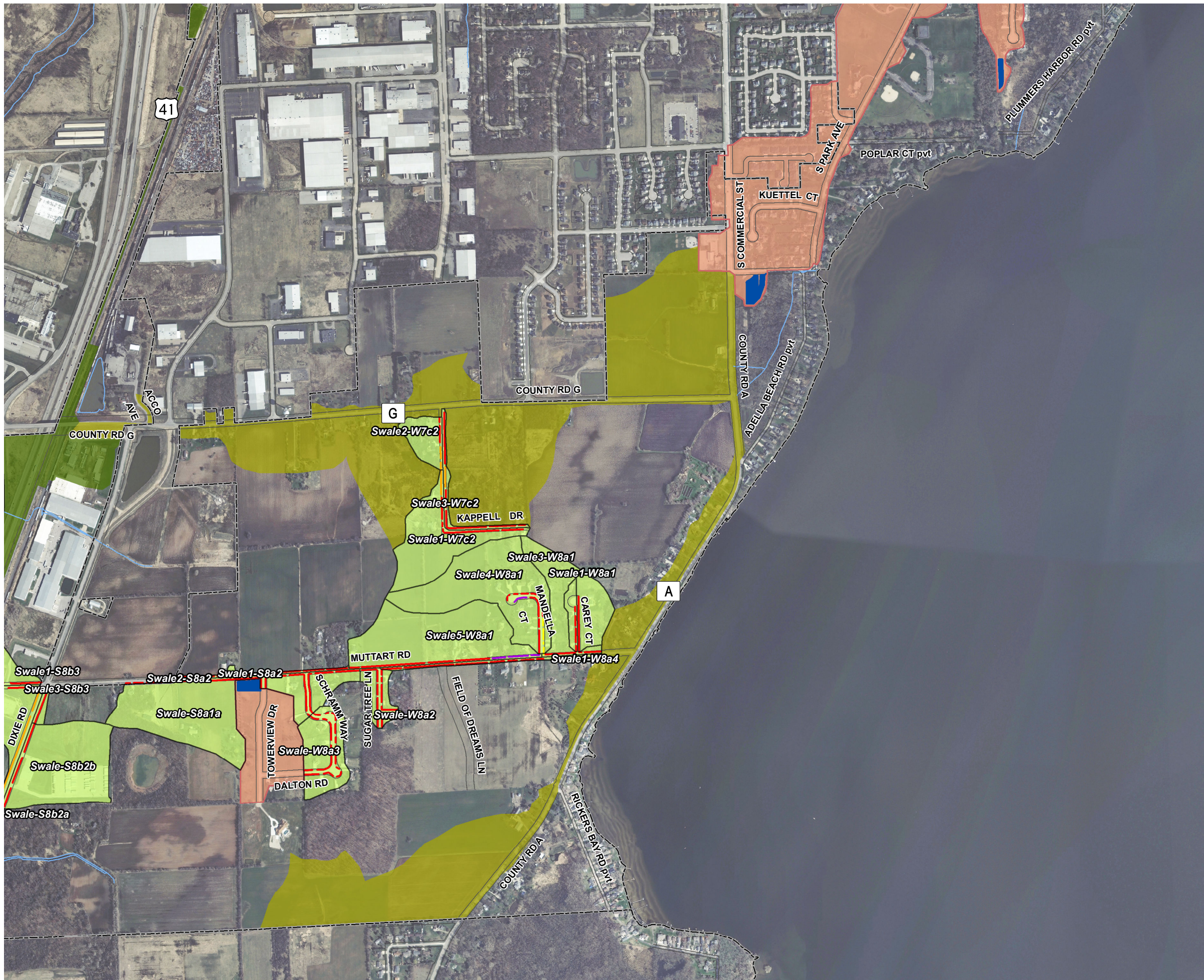
FIGURE I-8d SWALE CATEGORIES STORMWATER MANAGEMENT PLAN TOWN OF NEENAH WINNEBAGO COUNTY, WISCONSIN
