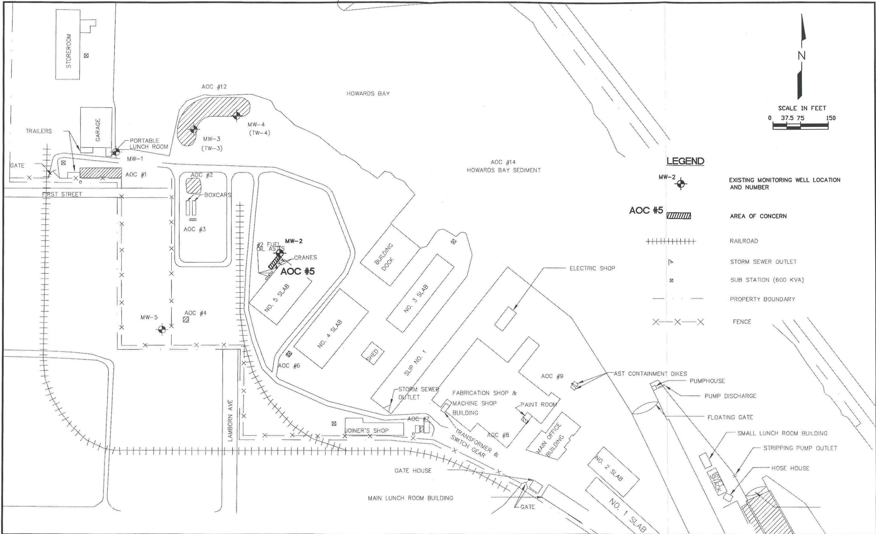
FIGURE 2 SITE PLAN
