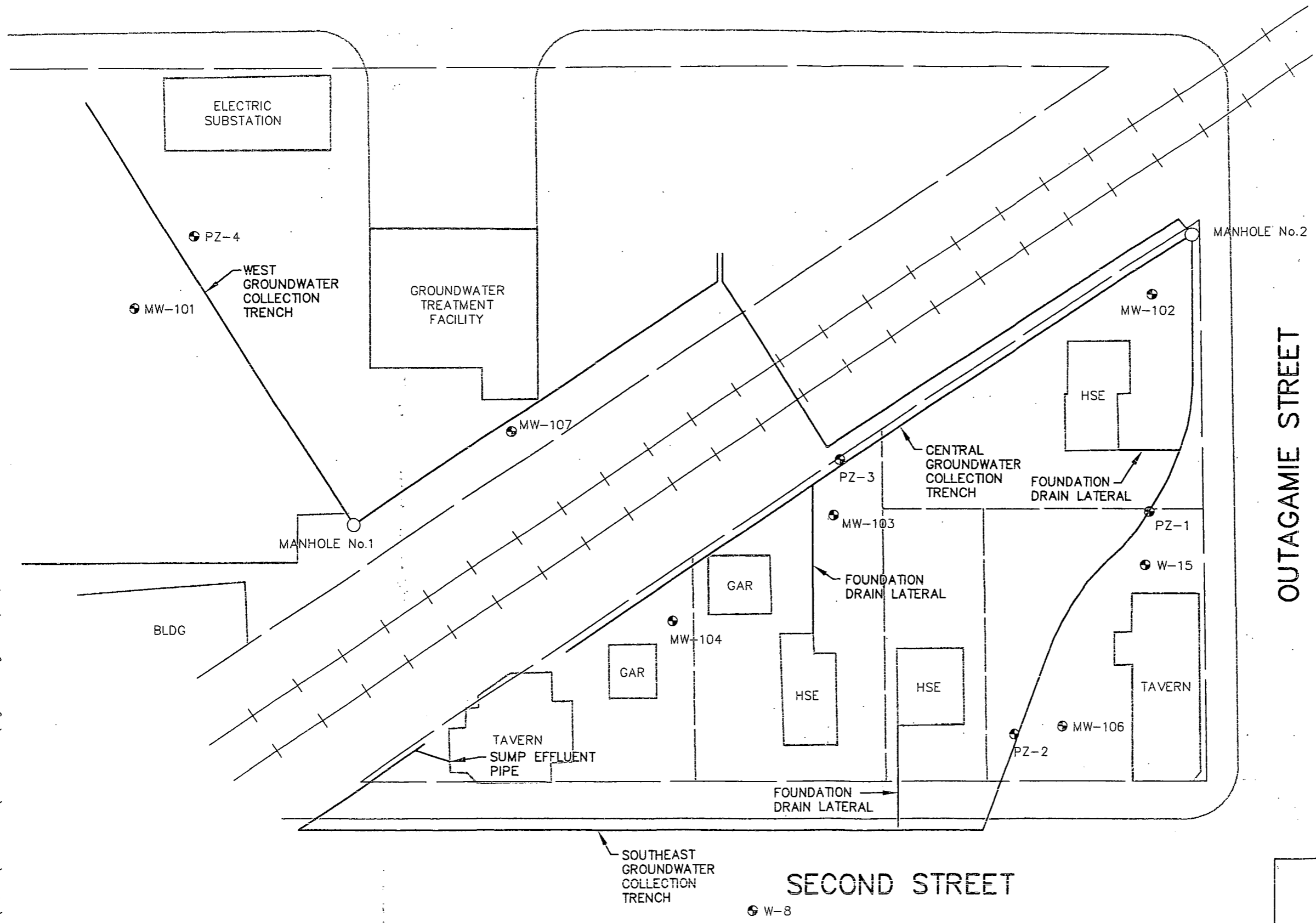
FIGURE 2 COLLECTION TRENCH AND MONITORING WELL LOCATIONS N.W. MAUTHE SUPERFUND SITE
