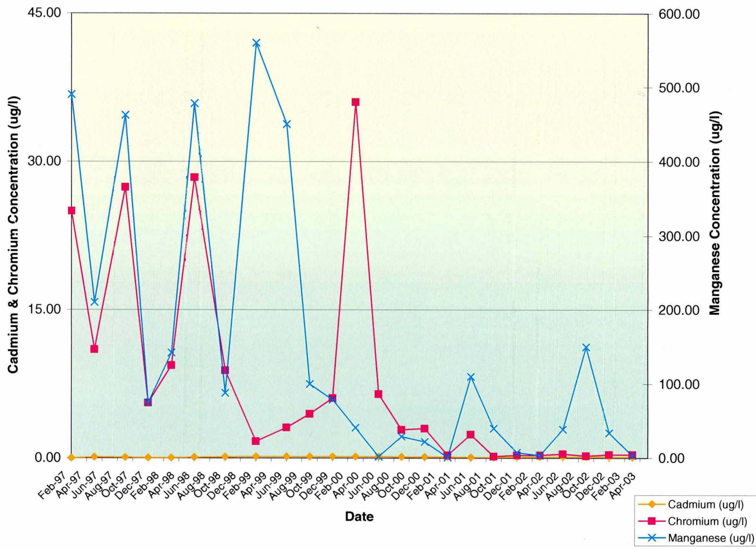
Well W-108 / Concentration Vs. Time
