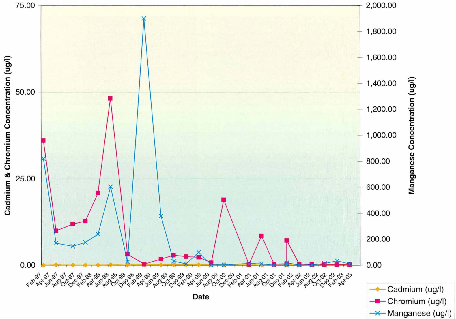
Well W-101 / Concentration Vs. Time
