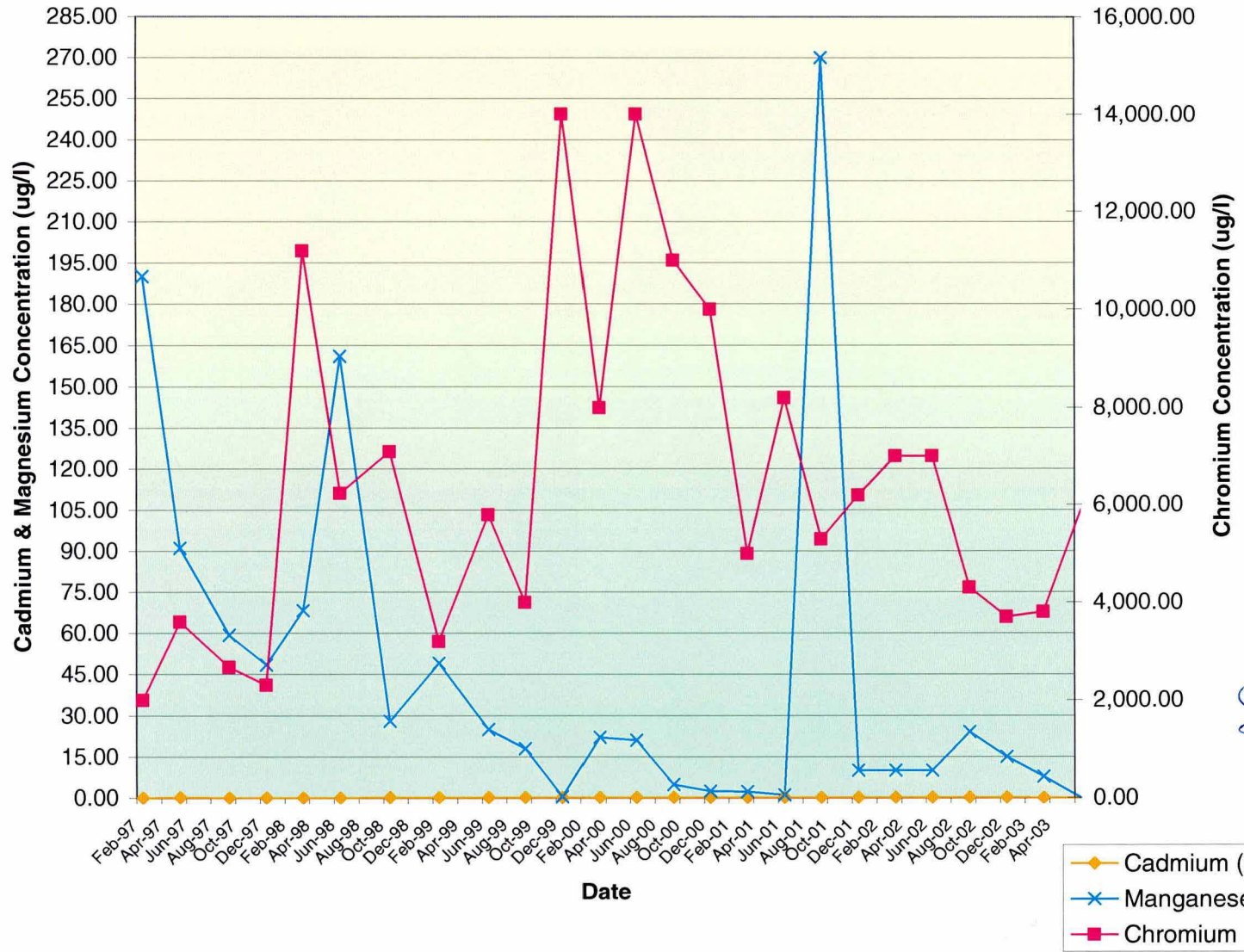
Well W-107 / Concentration Vs. Time
