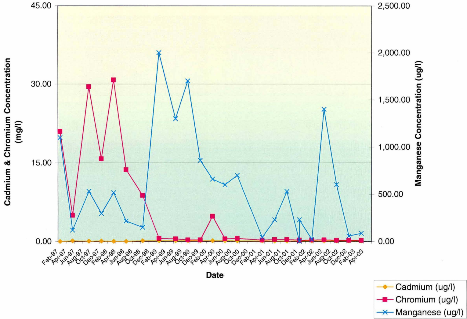
Well W-105 / Concentration Vs. Time
