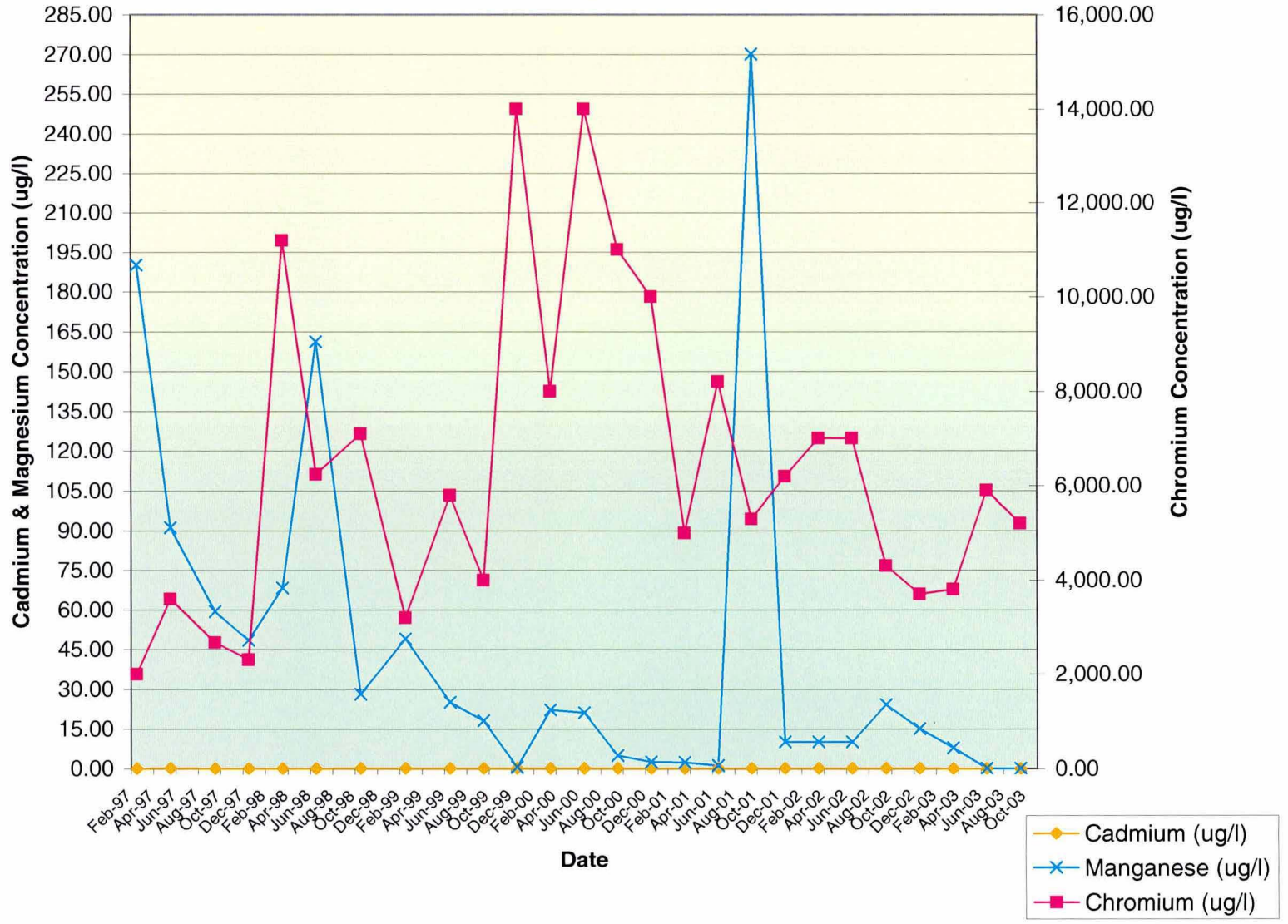
Well W-107 / Concentration Vs. Time
