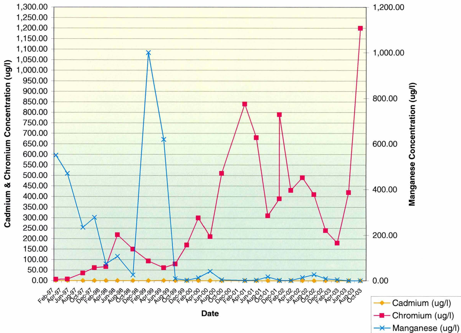
Well W-104 / Concentration Vs. Time
