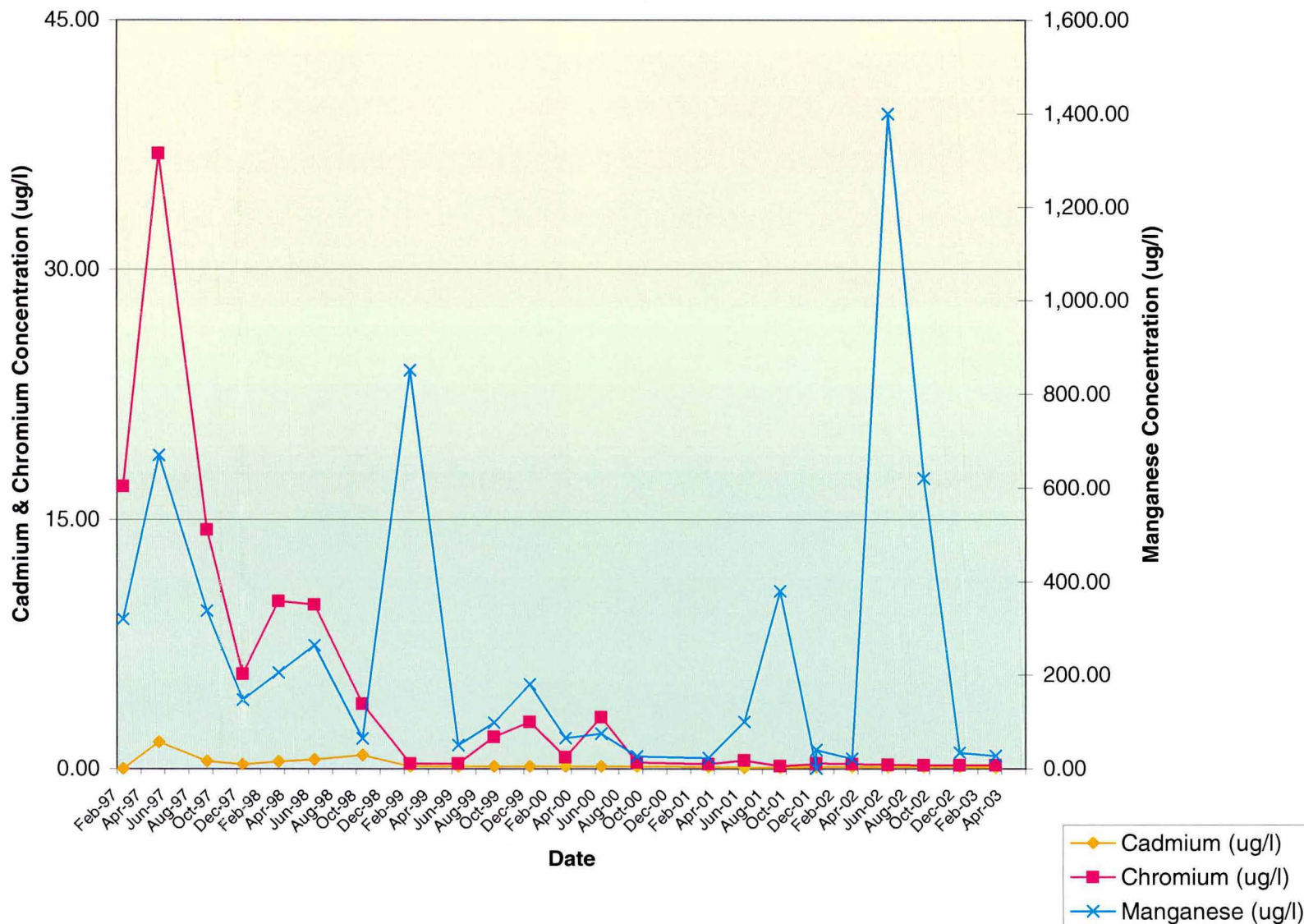
Well W-8 / Concentration Vs. Time
