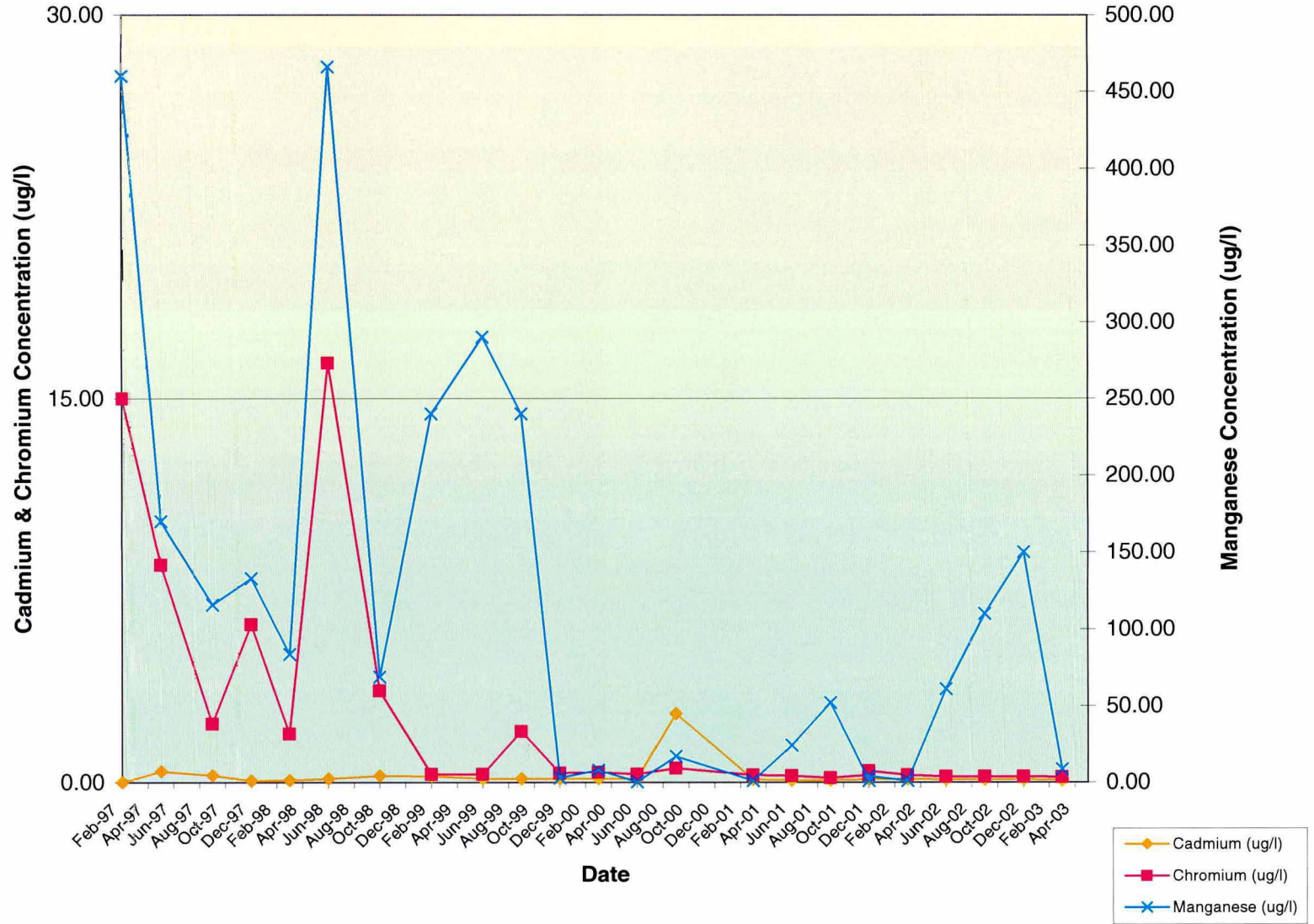
Well W-2 / Concentration Vs. Time
