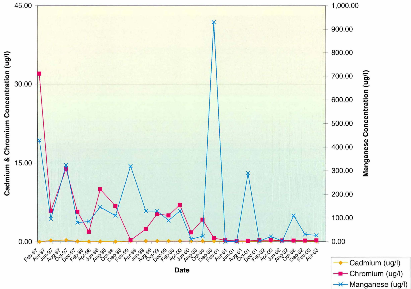
Well W-15 / Concentration Vs. Time
