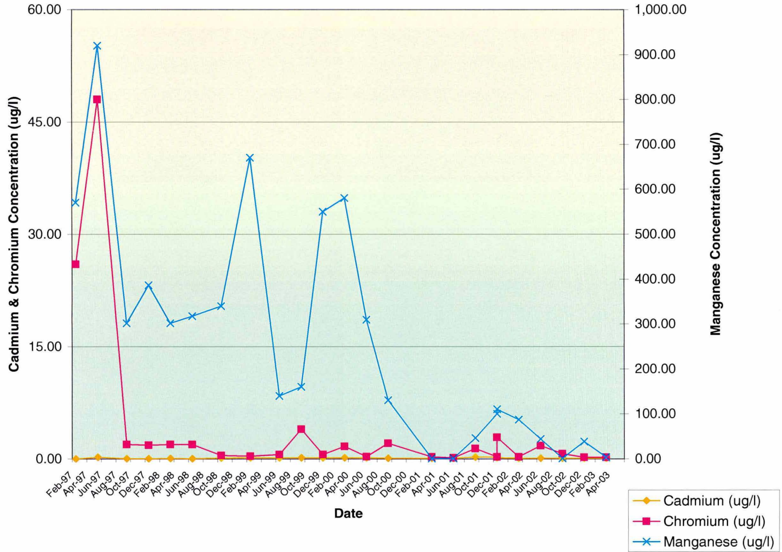
Well W-102 / Concentration Vs. Time
