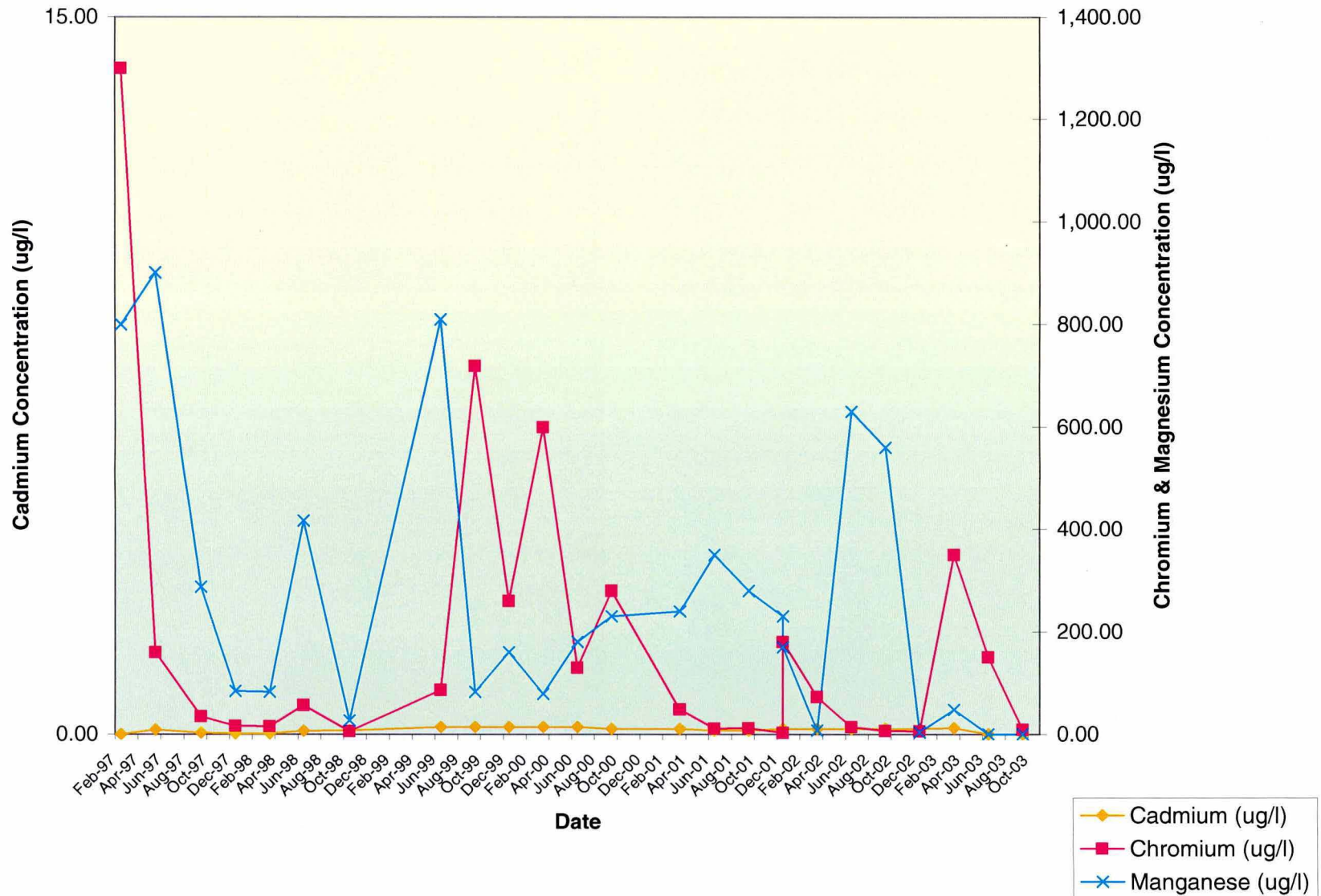
Well W-103 / Concentration Vs. Time
