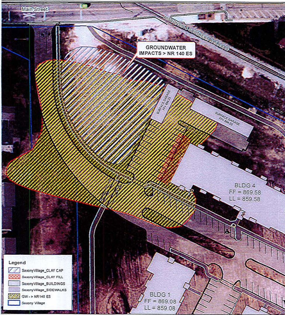
Figure 5: Barrier Installations for Groundwater Contamination
