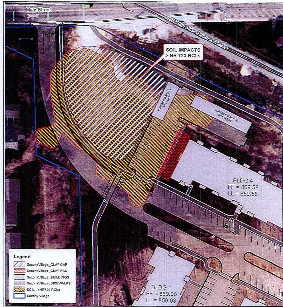
Figure 4: Barrier Installations for Soil Contamination
