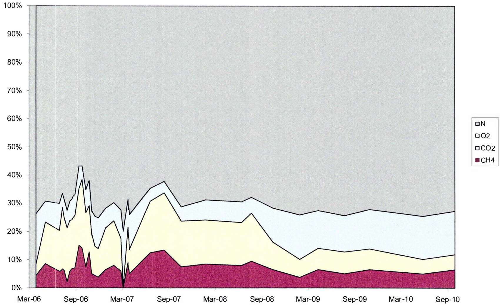
Chart 4-14: System Exhaust
