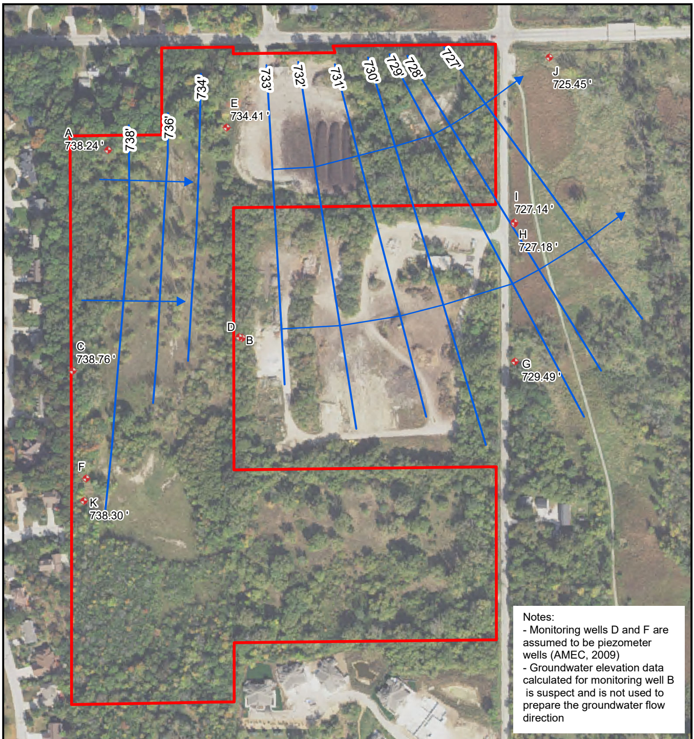
FIGURE 3 - WATER TABLE ELEVATION DATA, 7/9/2018 & 9/25/18
