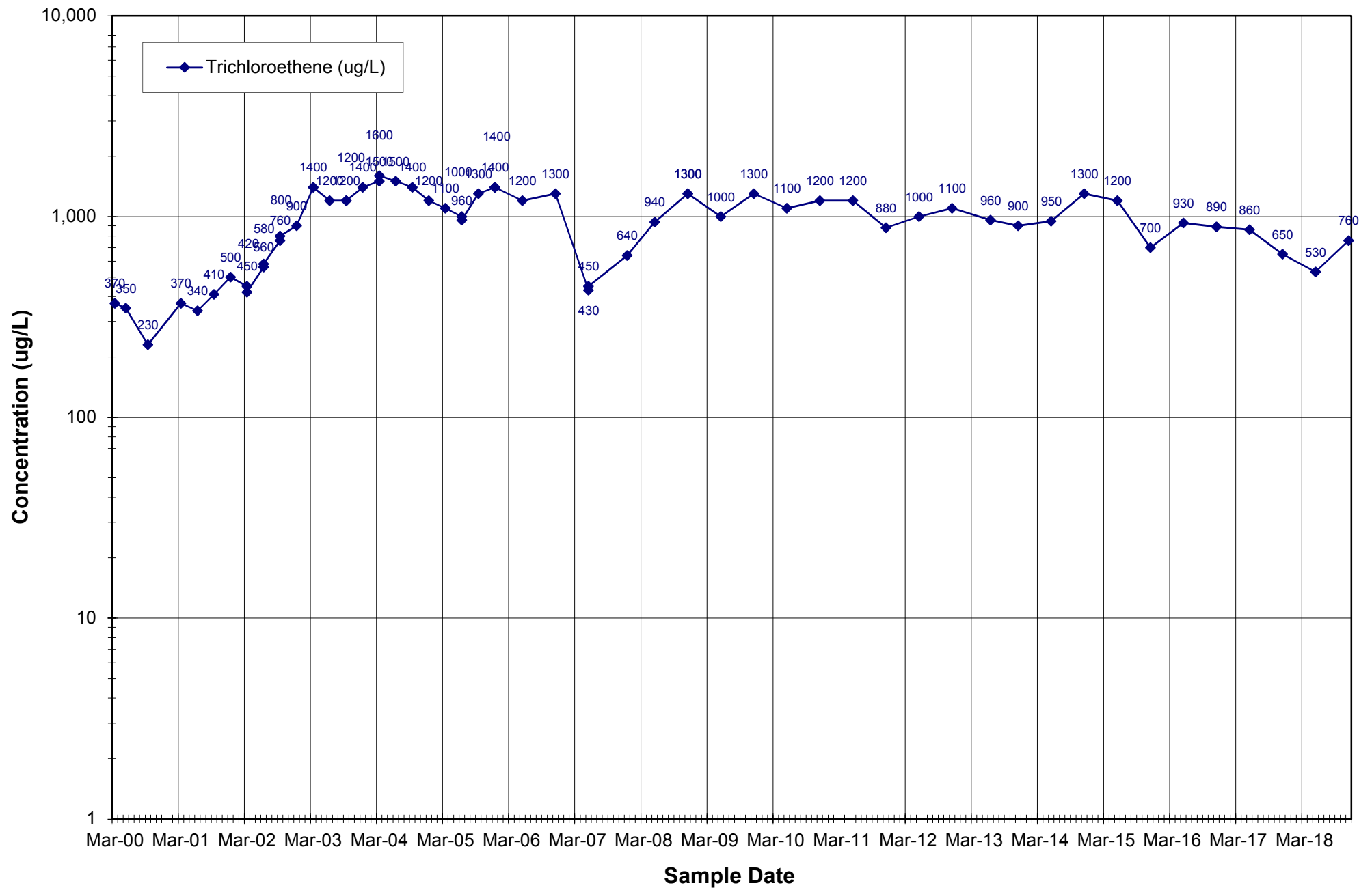
Monitor Well MW-17D Groundwater Chemistry Time Series Chart
