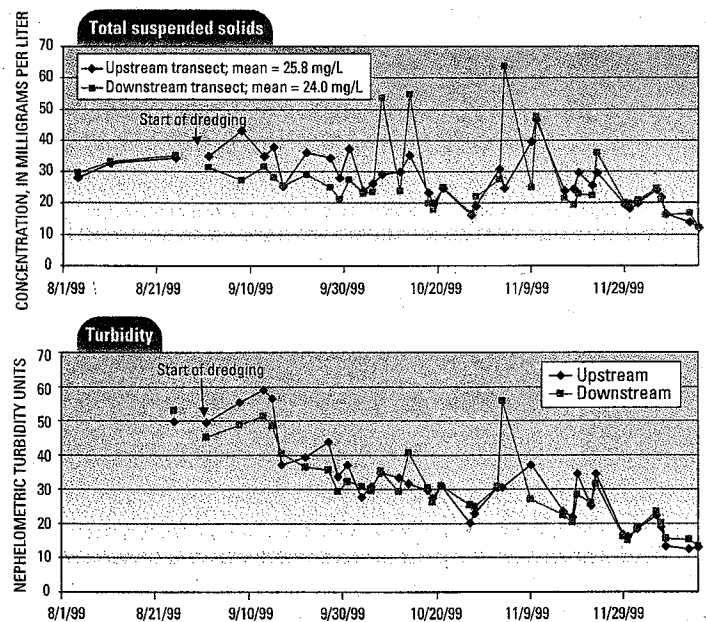
Figure 5. Daily mean total suspended solids concentrations and turbidity values for the upstream and downstream transects, Fox River, Wis.
