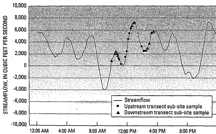
Figure 4. Fox River streamflow and sample-collection times on December 13, 1999.
