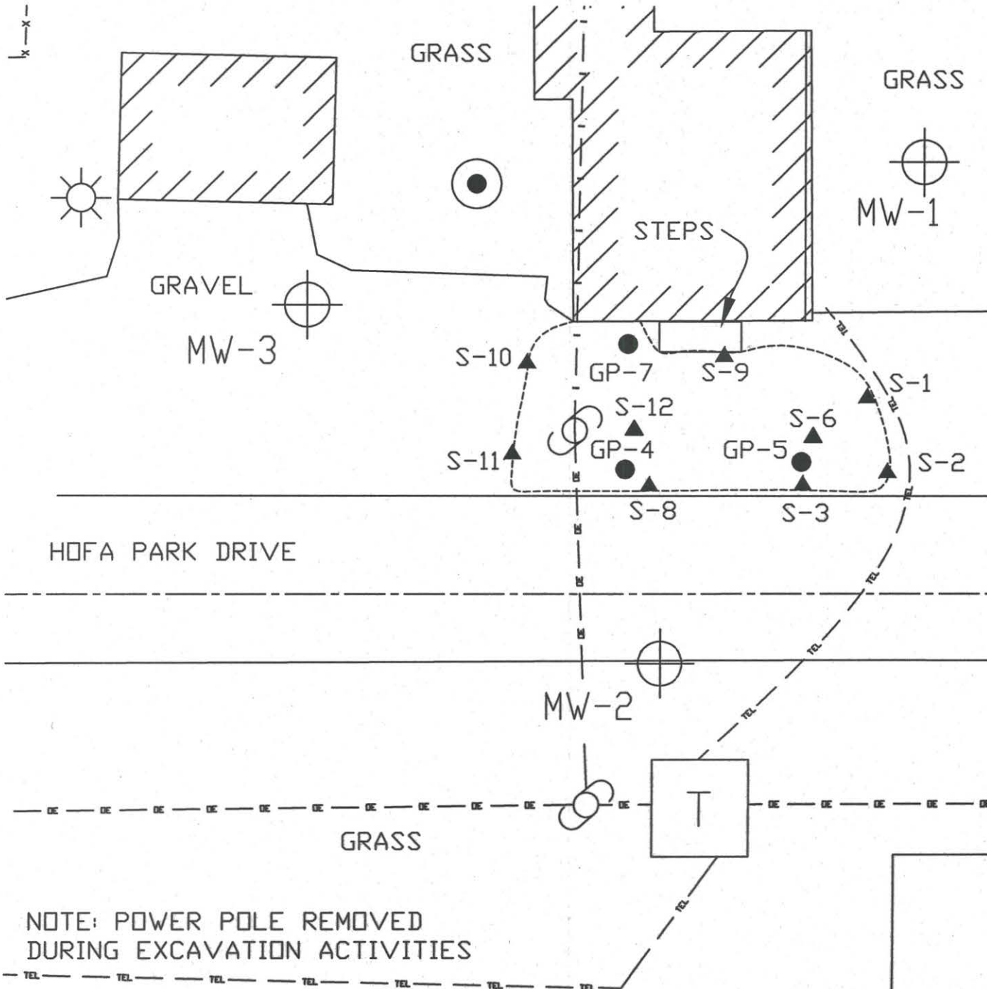
FIGURE 2 EXCAVATION EXTENT DA SWAMP BAR SEYMOUR, WISCONSIN
