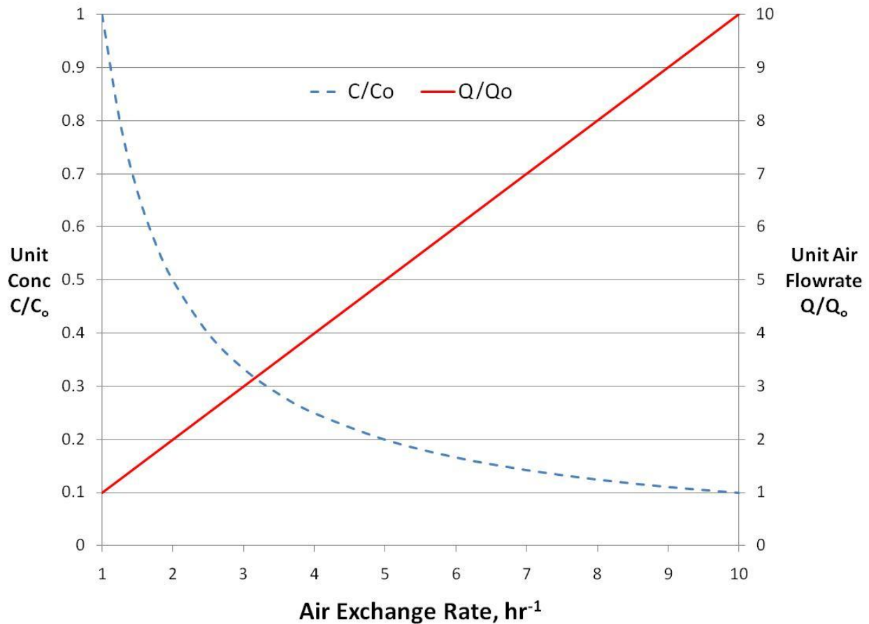
Figure 2: Influence of outdoor air exchange rate on indoor air concentration.
