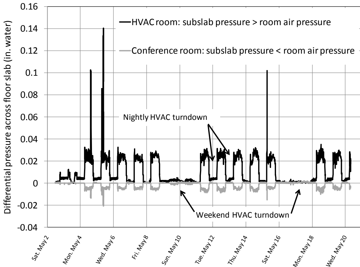
Figure 4. HVAC influence on subslab pressure differentials across the floor slab.
