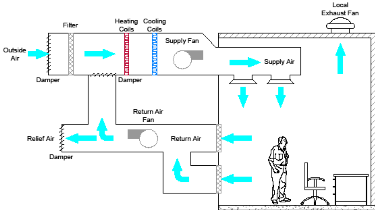
Figure 1: Schematic of typical commercial/industrial “all-air” HVAC system.
