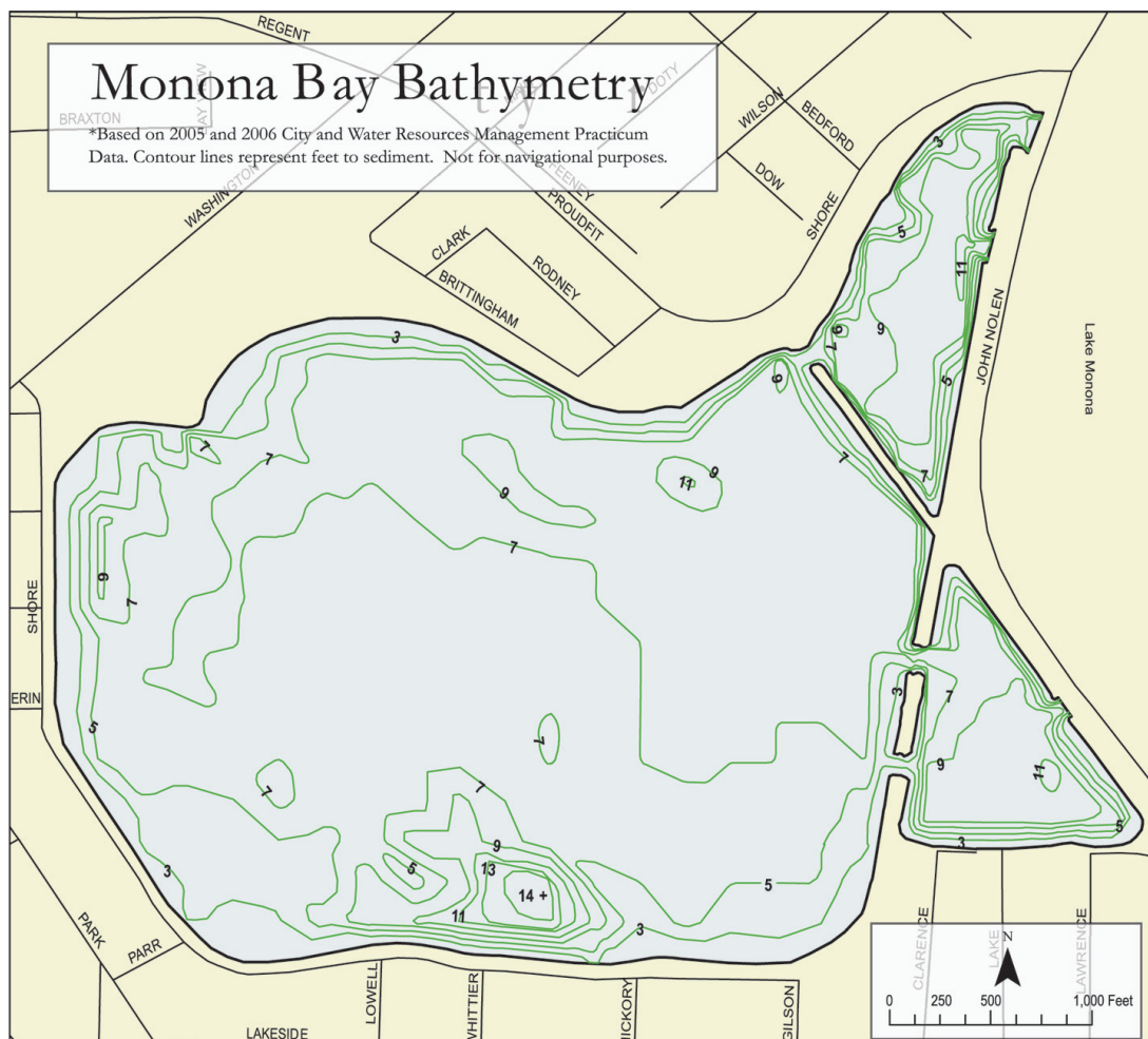
Figure 3.1. Monona Bay bathymetric map.
