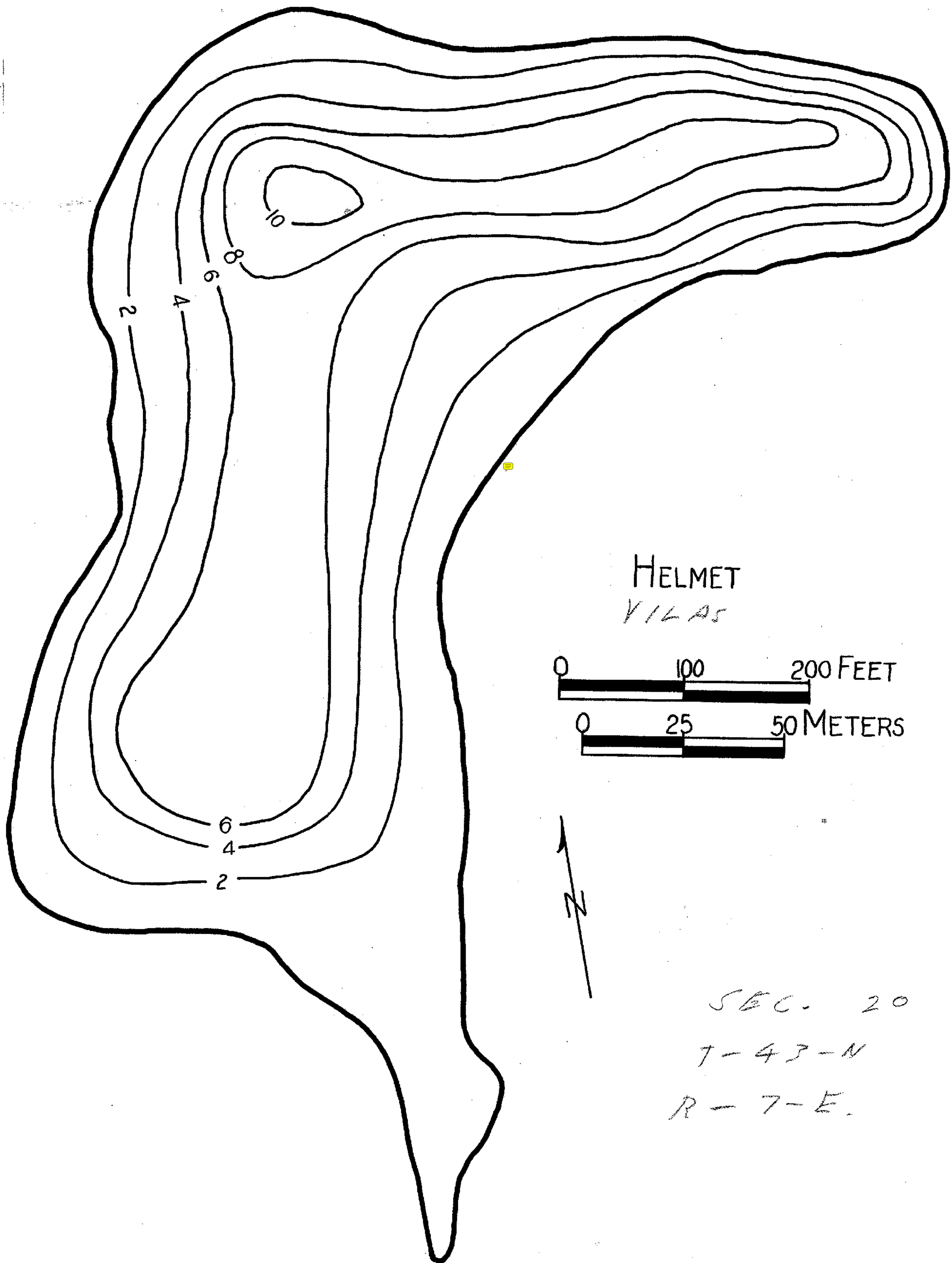
Fig. 11. Hydrographic map of Helmet Lake;
