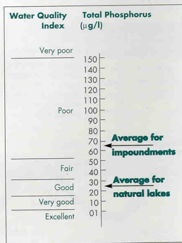
Figure 9. Total phosphorus concentrations for Wisconsin’s natural lakes and impoundments (Shaw et al., 2004).
