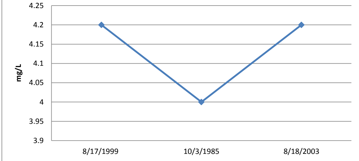
Figure 14. Round Lake magnesium.
