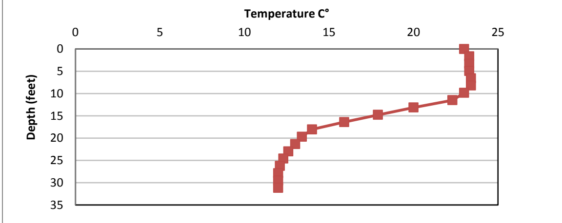
Figure 3. Round Lake temperature profile July, 2010.
