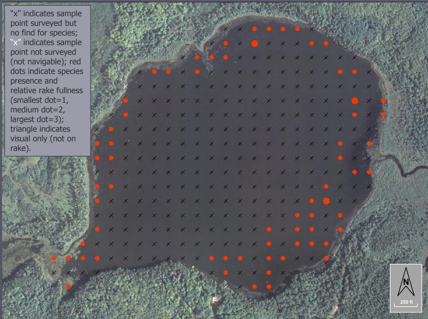
Figure 7. Distribution of plant species, Round Lake (2010)
