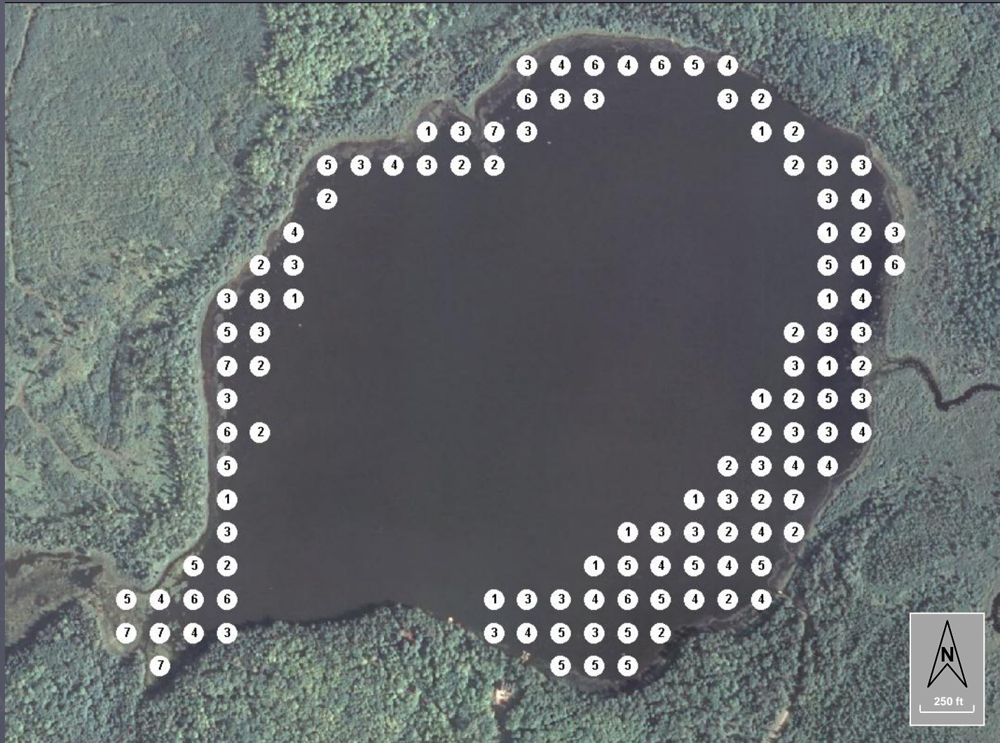
Figure 1. Number of plant species recorded at Round Lake sample sites (2010).
