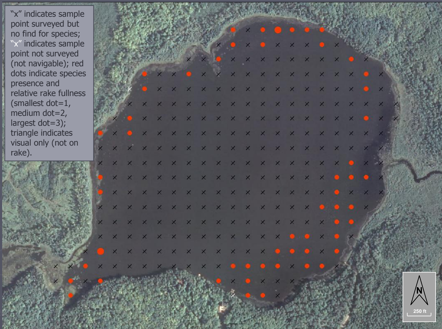
Figure 9. Distribution of plant species, Round Lake (2010)
