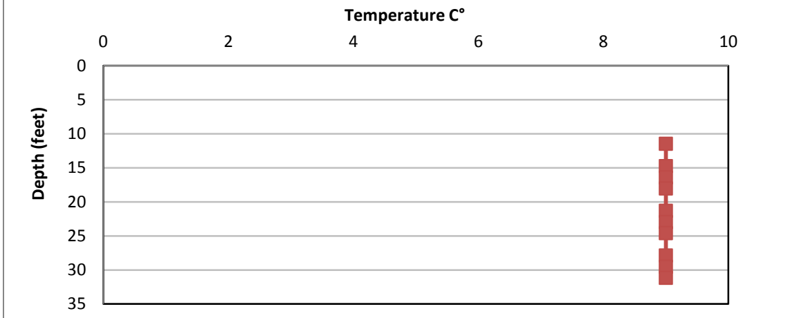
Figure 2. Round Lake temperature profile October, 1985.
