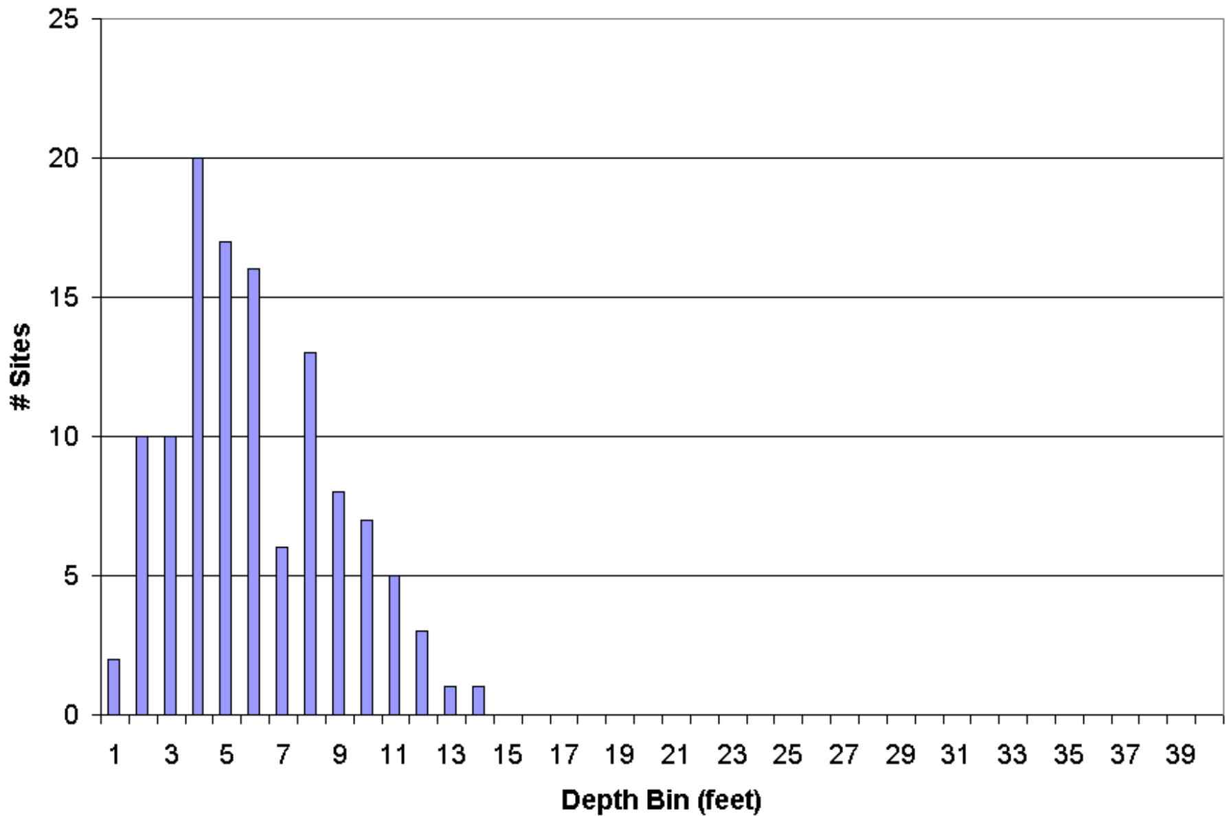
Figure 3. Maximum Depth of Plant Colonization in Round Lake.
