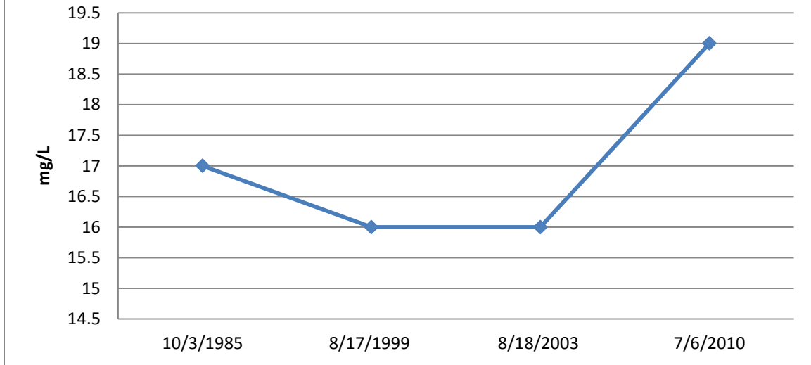
Figure 13. Round Lake calcium.
