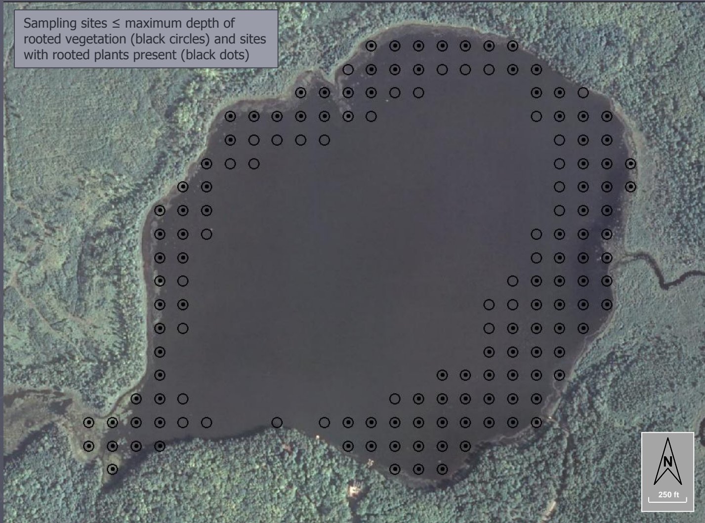
Figure 4. Round Lake sampling sites less than or equal to maximum depth of rooted vegetation (2010).
