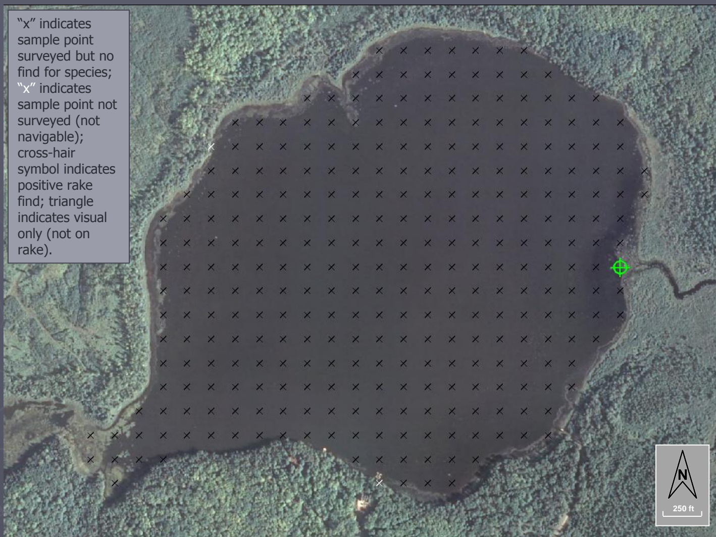
Figure 11. Distribution of plant species, Round Lake (2010)
