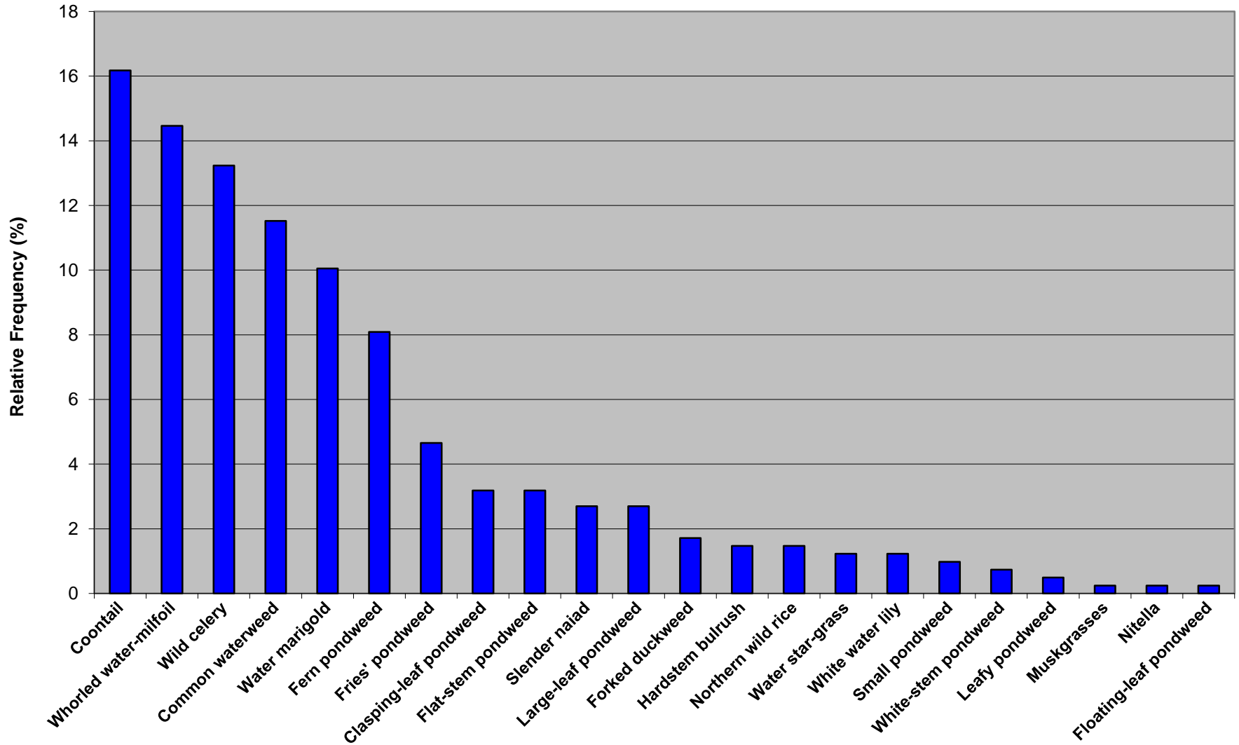
Figure 6. Round Lake aquatic plant occurrences for 2010 point-intercept survey data.
