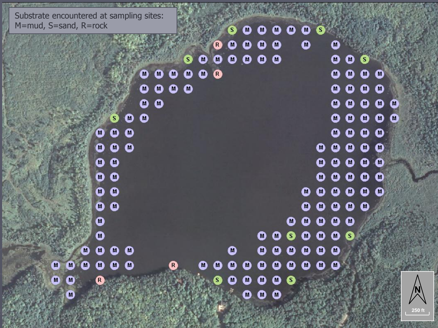
Figure 5. Round Lake substrate encountered at point-intercept plant sampling sites (2010).
