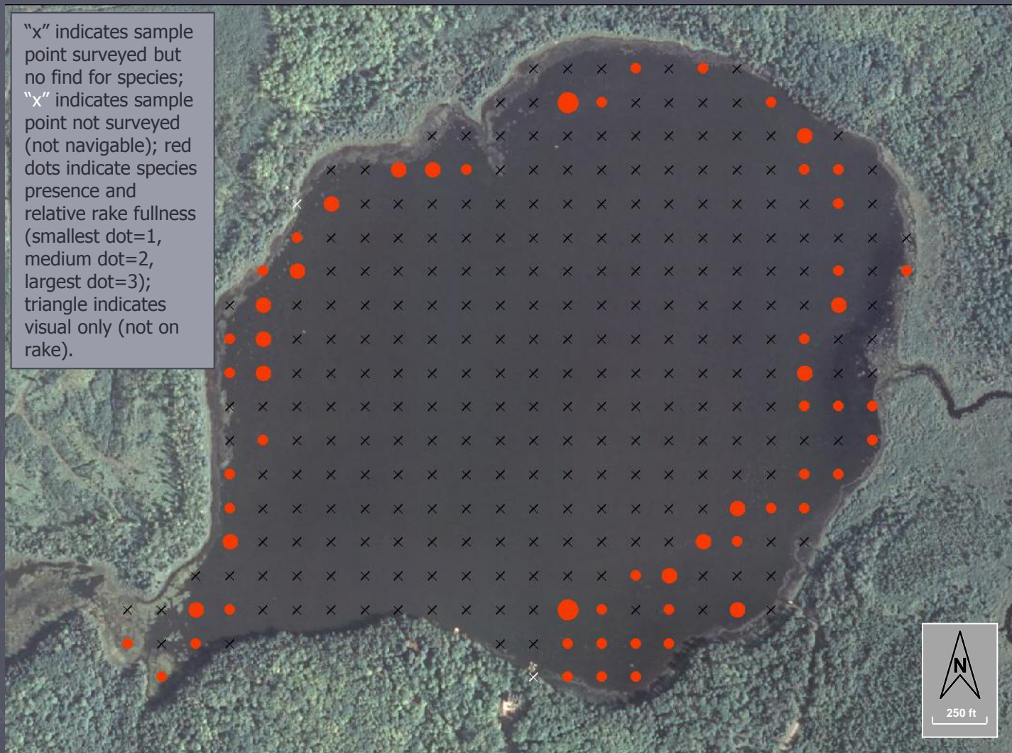
Figure 8. Distribution of plant species, Round Lake (2010)
