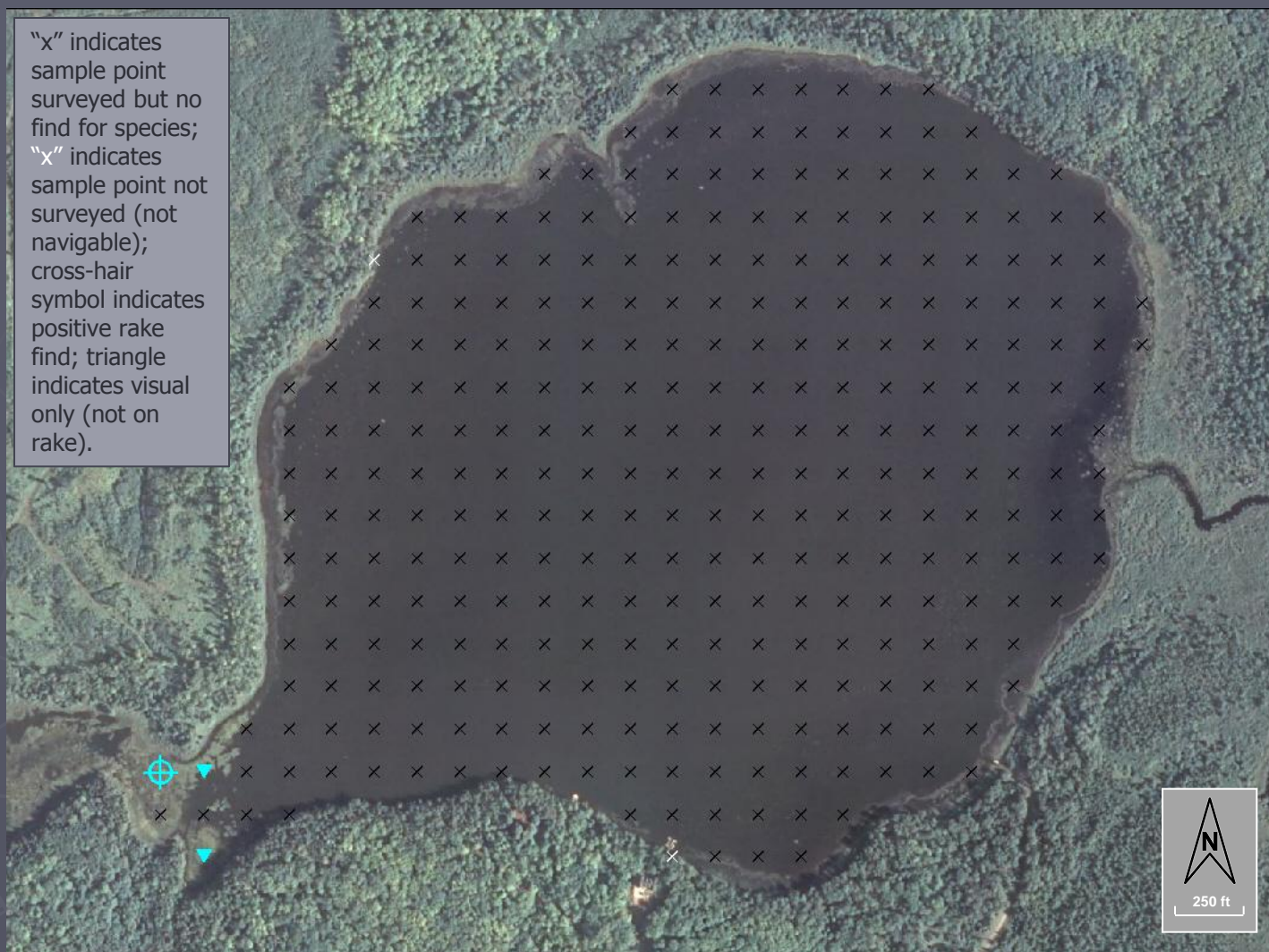
Figure 12. Distribution of plant species, Round Lake (2010)
