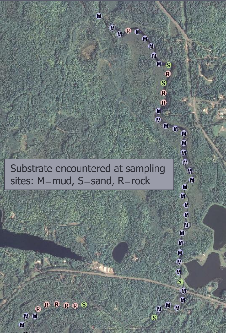
Figure 5. South Branch Presque Isle River substrate encountered at point-intercept plant sampling sites (2010).
