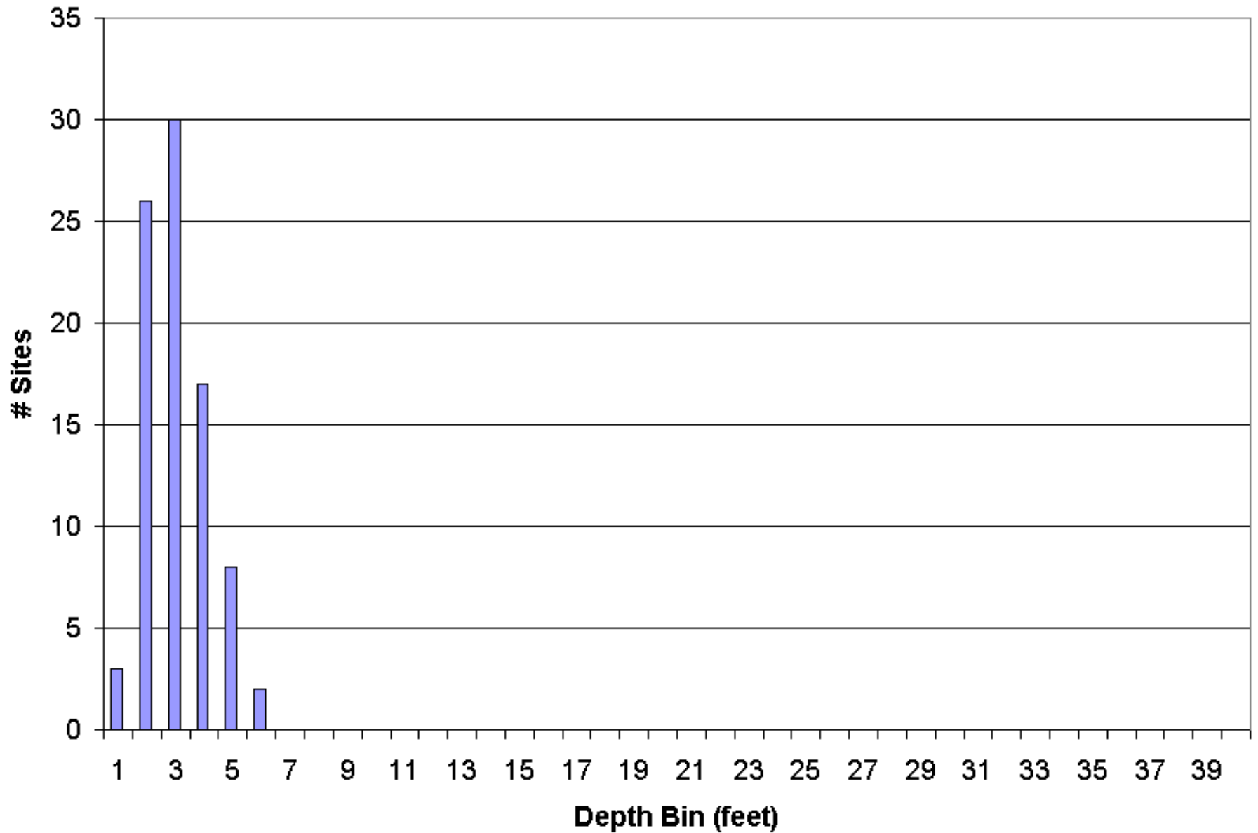
Figure 3. Maximum Depth of Plant Colonization in South Branch Presque Isle River.
