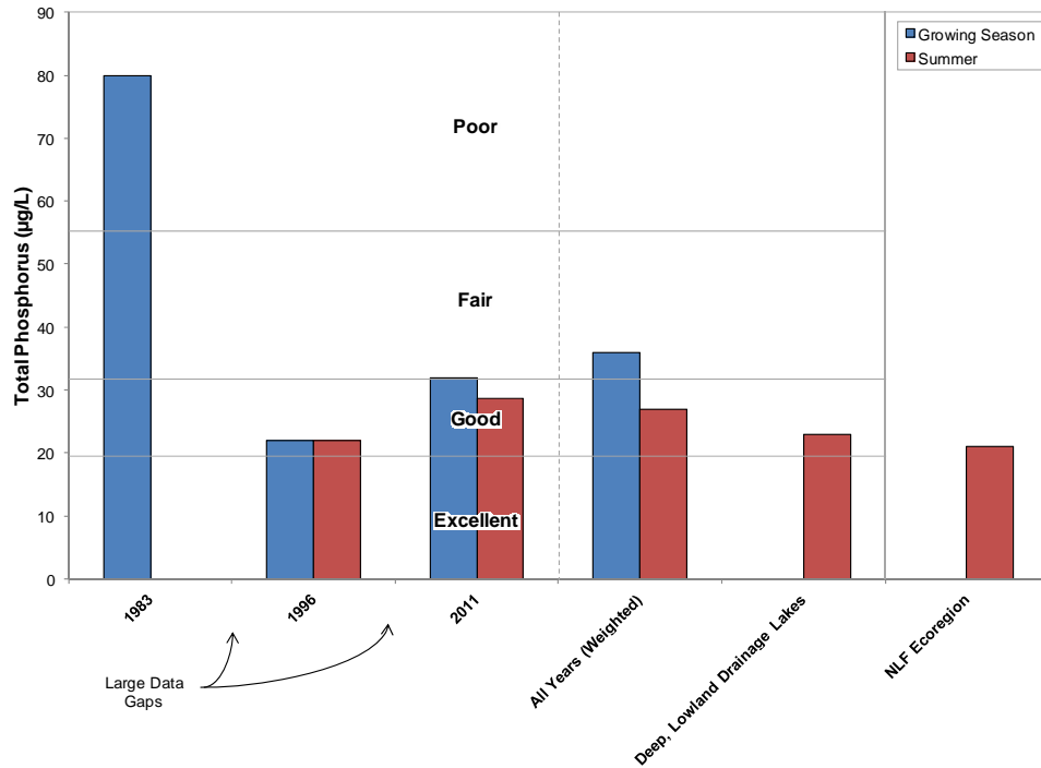
Figure 3.1-3. Big Arbor Vitae Lake, state-wide class 4 lakes, and regional total phosphorus concentrations. Mean values calculated with summer month surface sample data. Water Quality Index median values adapted from WDNR PUB WT-913.
