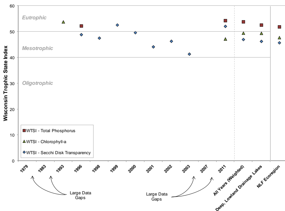
Figure 3.1-7. Big Arbor Vitae Lake, state-wide class 3 lakes, and regional Trophic State Index values. Values from summer month surface sample data using WDNR PUB-WT-193.
