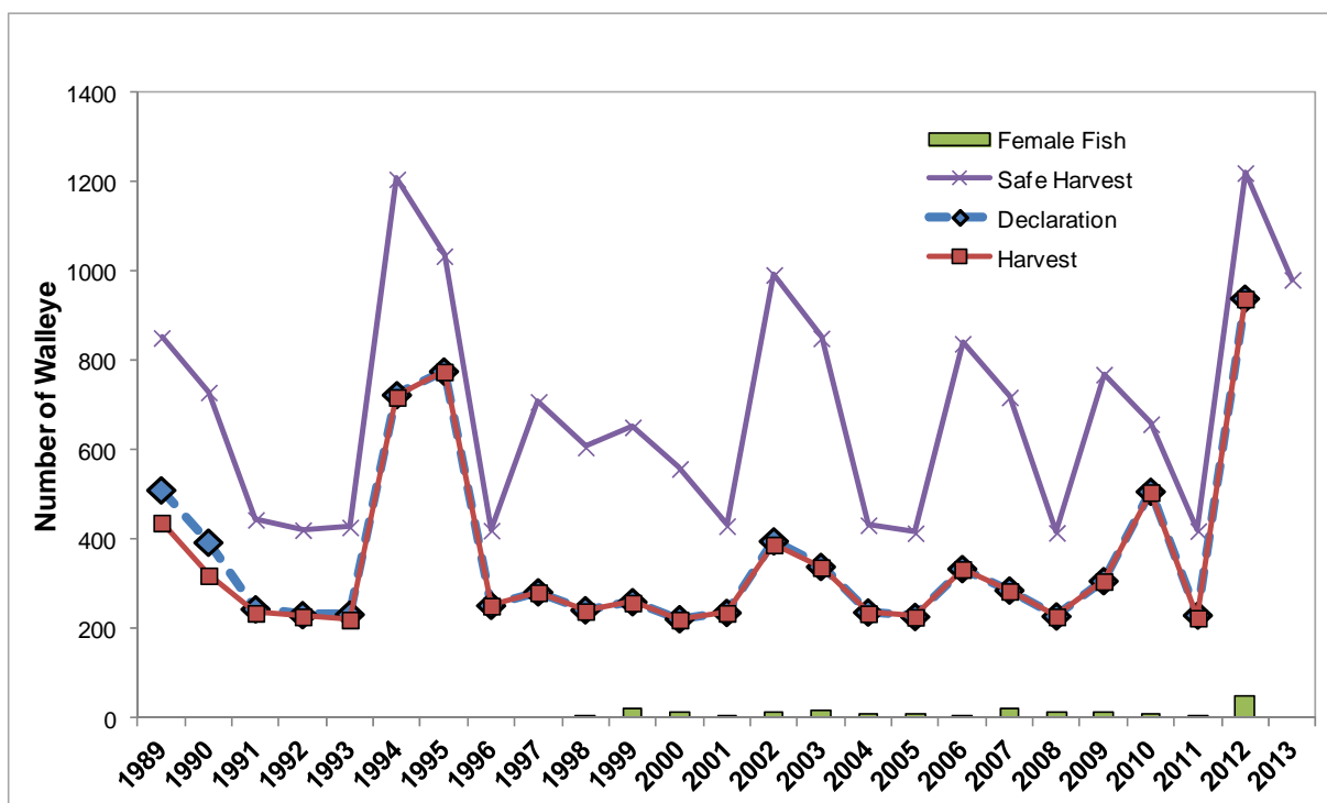
Figure 3.5-3. Open water spear harvest data of walleye for Big Arbor Vitae Lake. Annual walleye spear harvest statistics are displayed since 1989 (T. Cichosz, personal communication).
