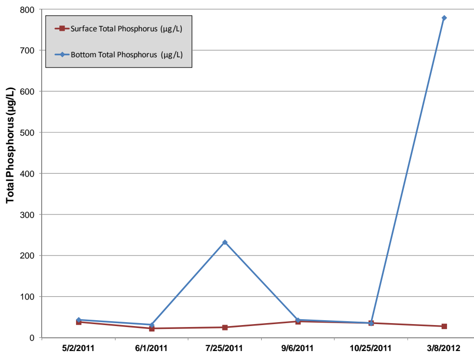
Figure 3.1-9. Big Arbor Vitae Lake phosphorus concentrations, 2011 - 2012. Includes both surface and bottom concentrations collected during water quality visits in 2011 and 2012.
