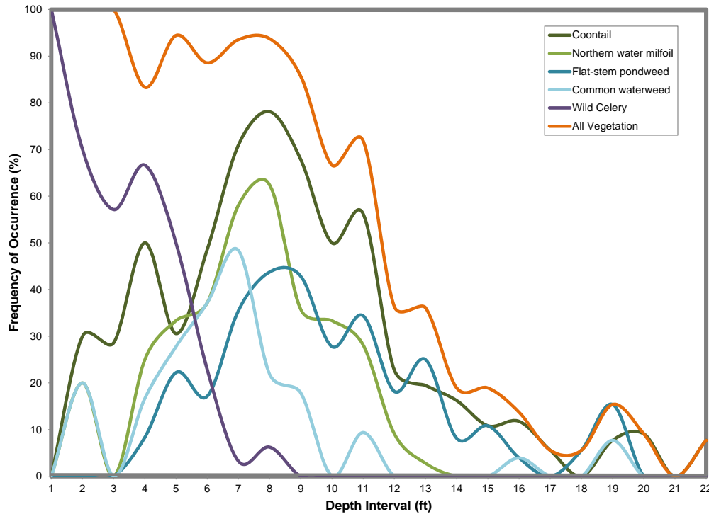
Figure 3.4-3. Frequency of occurrence of select aquatic plant species across littoral depths of Big Arbor Vitae Lake. Created using data from 2011 aquatic plant point-intercept survey. Lines are smoothed to ease visualization.
