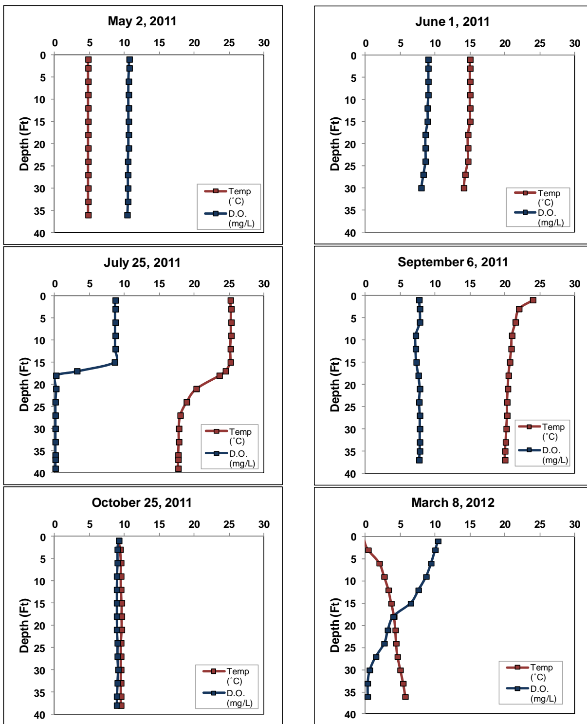
Figure 3.1-8. Big Arbor Vitae Lake dissolved oxygen and temperature profiles.
