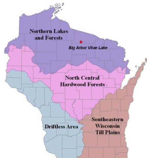
Figure 3.1-2. Location of Big Arbor Vitae Lake within the ecoregions of Wisconsin. After Nichols 1999.
