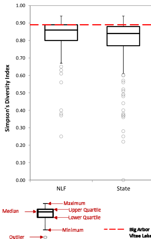
Figure 3.4-6. Big Arbor Vitae Lake species diversity index. Created using data from 2011 aquatic plant point-intercept survey.
