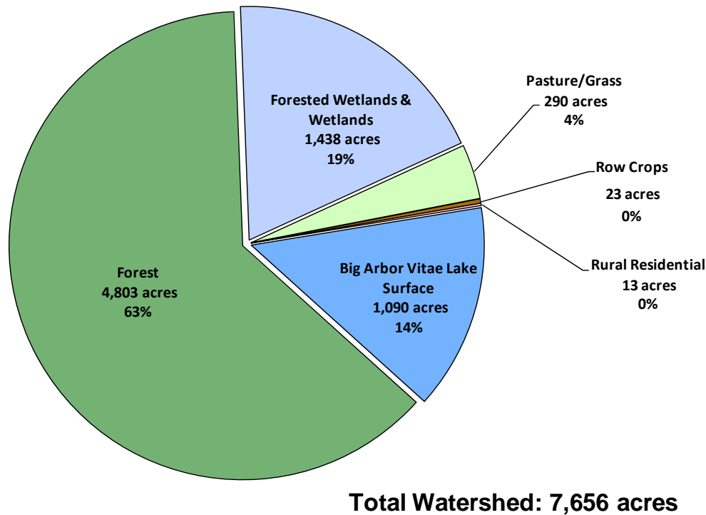
Figure 3.2-1. Big Arbor Vitae Lake watershed land cover types in acres. Based upon National Land Cover Database (NLCD – Fry et. al 2011).
