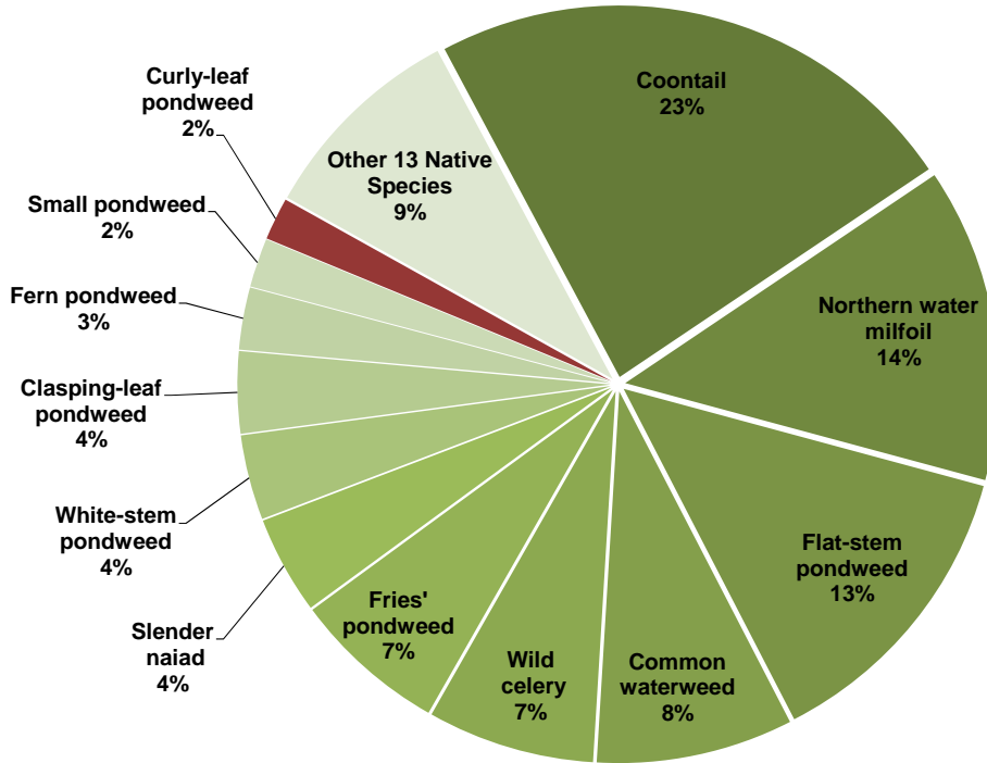
Figure 3.4-7. Big Arbor Vitae Lake aquatic plant relative occurrence analysis. Created using data from 2011 aquatic plant point-intercept survey.
