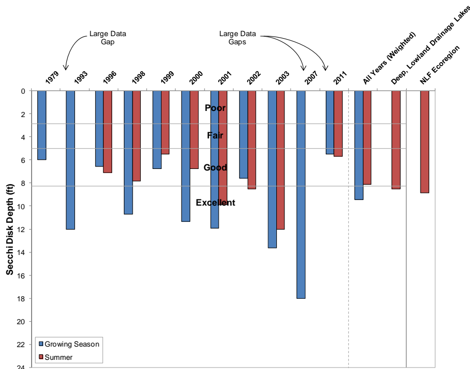
Figure 3.1-5. Big Arbor Vitae Lake, state-wide class 4 lakes, and regional Secchi disk clarity values. Mean values calculated with summer month surface sample data. Water Quality Index median values adapted from WDNR PUB WT-913.
