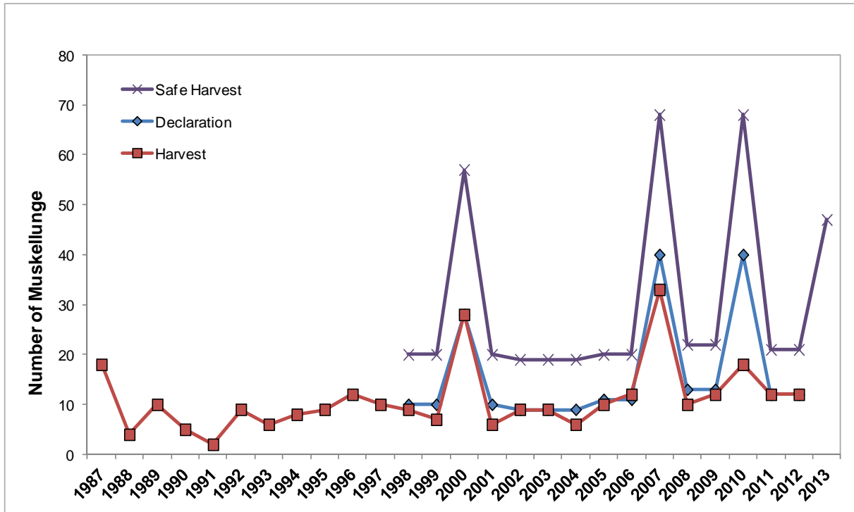
Figure 3.5-4. Big Arbor Vitae Lake muskellunge spear harvest data. Annual muskellunge spear harvest statistics are displayed since 1987 (T. Cichosz, personal communication).
