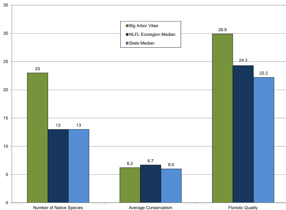
Figure 3.4-5. Big Arbor Vitae Lake Floristic Quality Assessment. Created using data from 2011 aquatic plant point-intercept survey.
