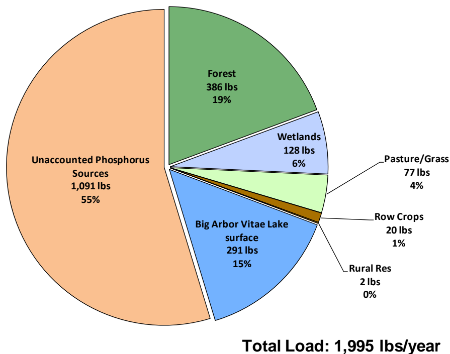
Figure 3.2-2. Big Arbor Vitae Lake watershed phosphorus loading in pounds. Based upon Wisconsin Lake Modeling Suite (WiLMS) estimates.
