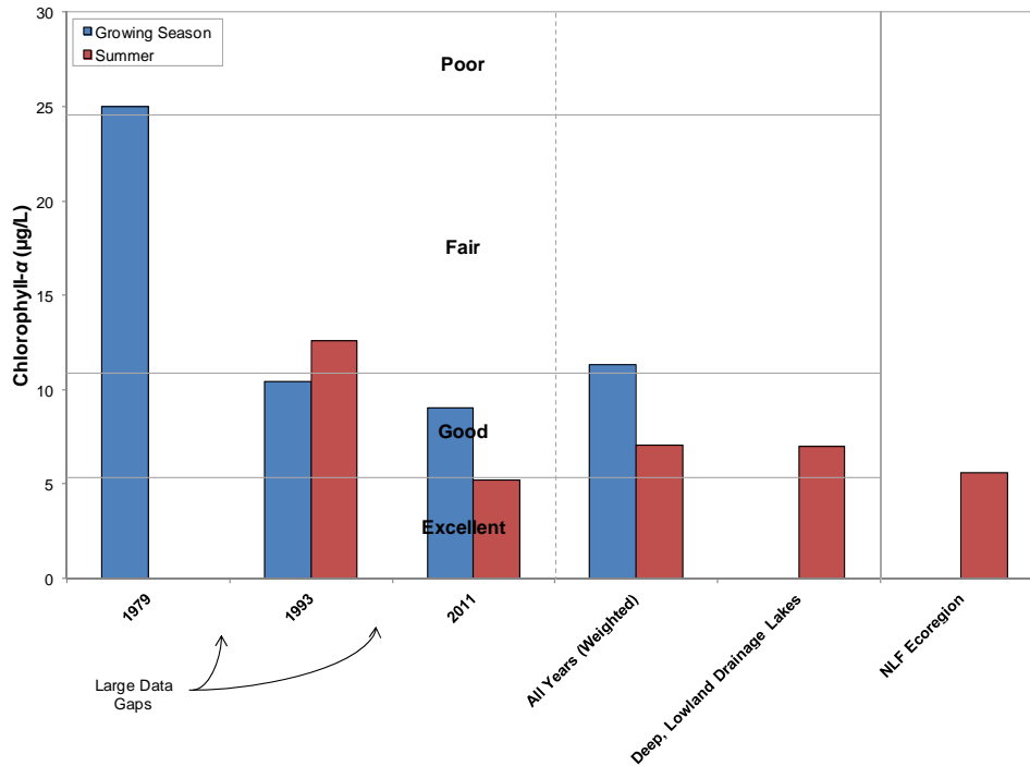
Figure 3.1-4. Big Arbor Vitae Lake, state-wide class 4 lakes, and regional chlorophyll-a concentrations. Mean values calculated with summer month surface sample data. Water Quality Index median values adapted from WDNR PUB WT-913.
