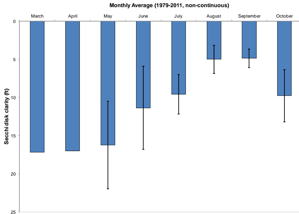
Figure 3.1-6. Big Arbor Vitae Lake monthly Secchi disk clarity averages. Includes all available data from years 1979 – 2011.
