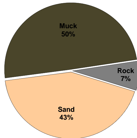
Figure 3.4-2. Big Arbor Vitae Lake proportion of substrate types within littoral areas. Created using data from 2011 aquatic plant point-intercept survey.
