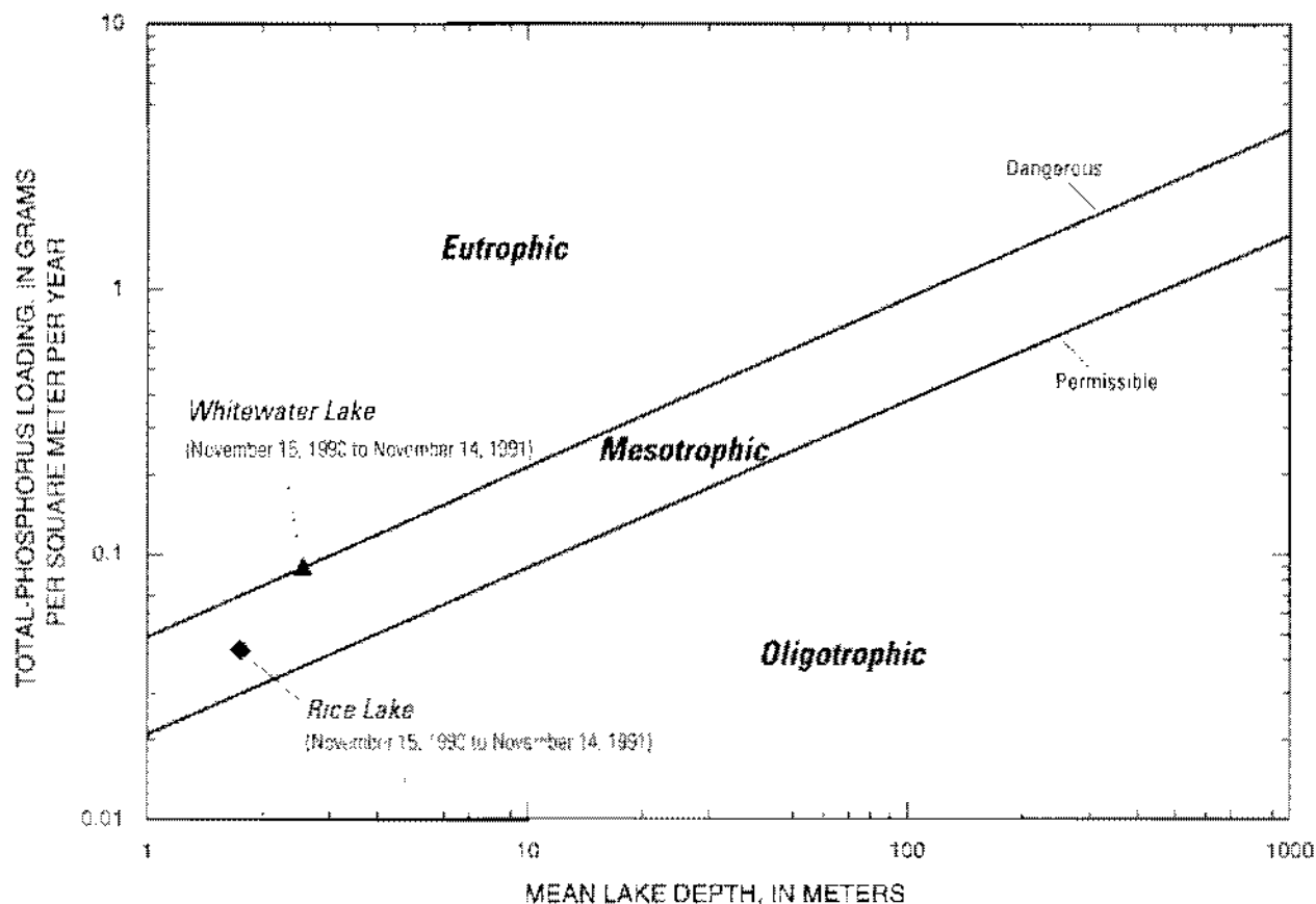
Figure 10. Vollenweider phosphorus-loading classification for Whitewater and Rice Lakes.
