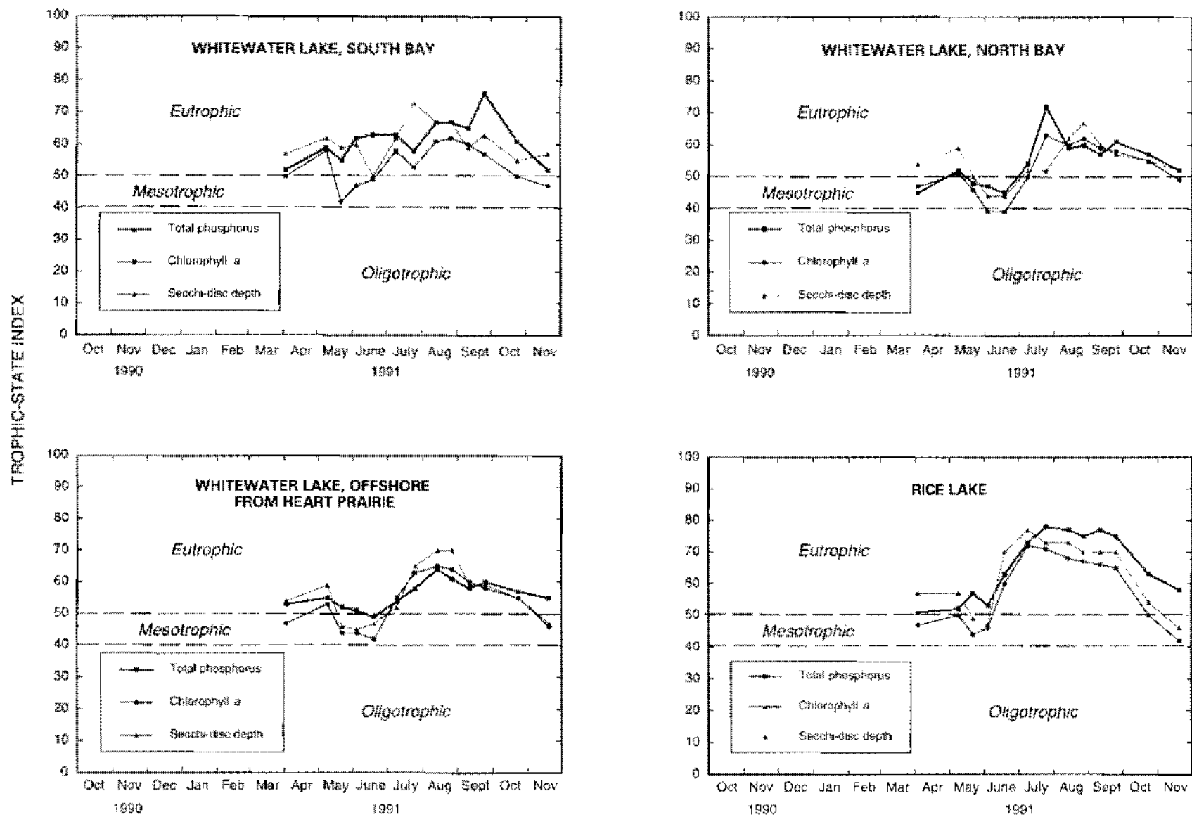
Figure 9. Trophic-State Indices for Whitewater and Rice Lakes.
