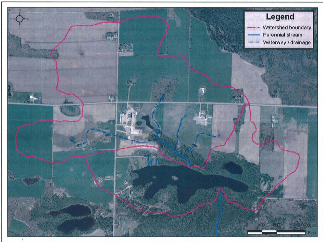
Figure 1. Bass Lake watershed and drainage patterns.
