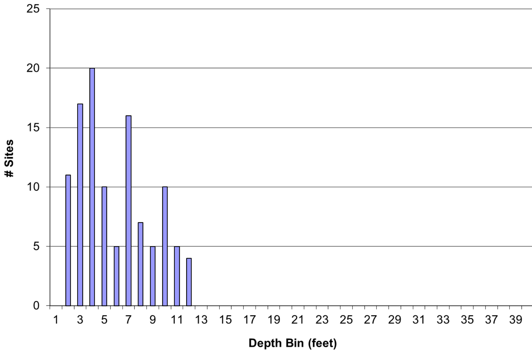
Figure 3. Maximum Depth of Plant Colonization in Oxbow Lake, 2014.
