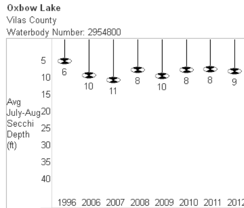
Figure 6. Oxbow Lake Secchi depth averages (July and August only).
