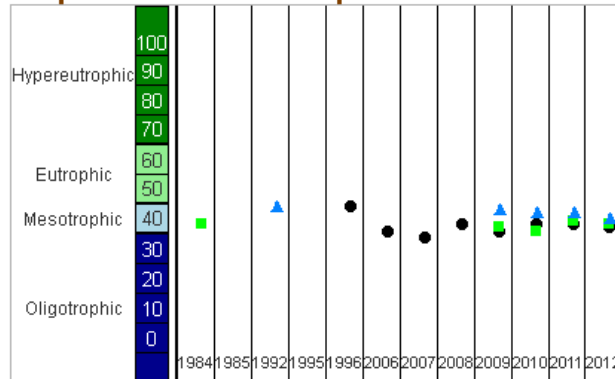
Figure 16. Oxbow Lake Trophic State Index (1984, 1992, 1996, 2006-2012).
