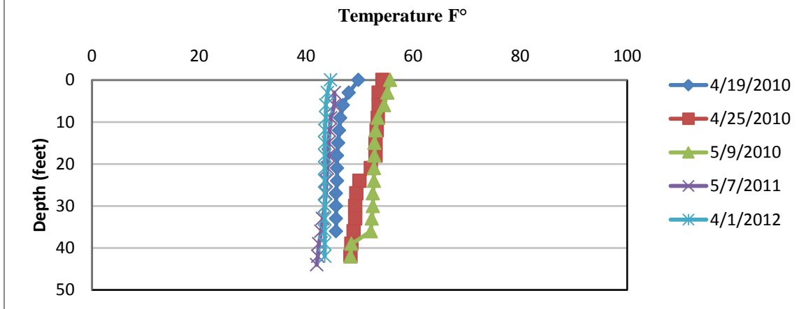
Figure 2. Oxbow Lake temperature profile, April and May (2010-2012).
