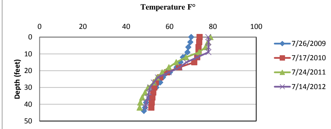
Figure 4. Oxbow Lake temperature profile, July (2009-2012).
