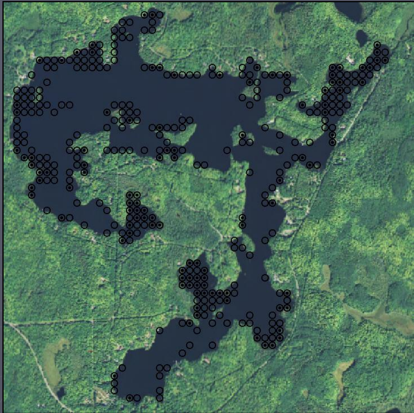
Figure 4. Oxbow Lake sampling sites less than or equal to maximum depth of rooted vegetation (2014).
