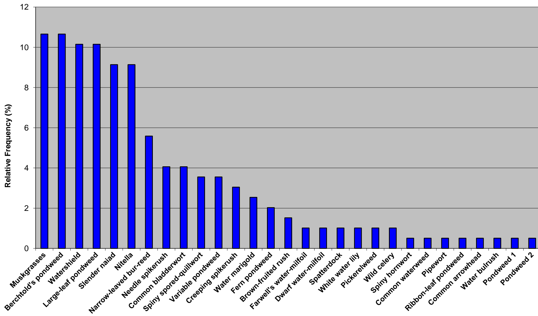
Figure 6. Oxbow Lake aquatic plant occurrences for 2014 point-intercept survey data.
