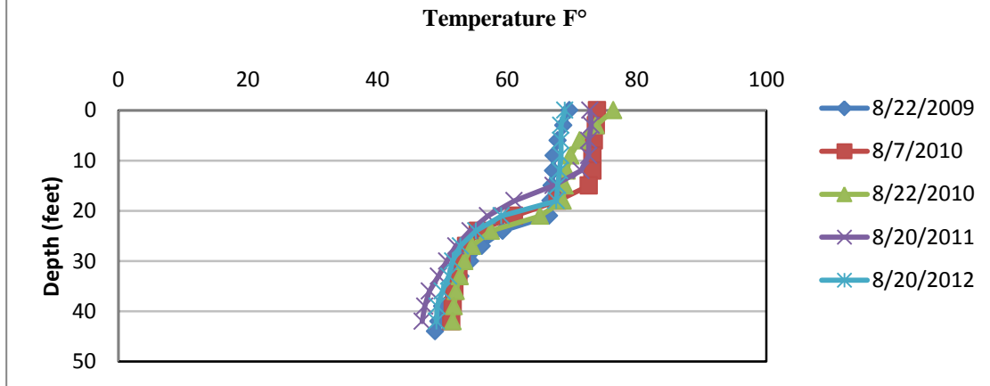
Figure 5. Oxbow Lake temperature profile, August (2009-2012).
