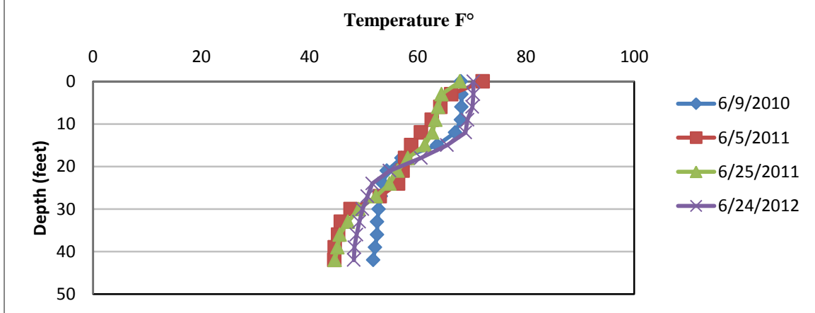
Figure 3. Oxbow Lake temperature profile, June (2010-2012).
