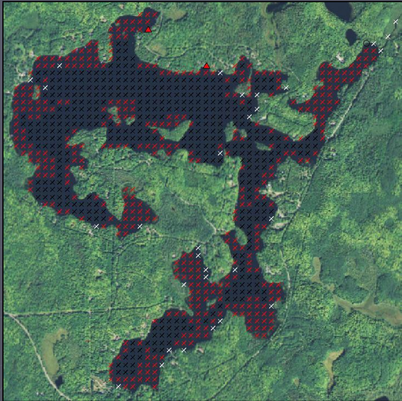
Figure 13. Distribution of plant species, Oxbow Lake (2014).
