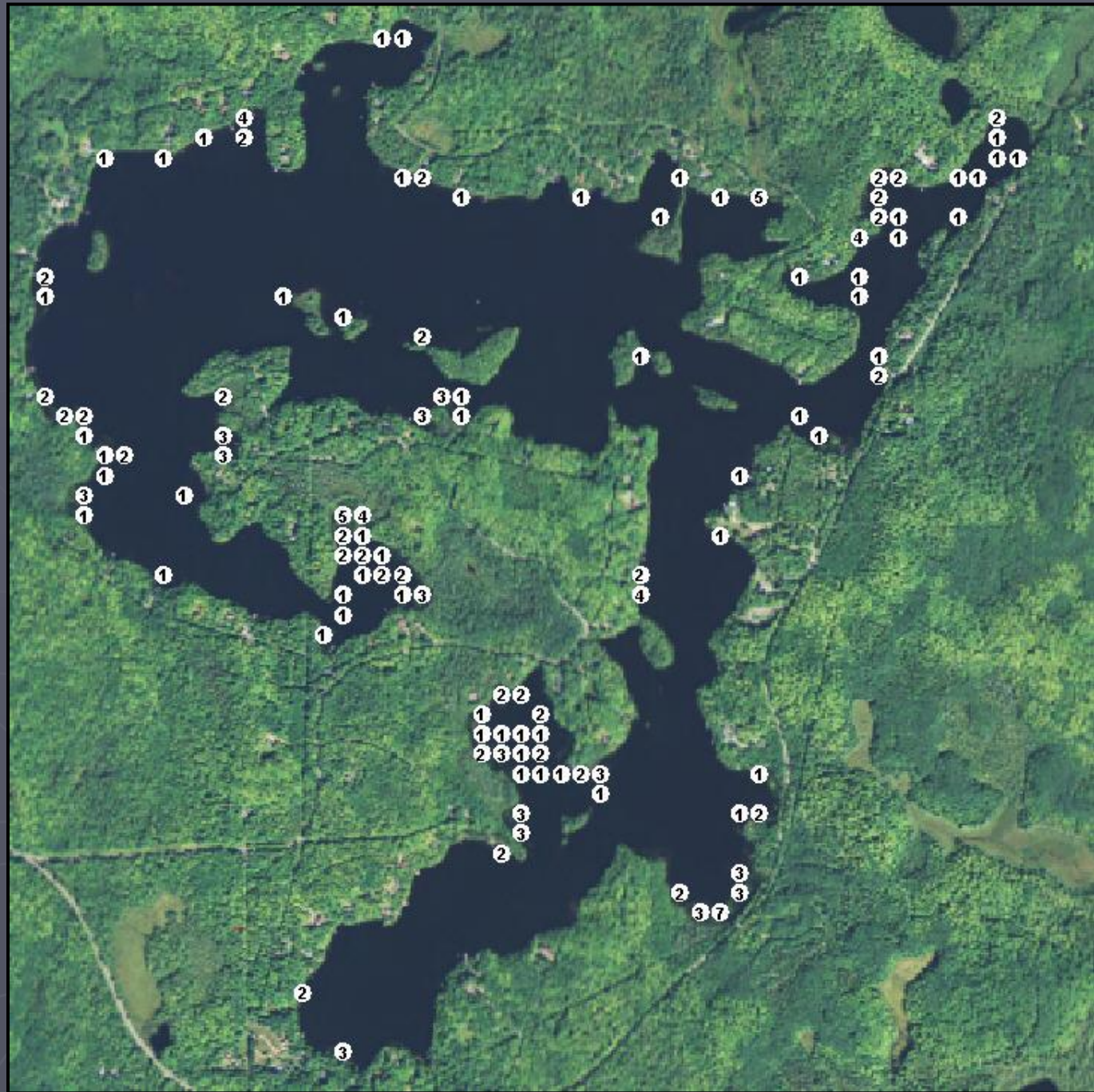
Figure 1. Number of plant species recorded at Oxbow Lake sample sites (2014).
