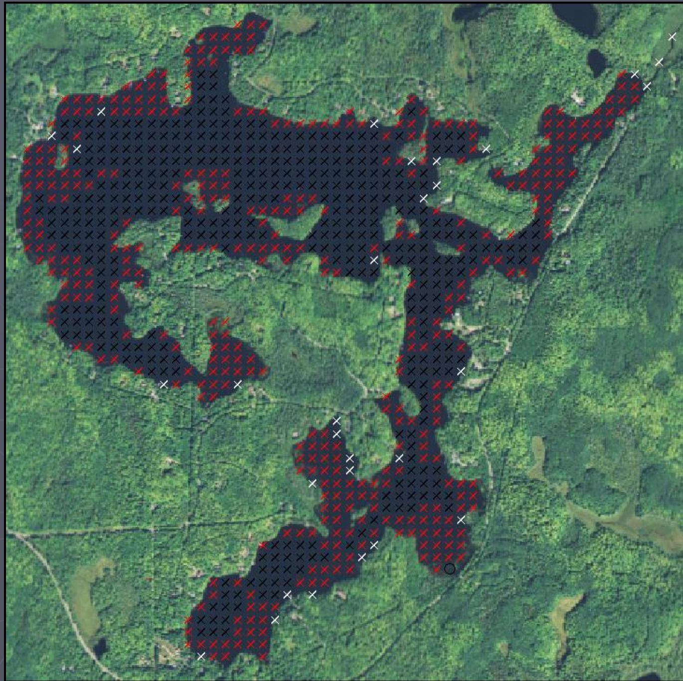
Figure 12. Distribution of plant species, Oxbow Lake (2014).
