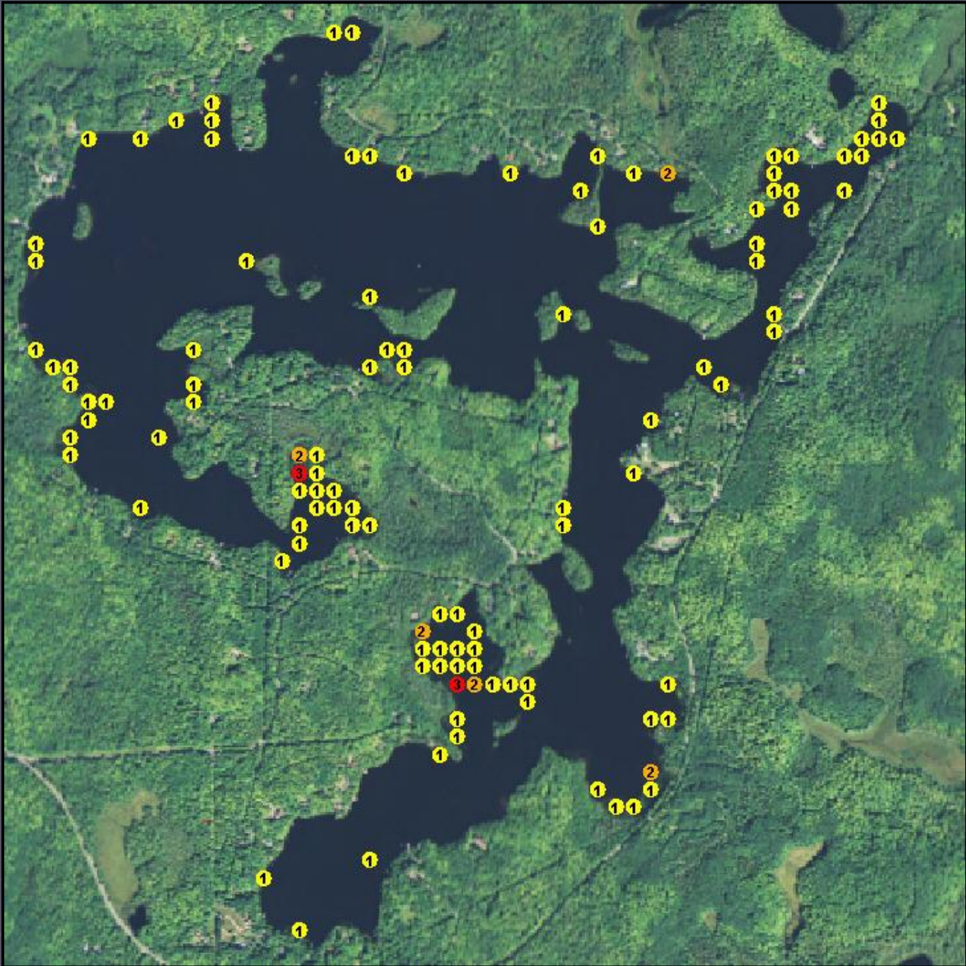
Figure 2. Rake fullness ratings for Oxbow Lake sample sites (2014).
