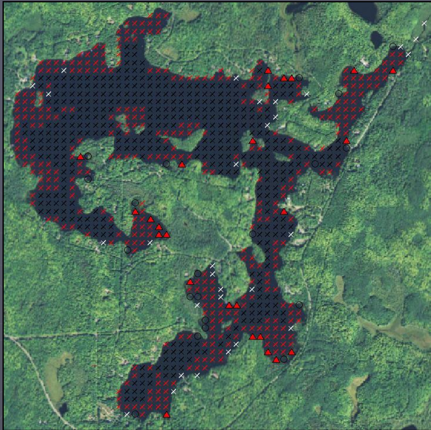
Figure 10. Distribution of plant species, Oxbow Lake (2014).
