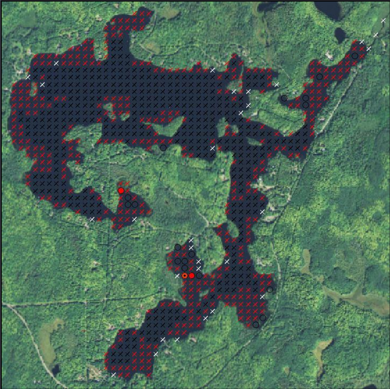
Figure 8. Distribution of plant species, Oxbow Lake (2014).
