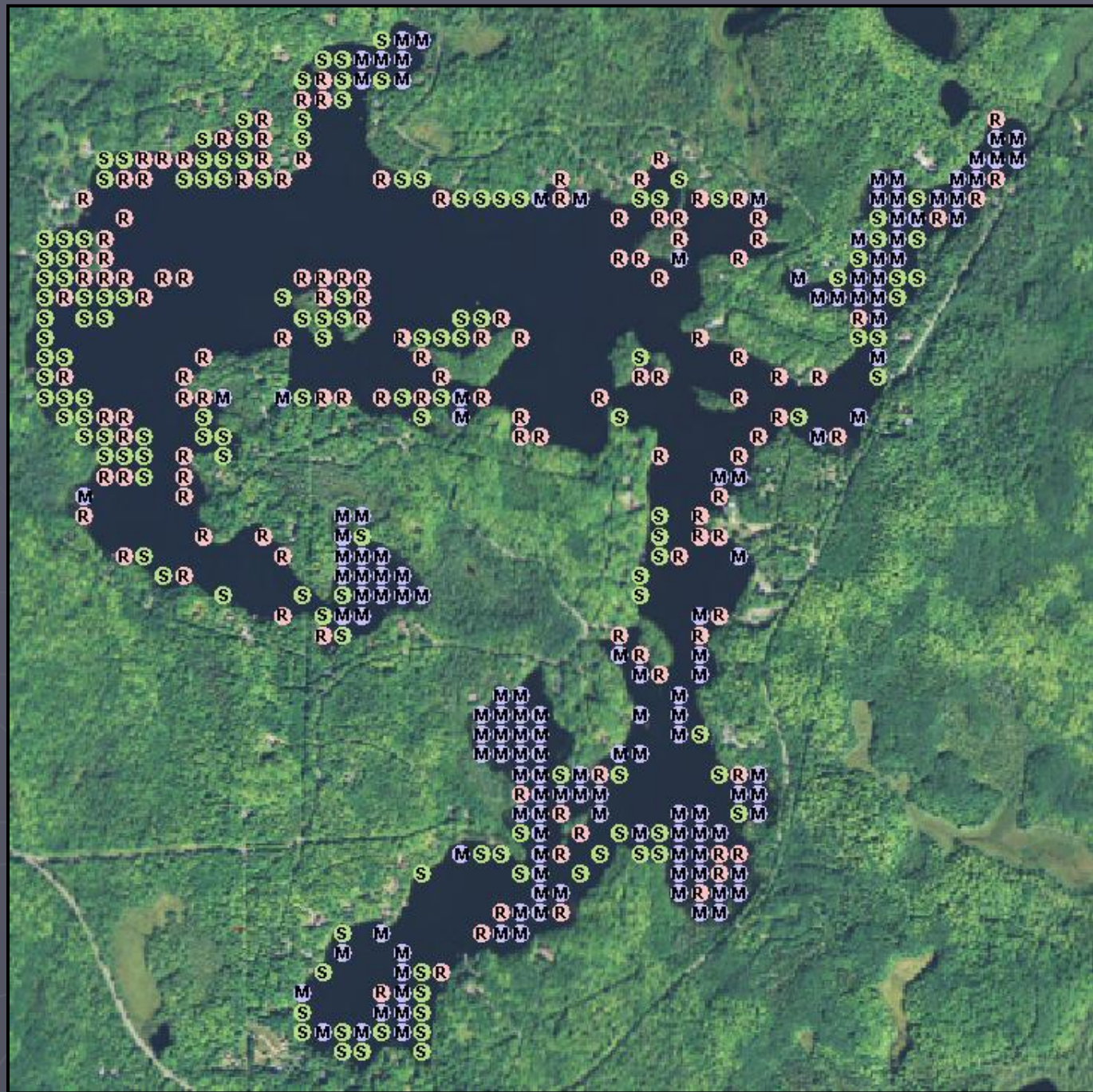
Figure 5. Oxbow Lake substrate encountered at point-intercept plant sampling sites (2014).
