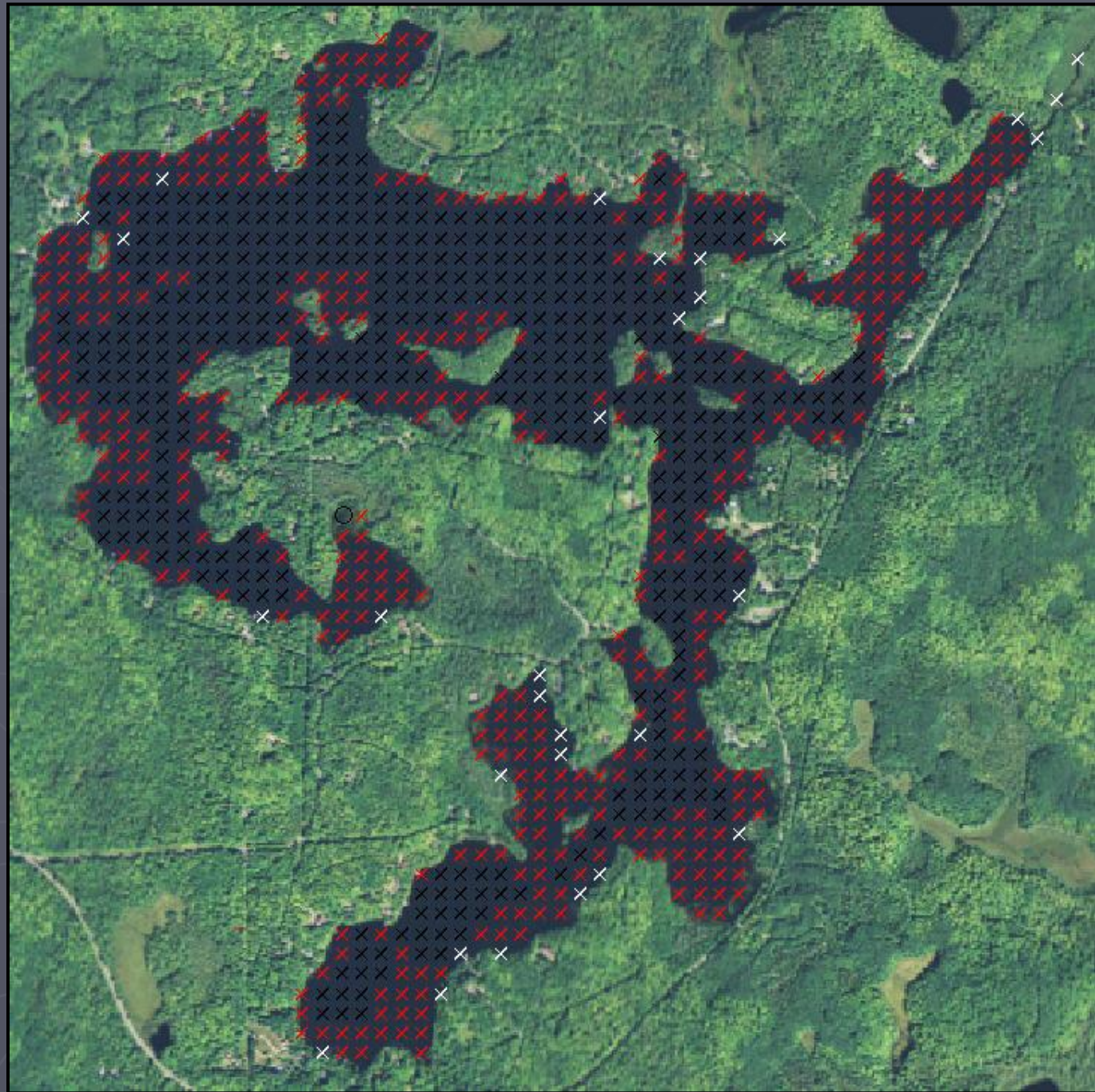
Figure 14. Distribution of plant species, Oxbow Lake (2014).
