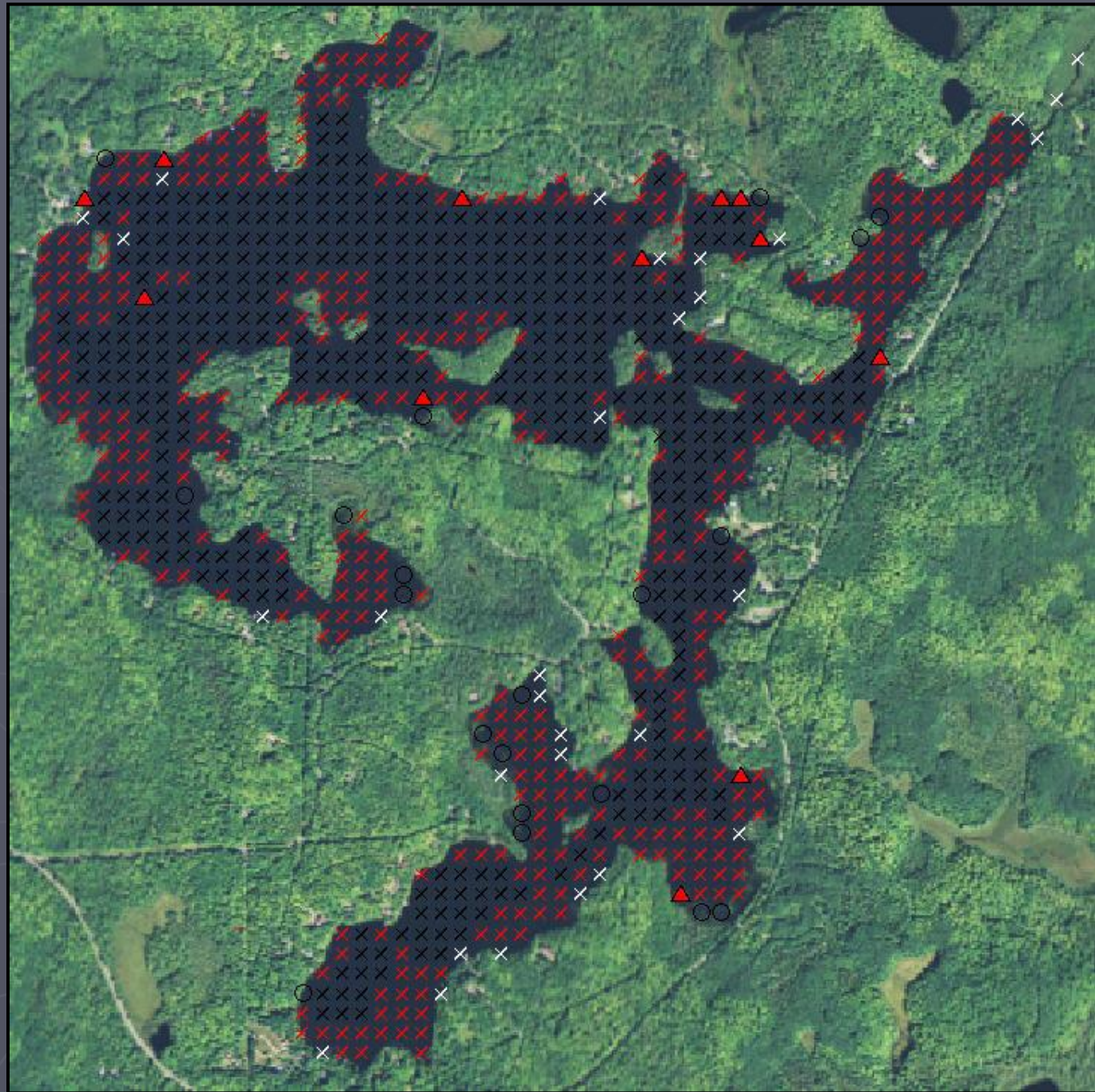
Figure 11. Distribution of plant species, Oxbow Lake (2014).
