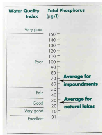
Figure 15. Total phosphorus concentrations for Wisconsin’s natural lakes and impoundments (Shaw et al., 2004).
