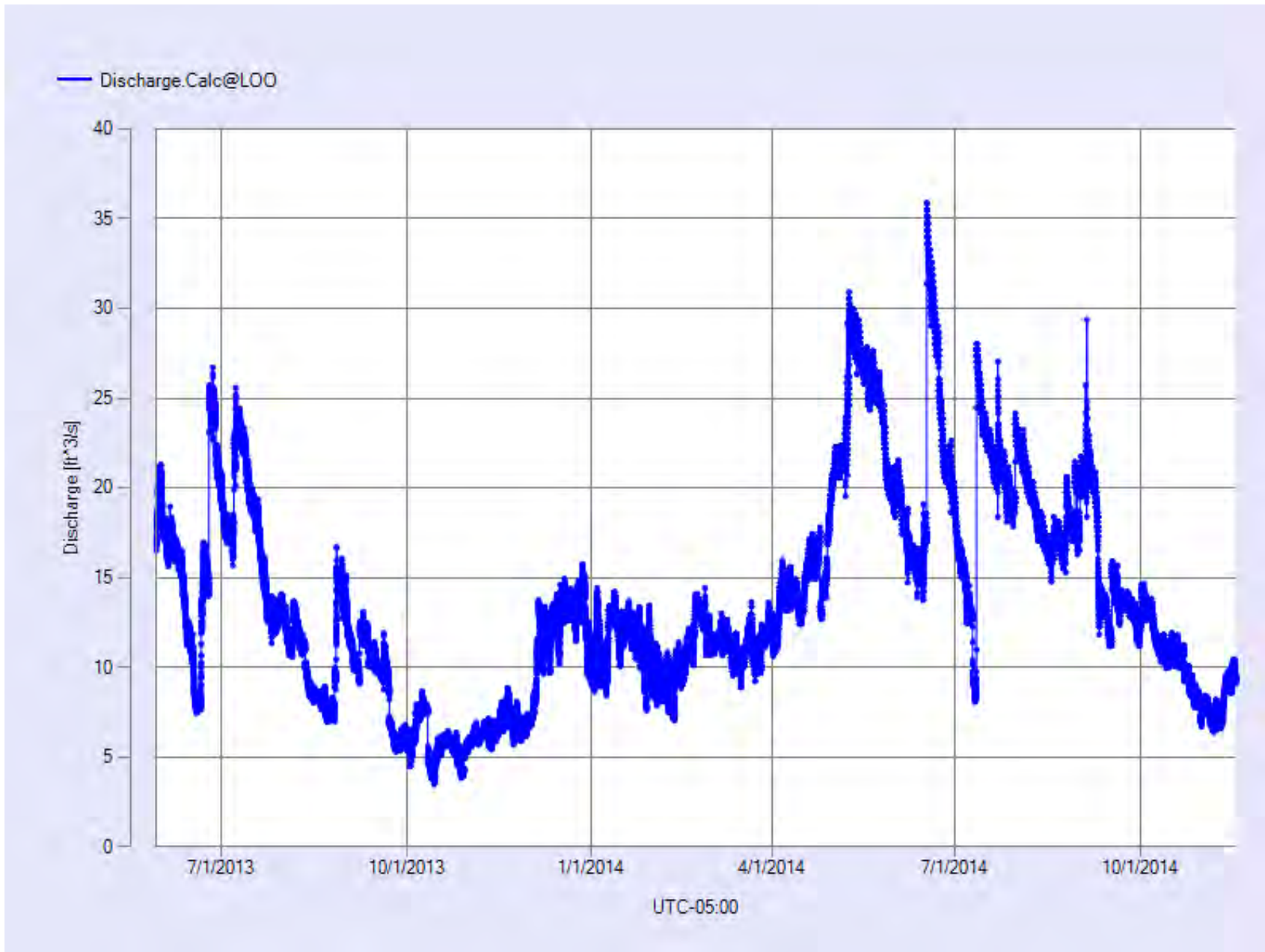
Figure 11.1 Discharge record from Lake Owen, 2013 to 2014.
