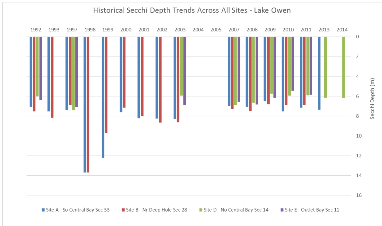
Figure 5.21. Historical trends in Secchi depth across all sites in Lake Owen.
