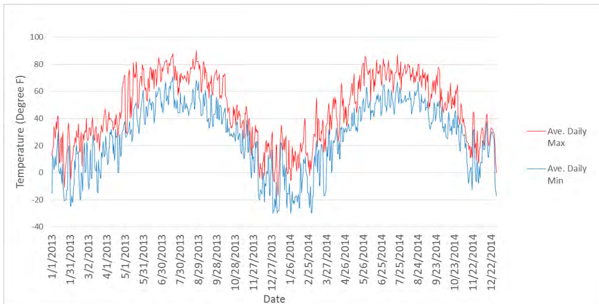
Figure 5.1. Minimum and maximum daily air temperatures through study period.
