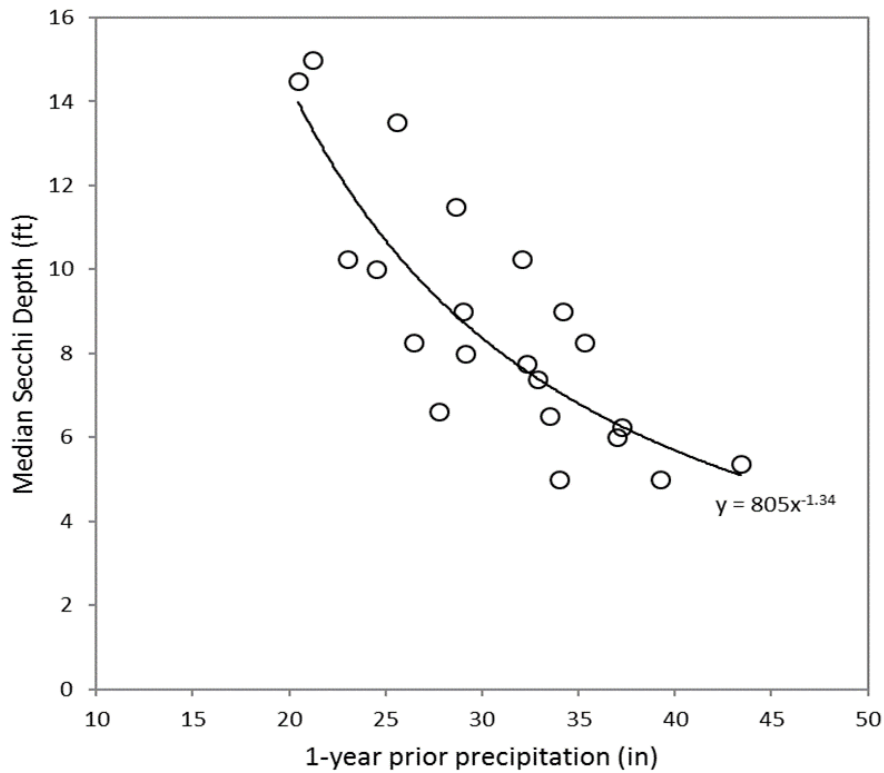
Figure 14. Secchi Disk Relation to Precipitation Dead Pike Lake Secchi disk measurements from the deep hole compared to the previous 365 days of total precipitation
