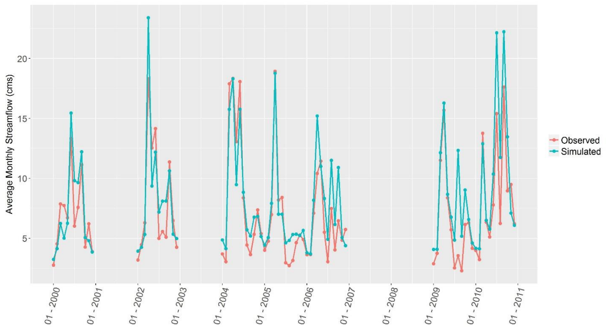
Figure D- 6. Monthly streamflow calibration hydrograph for USGS site 04078500 (Embarrass River near Embarrass, WI).
