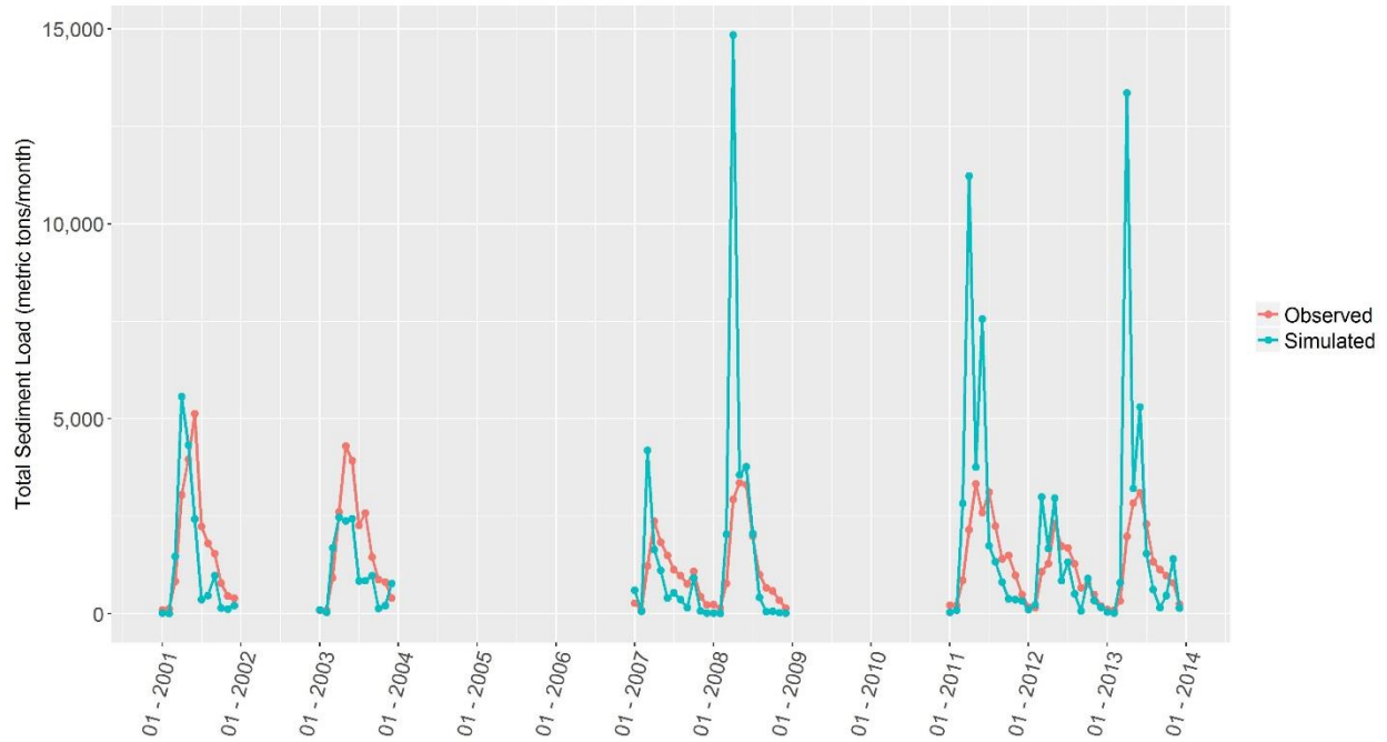
Figure E- 1. Monthly sediment calibration plot for USGS site 04079000 (Wolf River at New London, WI).
