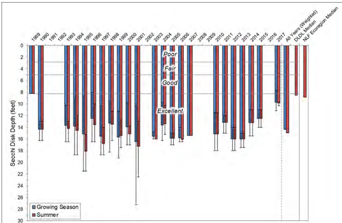
Figure 8.1.1-3. Plum Lake, statewide deep lowland drainage lakes, and regional Secchi disk clarity values. Mean values calculated with summer month surface sample data. Water Quality Index values adapted from WDNR PUB WT-913.
