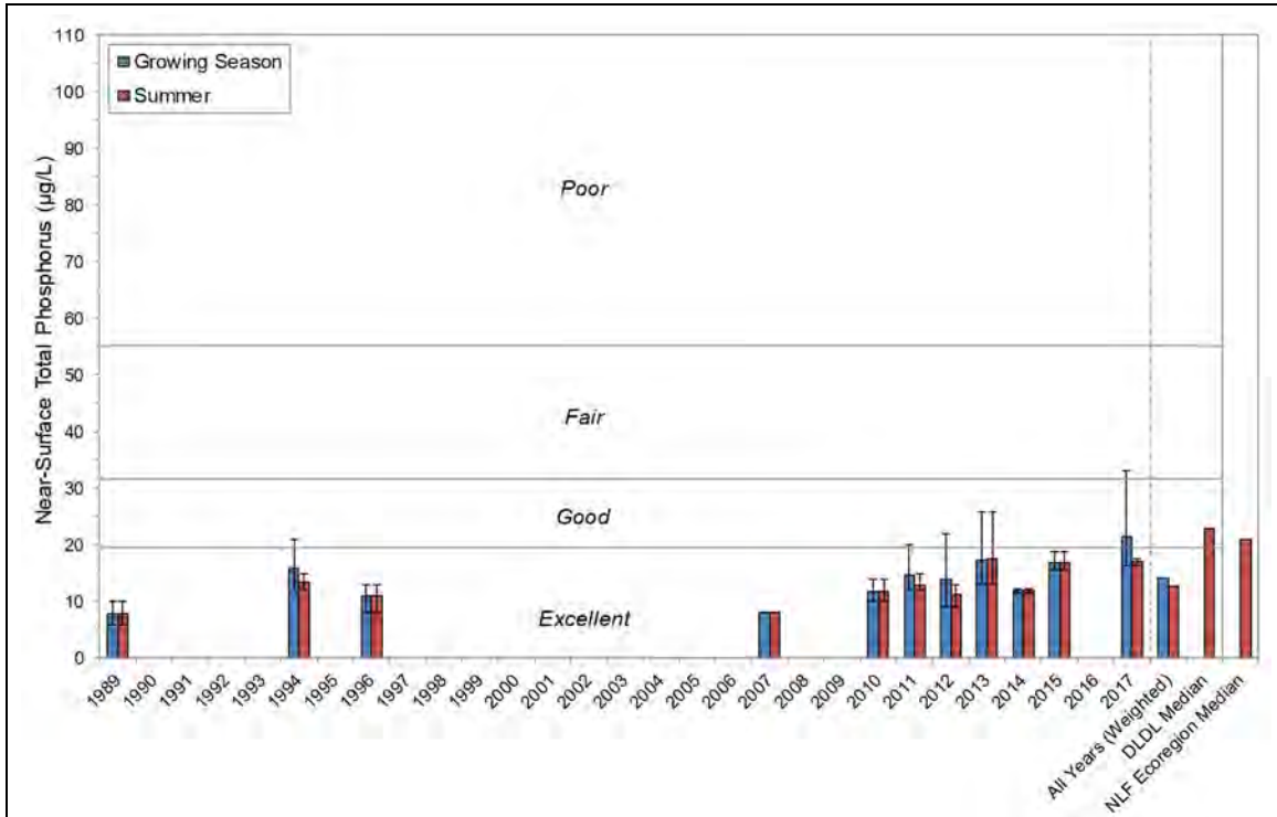
Figure 8.1.1-1. Plum Lake, statewide deep lowland drainage lakes, and regional total phosphorus concentrations. Mean values calculated with summer month surface sample data. Water Quality Index values adapted from WDNR PUB WT-913.
