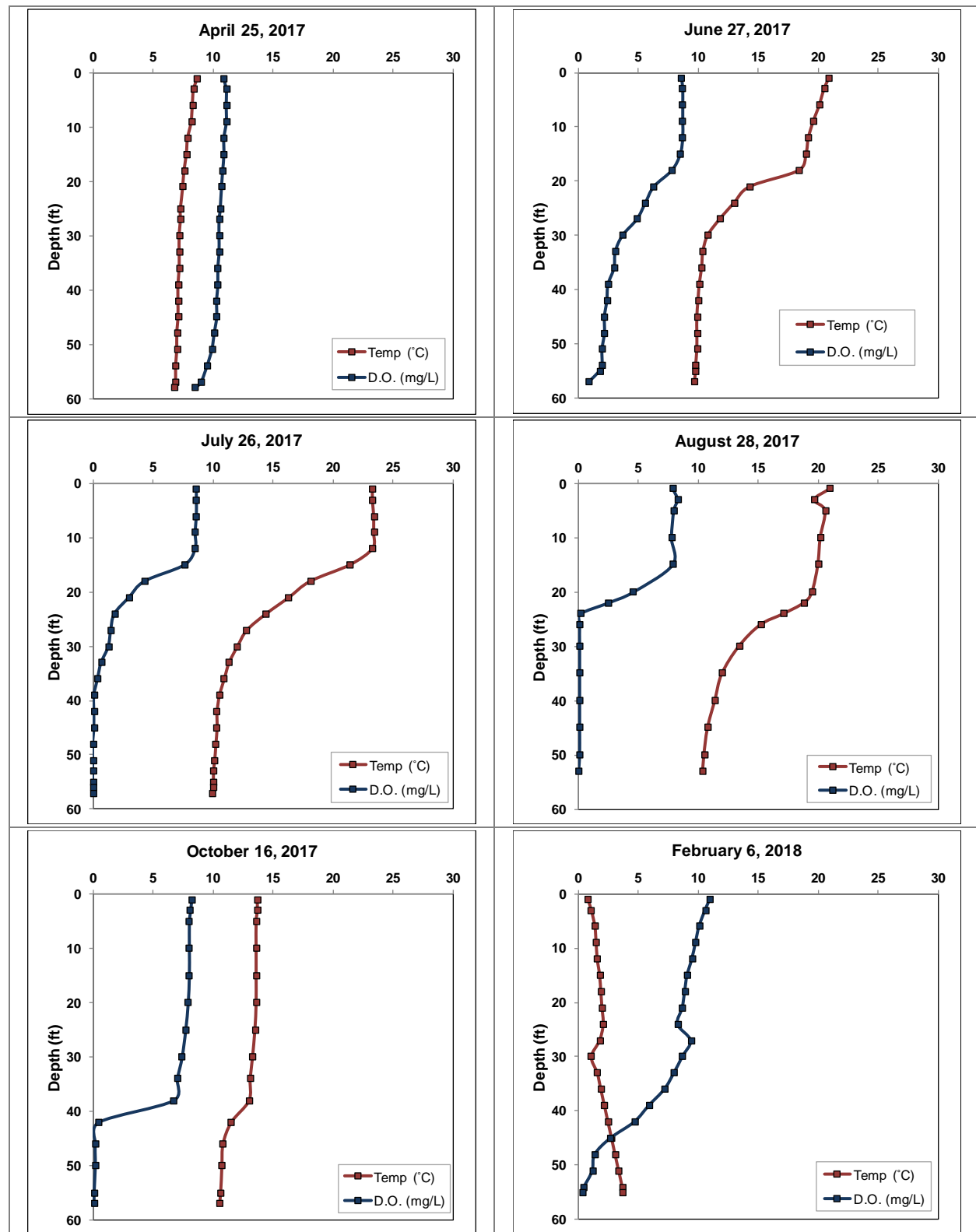
Figure 8.1.1-5. Plum Lake 2017/2018 dissolved oxygen and temperature profiles.
