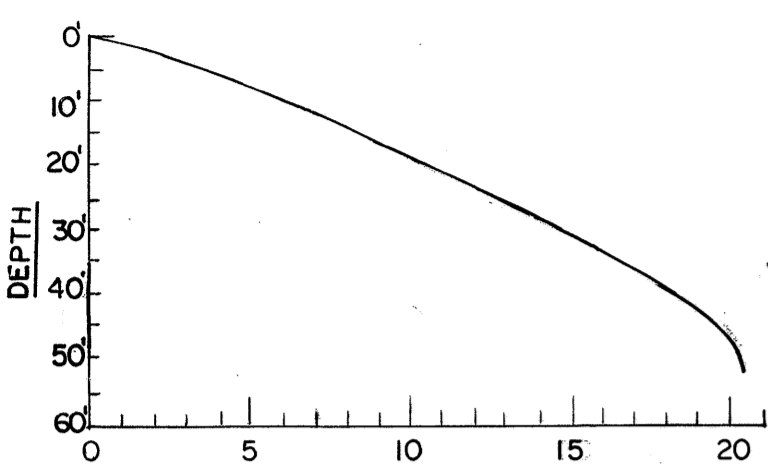
VOLUME ACRE FEET IN HUNDREDS
