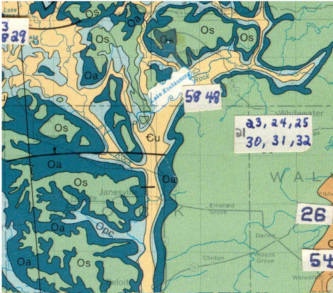
Figure 3: Bedrock geology of Lake Koshkonong area (figure from WGNHS 1982)
