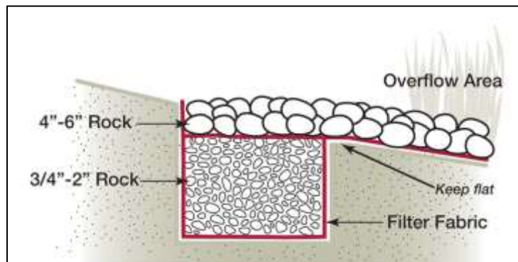
Figure 13: Rock Infiltration Set-up
