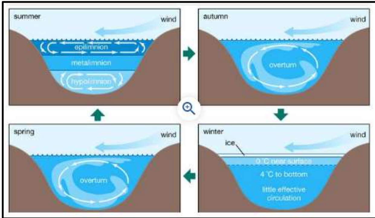
Figure 6. Seasonal thermal stratification in lakes (Encyclopedia Britannica)
