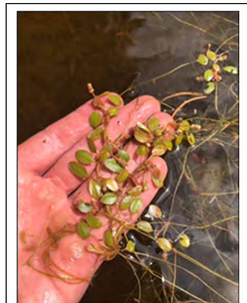
Photograph 8.4.4-1. Vasey’s pondweed ( Potamogeton vaseyi ), with floating leaves and flowering present. P. vaseyi is an uncommon native aquatic plant listed as special concern found in Fawn Lake. Photo credit: Onterra.
