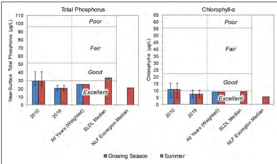
Figure 8.4.1-1. Fawn Lake average annual near-surface total phosphorus and chlorophyll- a concentrations and median near-surface total phosphorus and chlorophyll- a concentrations for state-wide shallow lowland drainage lakes (SLDL) and Northern Lakes and Forests (NLF) ecoregion lakes. Water Quality Index values adapted from WDNR PUB WT-913. Error bars represent maximum and minimum values.
