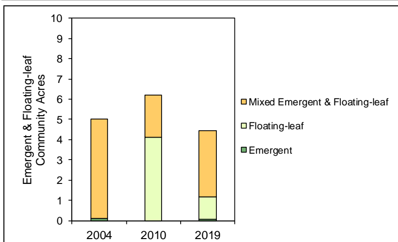
Figure 8.4.4-8. Fawn Lake emergent and floating-leaf community acres from 2004, 2010, and 2019. Change in acreage likely due to fluctuations in water levels over this period.
