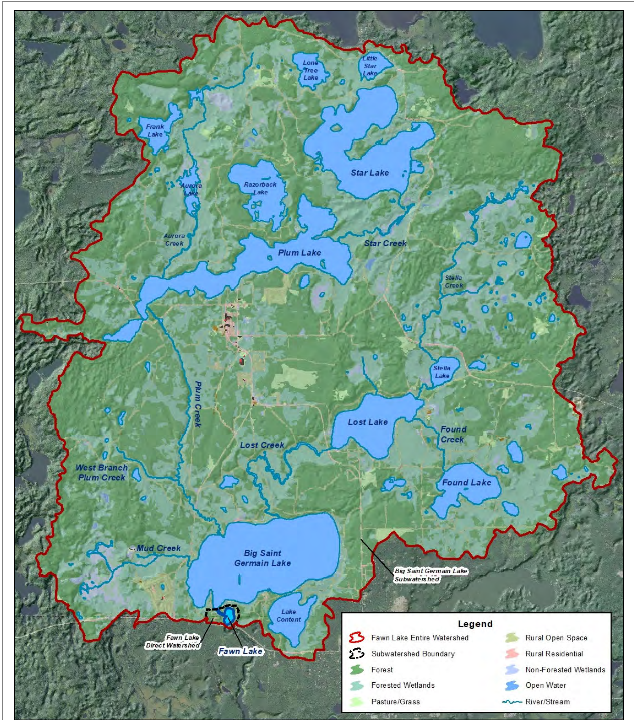
Figure 8.4.2-1. Fawn Lake watershed and land cover types.
