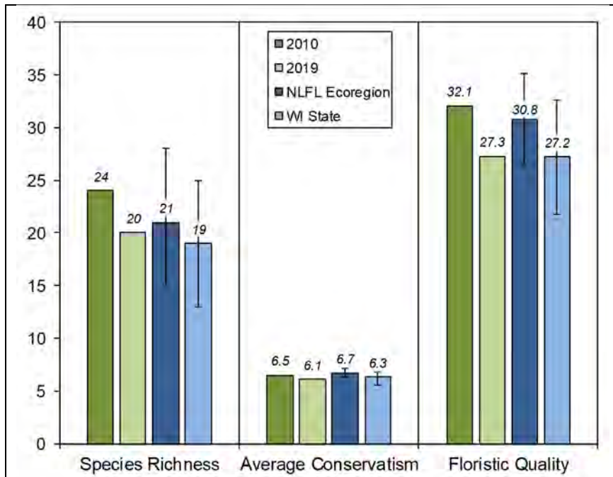
Figure 8.4.4-7. Fawn Lake Floristic Quality Assessment. Error bars represent interquartile range. Created using data from Onterra 2010 and 2019 point-intercept surveys. Regional and state medians calculated with Onterra and WDNR data. Analysis follows Nichols 1999.
