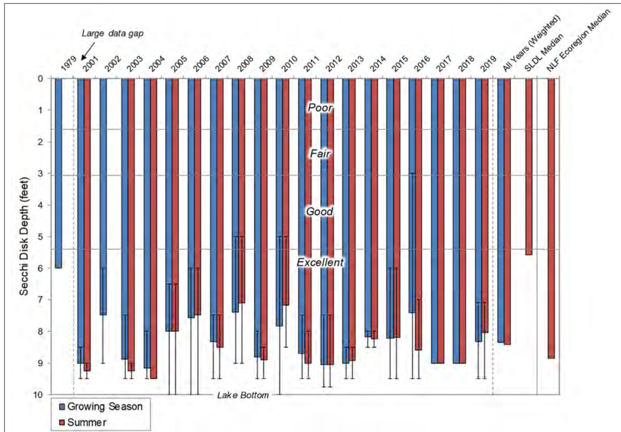
Figure 8.4.1-2. Fawn Lake average Secchi disk depth and median Secchi disk depths for state-wide shallow lowland drainage lakes (SLDL) and Northern Lakes and Forests (NLF) ecoregion lakes. Water Quality Index values adapted from WDNR PUB WT-913. Error bars represent maximum and minimum values.
