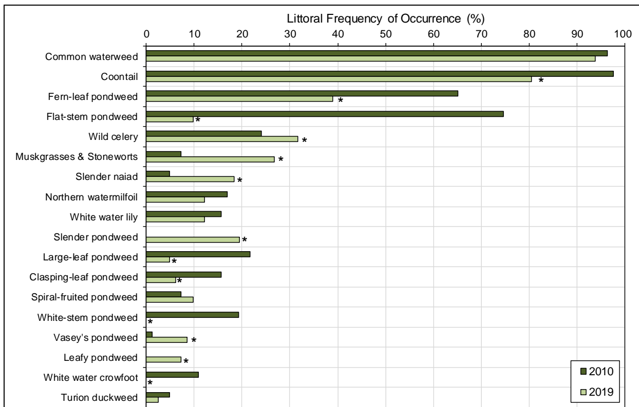
Figure 8.4.4-3. Littoral frequency of occurrence of select aquatic plant species in Fawn Lake from 2010 and 2019 point-intercept surveys. Species with a littoral frequency of occurrence of at least 5% in one of the two surveys are displayed. * = Statistically valid change in occurrence from 2010. Created using data from Onterra 2010 and 2019 point-intercept surveys.
