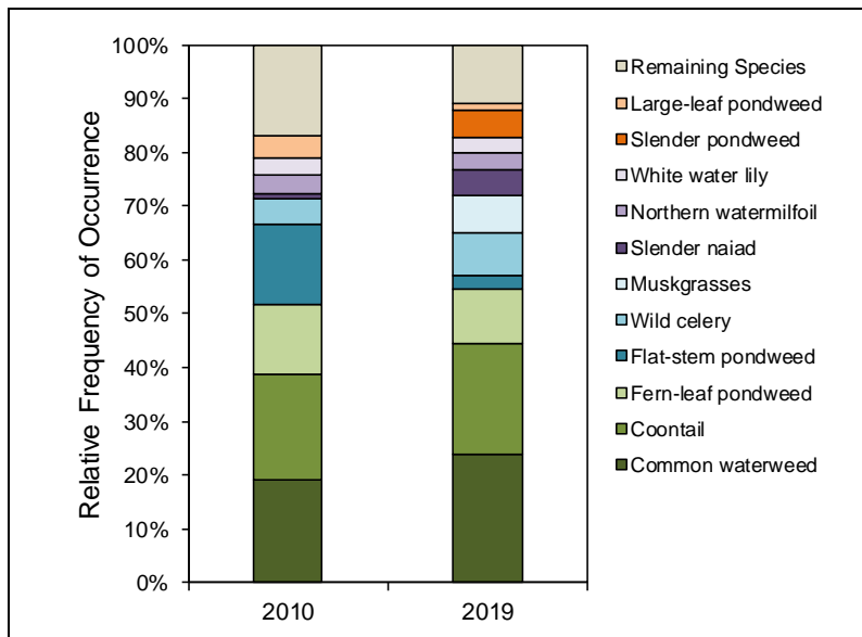
Figure 8.4.4-5. Fawn Lake aquatic plant relative frequency of occurrence. Created using data from Onterra 2010 and 2019 point-intercept surveys.
