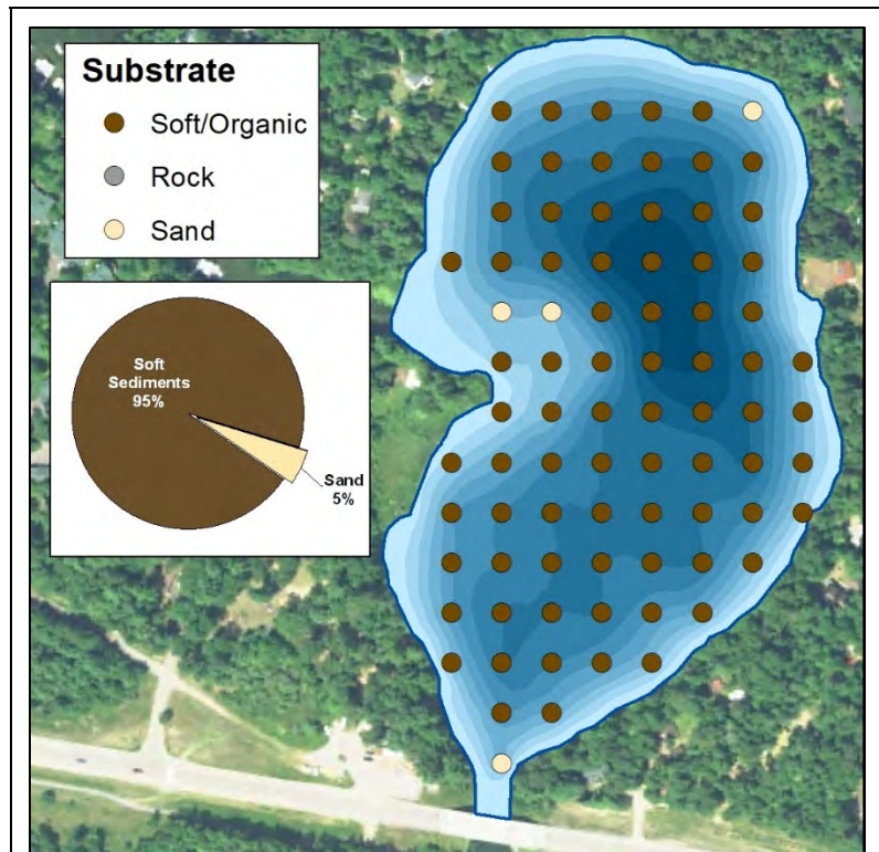
Figure 8.4.4-1. Fawn Lake substrate types as determined from the 2019 point-intercept survey. Please note substrate types can only be determined at sampling locations in 15 feet of water or less.
