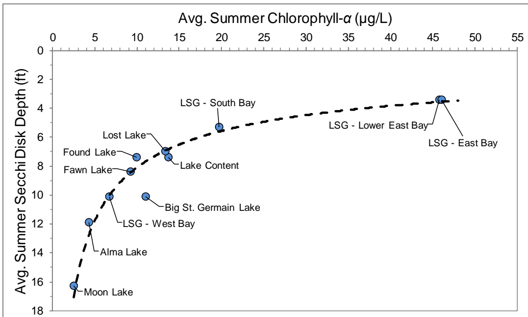
Figure 3.1-9. Town of Saint Germain project lakes average summer Secchi disk depths plotted against average summer chlorophyll-α concentrations. Chlorophyll is a good predictor of Secchi disk depth in the project lakes.
