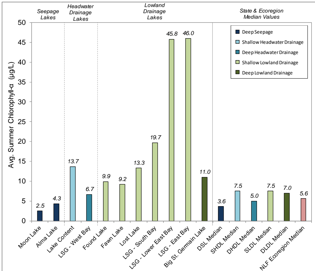
Figure 3.1-6. Town of Saint Germain project lakes summer average chlorophyll- a concentrations and median summer chlorophyll- a concentrations for comparable lakes. Individual lake values calculated using all available historical and current data. DSL = deep seepage lake; SHDL = shallow headwater drainage lake; DHDL = deep headwater drainage lake; SLDL = shallow lowland drainage lake; DLDL = deep lowland drainage lake; NFL = Northern Lakes and Forests Lakes ecoregion.
