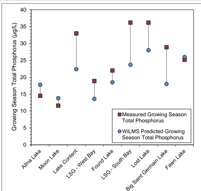
Figure 3.2-6. Town of St. Germain lakes measured versus WiLMS-predicted in-lake growing season total phosphorus concentrations. Internal phosphorus loading from bottom sediments is the primary reason why measured concentrations in some lakes are higher than predicted. Phosphorus loading from internal loading is not accounted for in WiLMS modeling.
