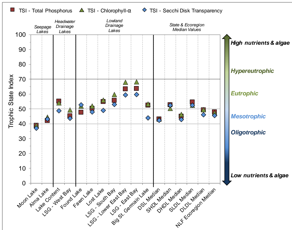
Figure 3.1-11. Town of Saint Germain project lakes Trophic State Index. Values calculated with summer month surface sample data using WDNR PUB-WT-193. DSL = deep seepage lake; SHDL = shallow headwater drainage lake; DHDL = deep headwater drainage lake; SLDL = shallow lowland drainage lake; DLDL = deep lowland drainage lake; NFL = Northern Lakes and Forests Lakes ecoregion.
