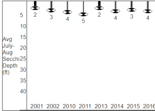
Past secchi averages in feet (July and August only).
