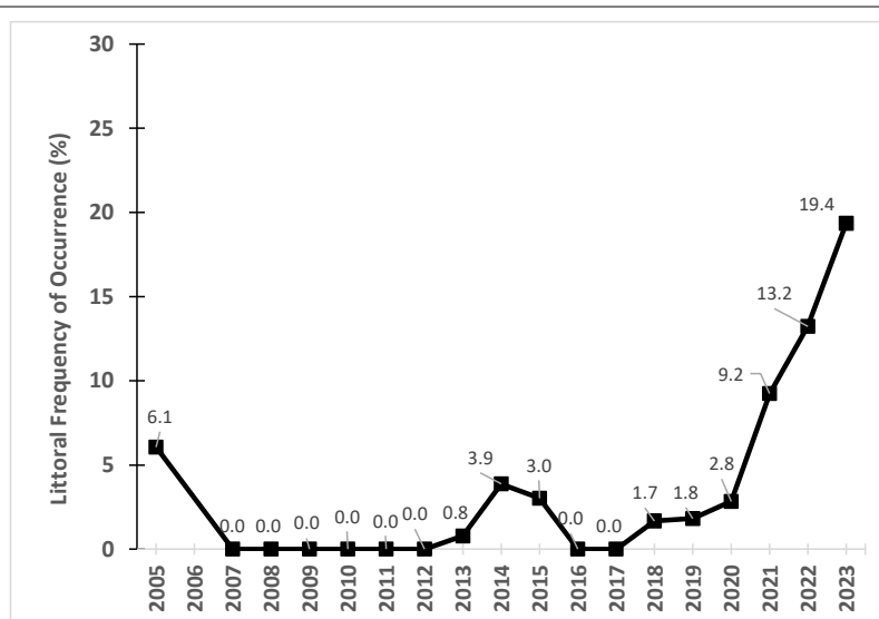
Figure 2.2-2. Littoral occurrence of EWM in Silver Lake. Created using data from whole-lake point-intercept surveys.
