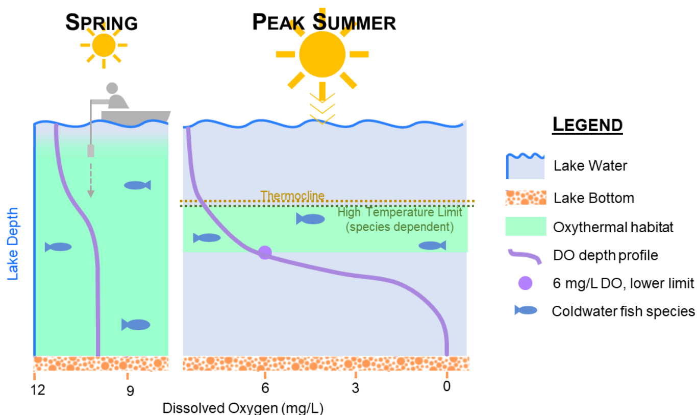
Figure 13. Availability of oxythermal habitat for coldwater fish species during the spring and summer in a two-story fishery lake. In the spring suitably cool and oxygenated water (oxythermal habitat, shown in green), is available from the top of the lake to the bottom because dissolved oxygen (DO) levels are high from the water's mixing in the spring (DO is shown as a purple line, with the DO scale along the bottom of the figure). In the summer, the lake has thermally stratified (producing a thermocline) and oxythermal habitat is limited in the top layer of the lake by warm temperatures. From below, oxythermal habitat is limited by low DO caused by oxygen depletion in the lake bottom. If a lake does not maintain a DO above 6 mg/L and with sufficiently cold temperatures, it is not fully protective of a healthy coldwater fish community, as reflected in new oxythermal criteria.
