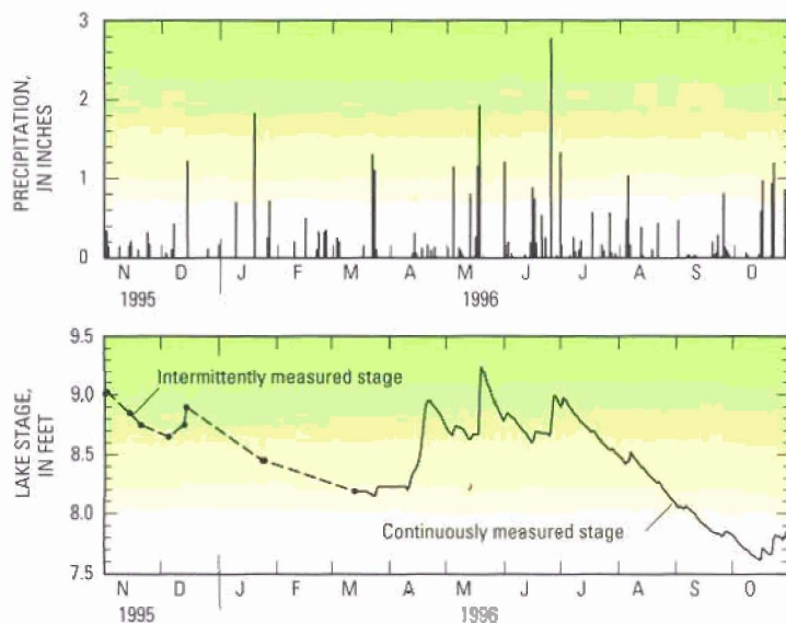
Figure 3. Daily precipitation at, and lake stage of, Kirby Lake.
