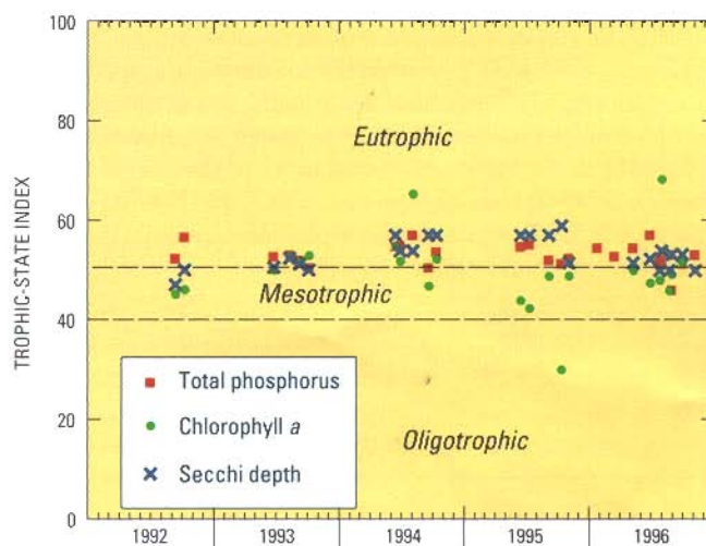
Figure 6. Trophic-state indices for total phosphorus, chlorophyll a , and Secchi depth for Kirby Lake.
