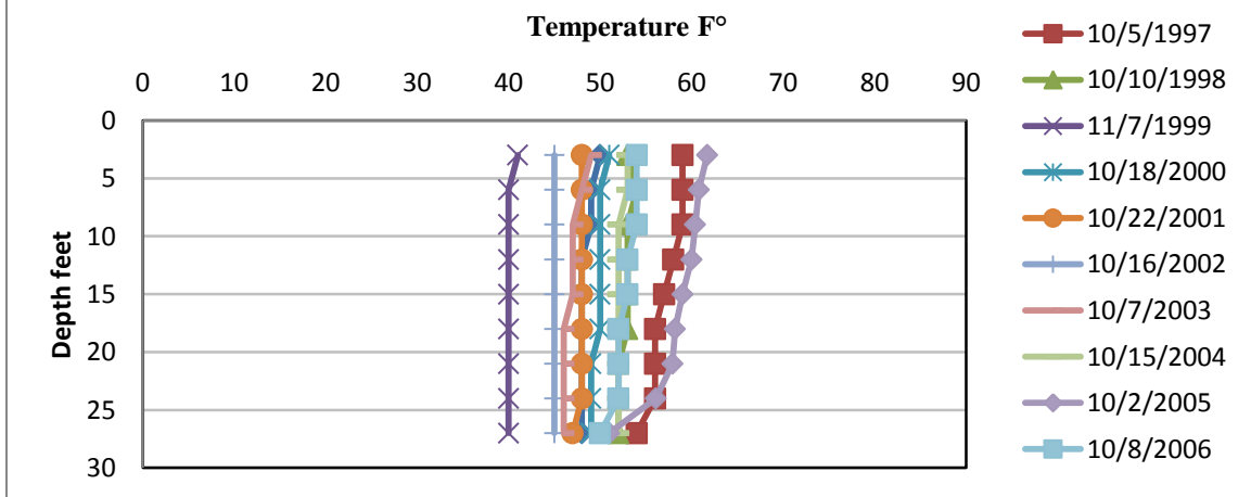
Figure 7. Annabelle Lake temperature profile, October-November (1996-2006).
