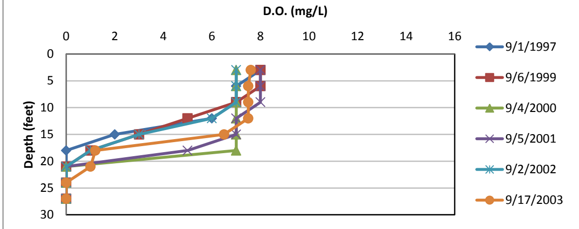
Figure 12. Annabelle Lake dissolved oxygen profile, September (1997-2003).
