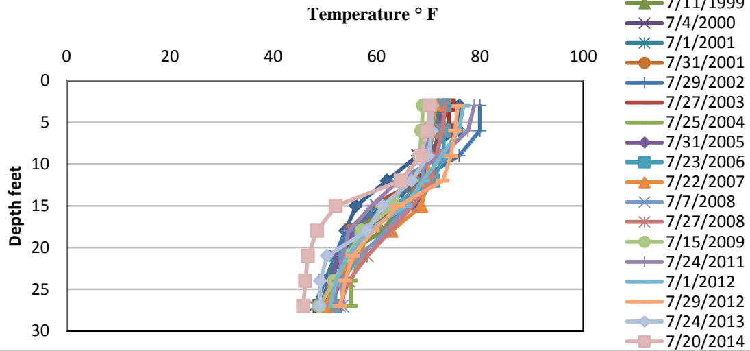
Figure 4. Annabelle Lake temperature profile, July (1997-2014).
