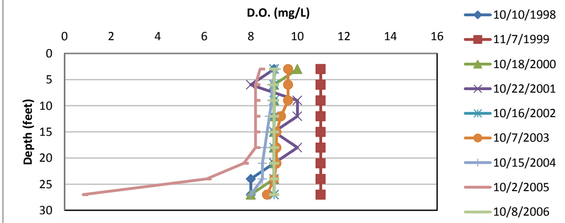
Figure 13. Annabelle Lake dissolved oxygen profile, October-November (1998-2006).
