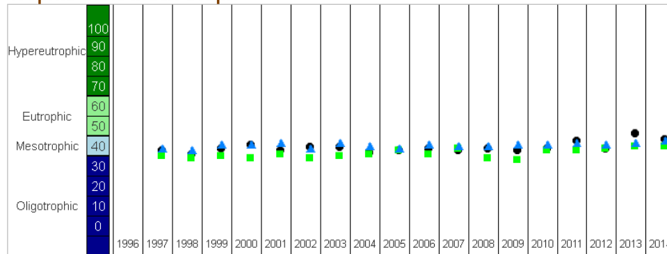
Figure 21. Annabelle Lake Trophic State Index (1997-2014).
