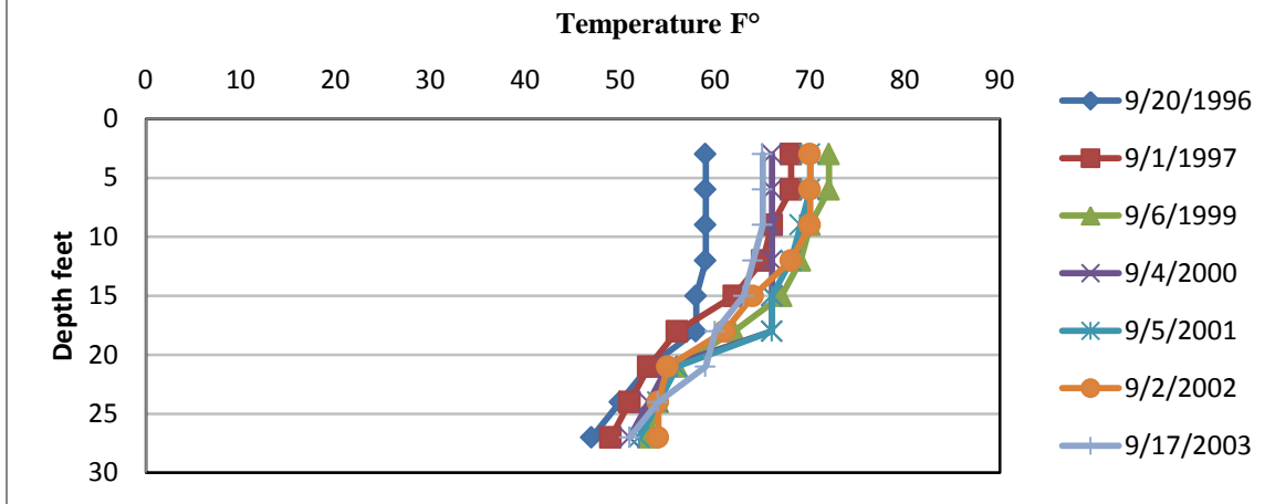
Figure 6. Annabelle Lake temperature profile, September (1996-2003).
