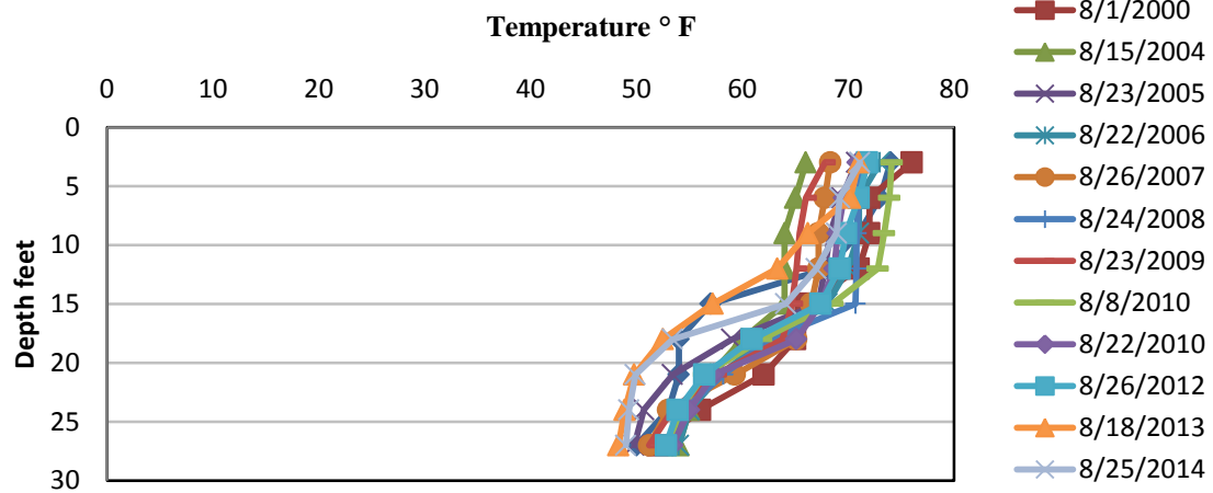
Figure 5. Annabelle Lake temperature profile, August (1998-2014).
