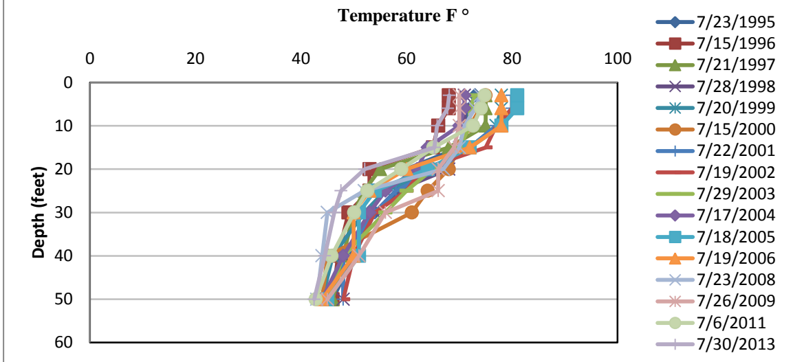
Figure 4. Crab Lake temperature profile, July.
