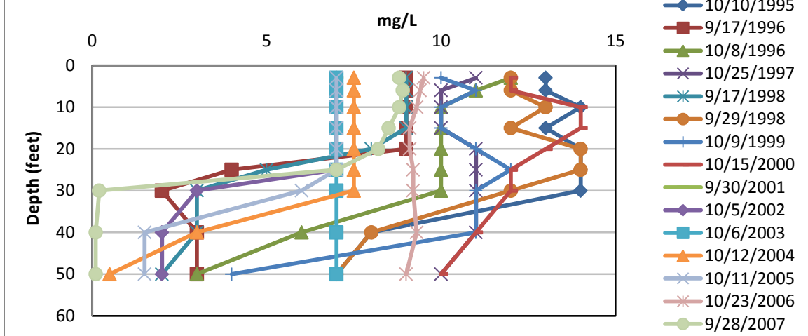
Figure 11. Crab Lake dissolved oxygen profile, September and October (1995-2007).
