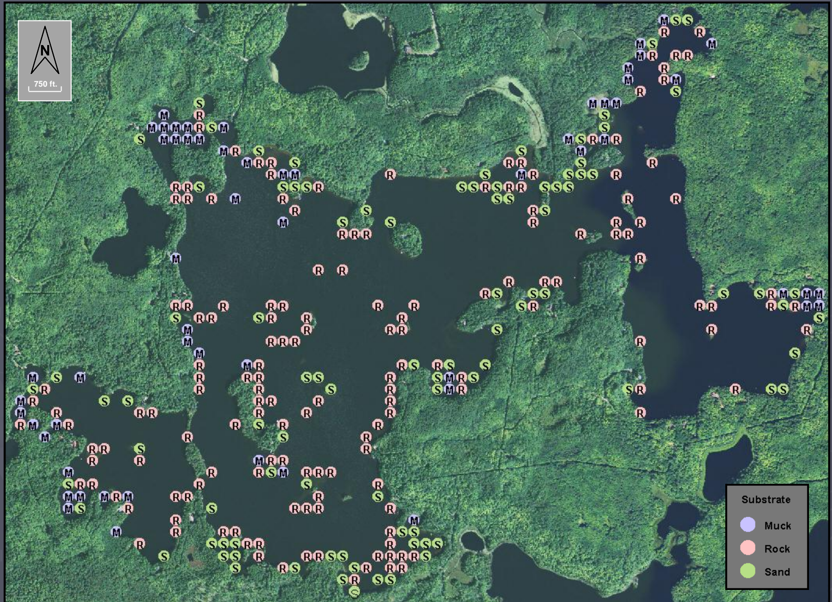
Figure 5. Crab Lake substrate encountered at point-intercept plant sampling sites (2014).
