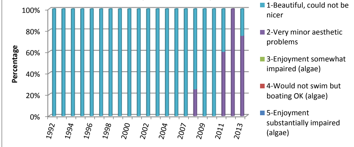
Figure 17. Crab Lake aesthetic value, (1992-2013).
