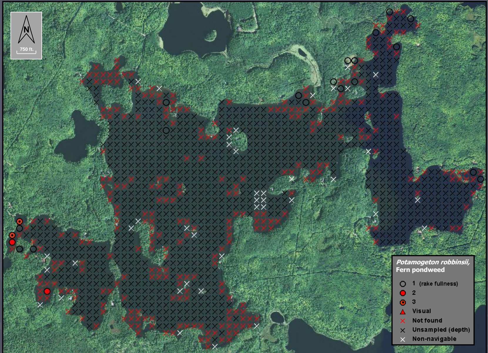
Figure 8. Distribution of plant species, Crab Lake (2014).
