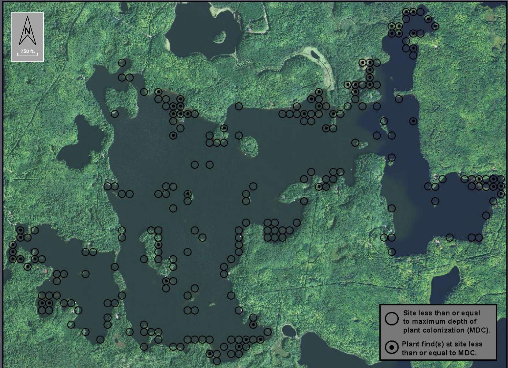
Figure 4. Crab Lake sampling sites less than or equal to maximum depth of rooted vegetation (2014).
