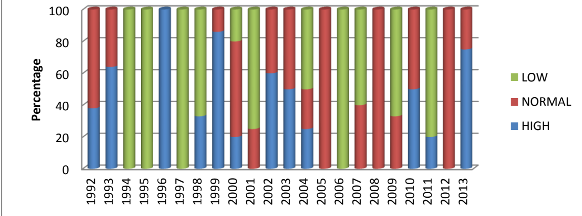
Figure 15. Crab Lake water level percentage viewed by CLMN, (1992-2013).
