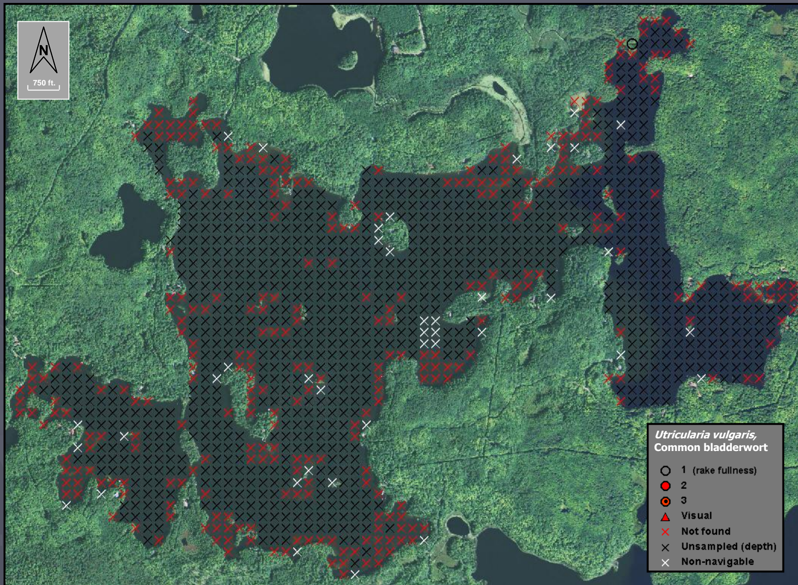
Figure 13. Distribution of plant species, Crab Lake (2014).
