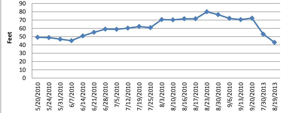
Figure 16. Crab Lake water level, 2010 and 2013.
