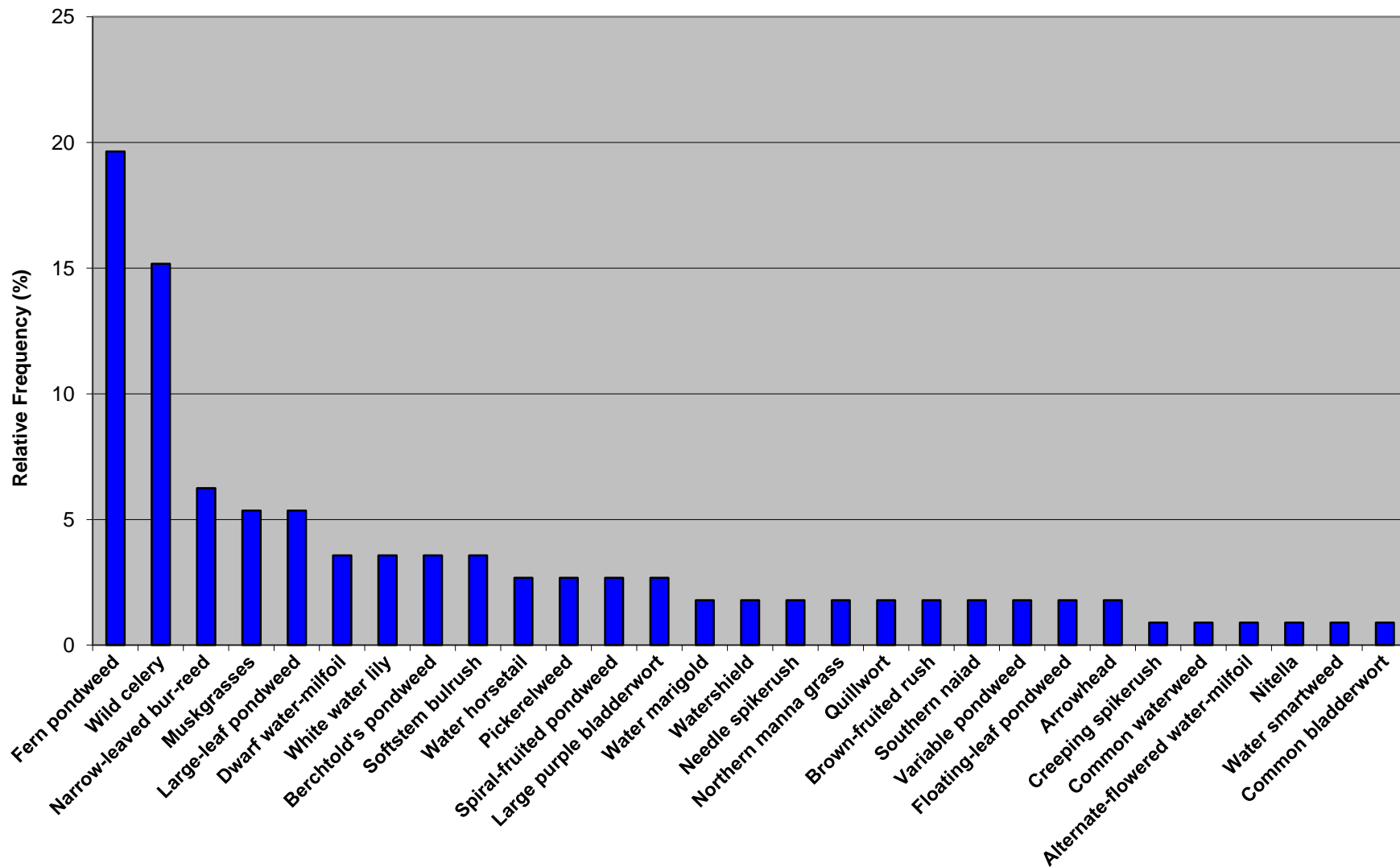
Figure 6. Crab Lake aquatic plant occurrences for 2014 point-intercept survey data.
