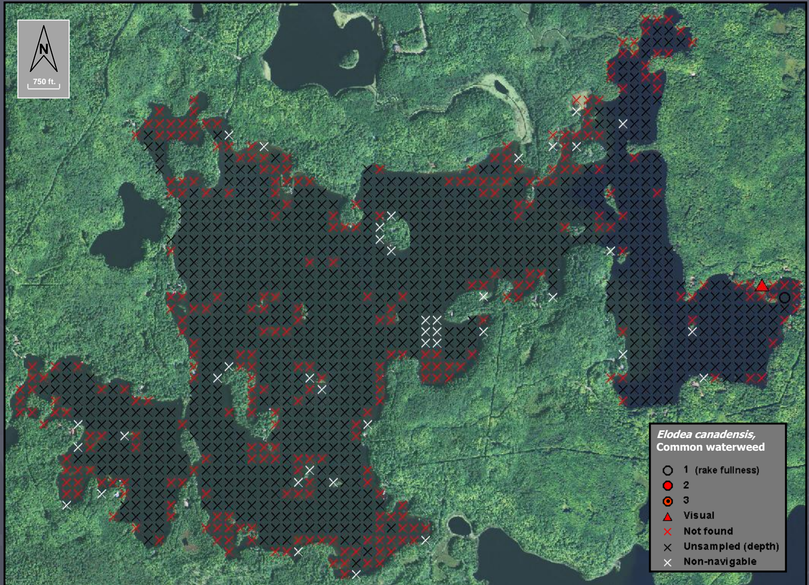
Figure 12. Distribution of plant species, Crab Lake (2014).
