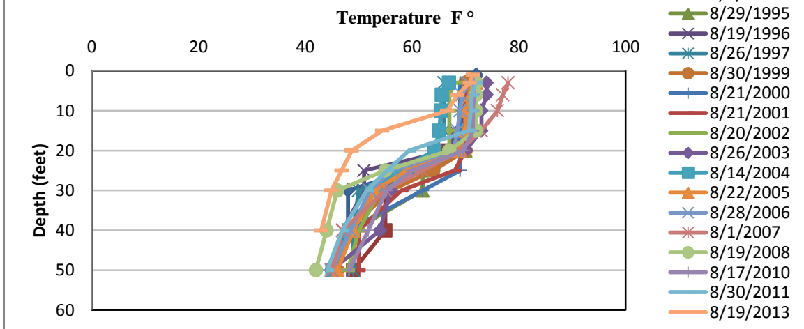
Figure 5. Crab Lake temperature profile, August.
