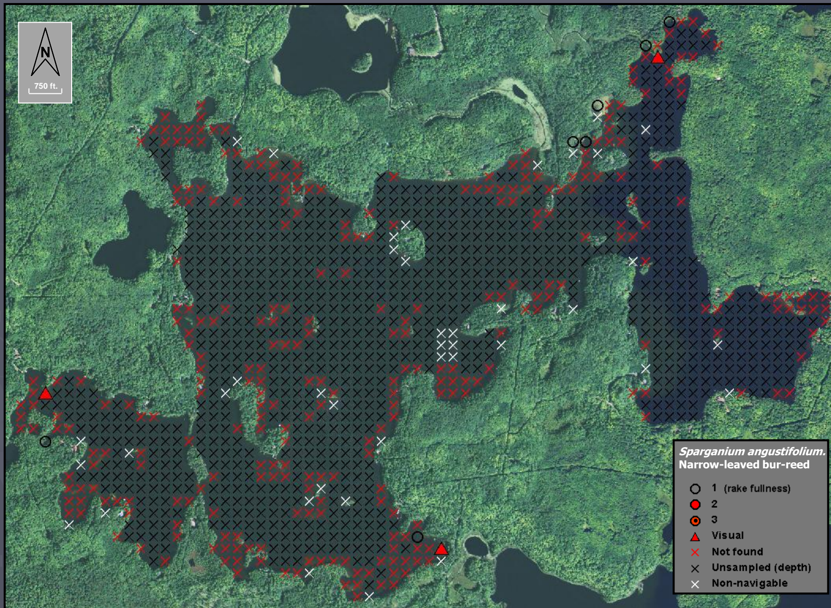
Figure 10. Distribution of plant species, Crab Lake (2014).
