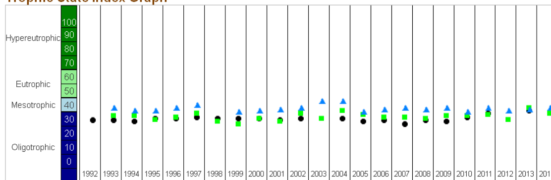
Figure 22. Crab Lake Trophic State Index (1992-2014).
