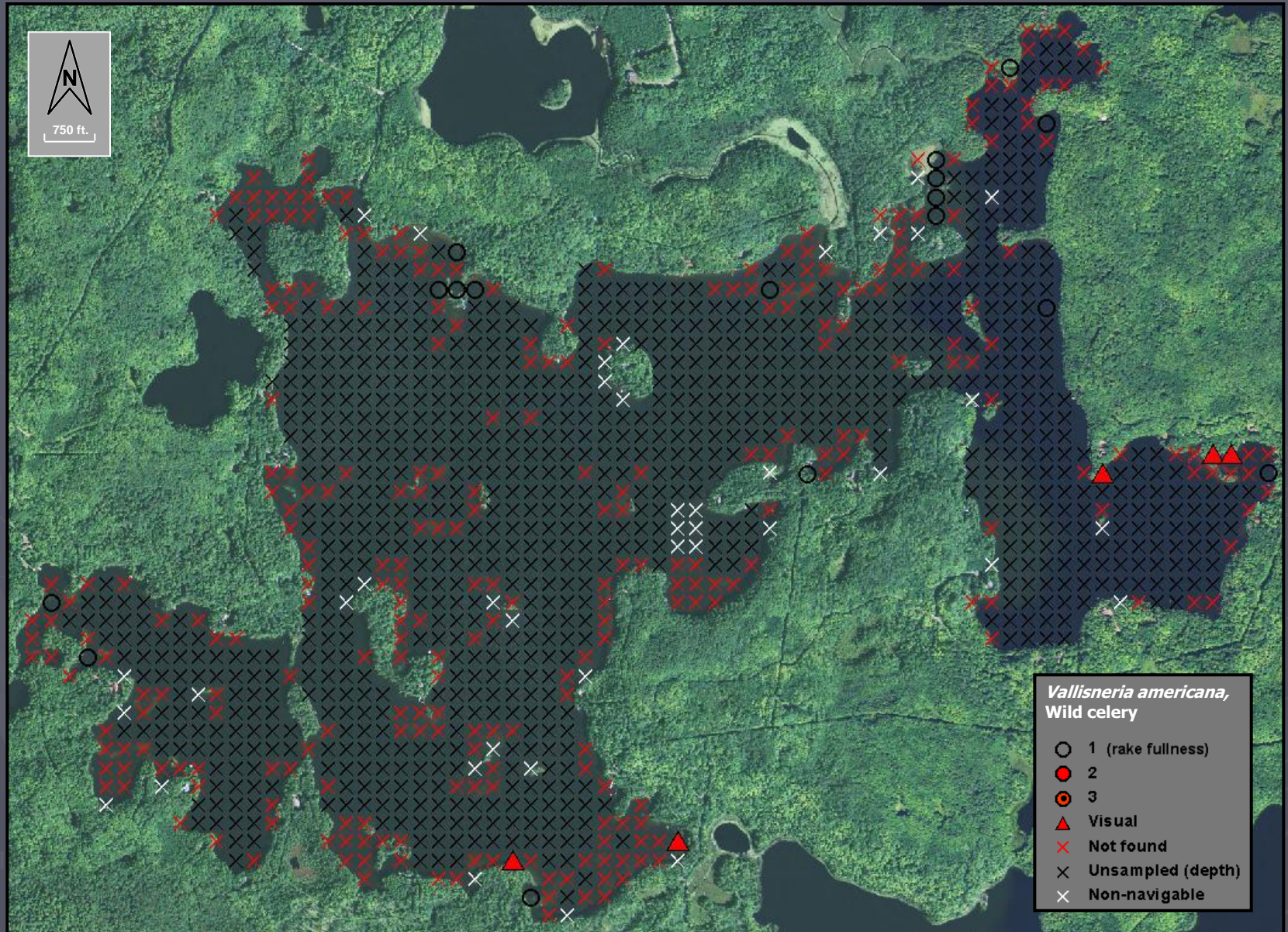
Figure 9. Distribution of plant species, Crab Lake (2014).
