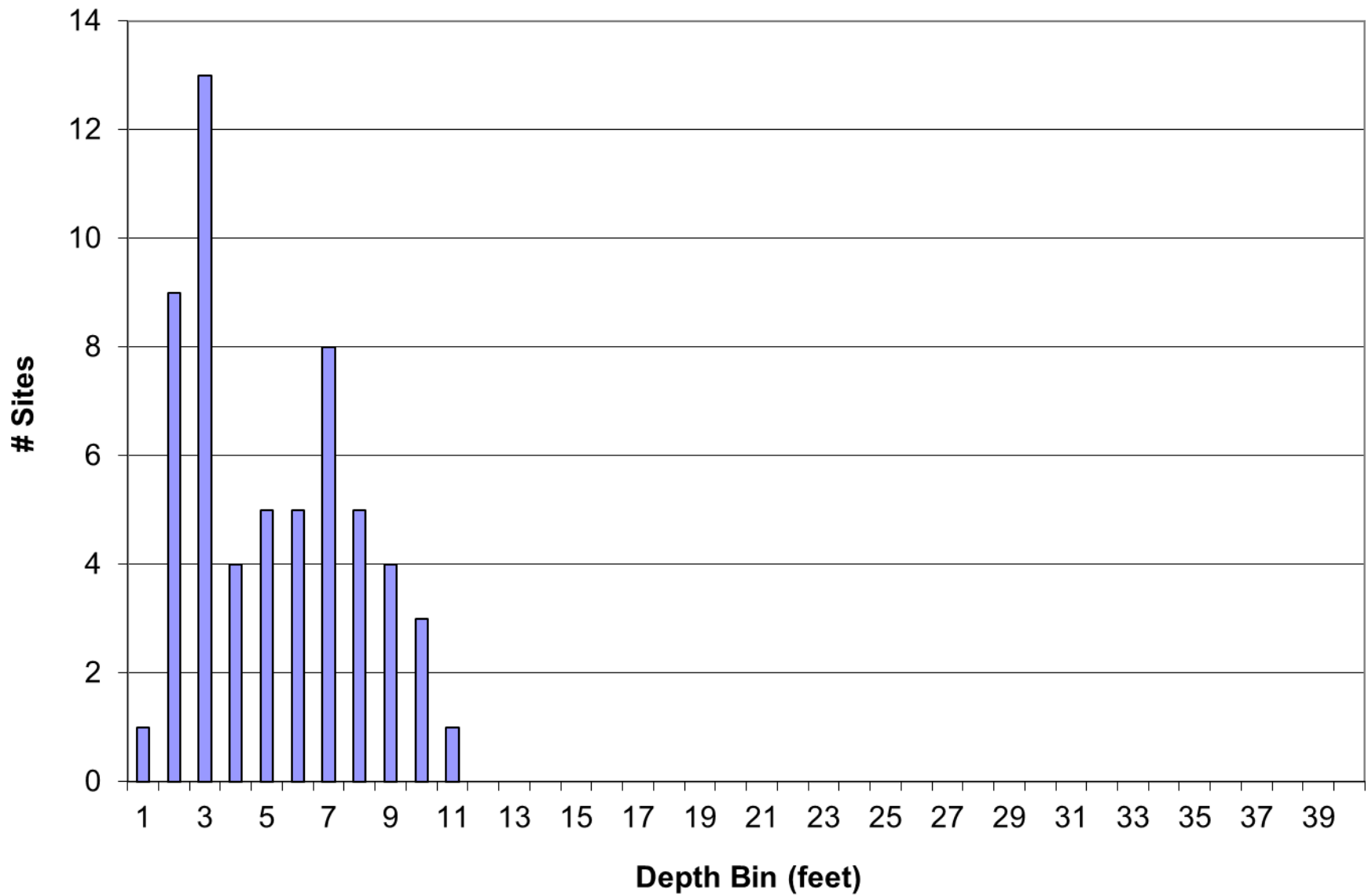
Figure 3. Maximum Depth of Plant Colonization in Crab Lake, 2014.
