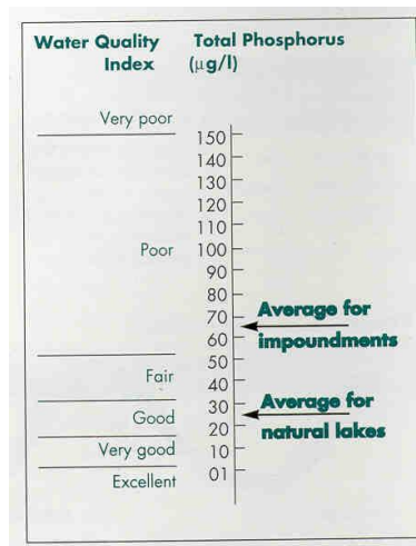
Figure 21. Total phosphorus concentrations for Wisconsin’s natural lakes and impoundments (Shaw et al., 2004).
