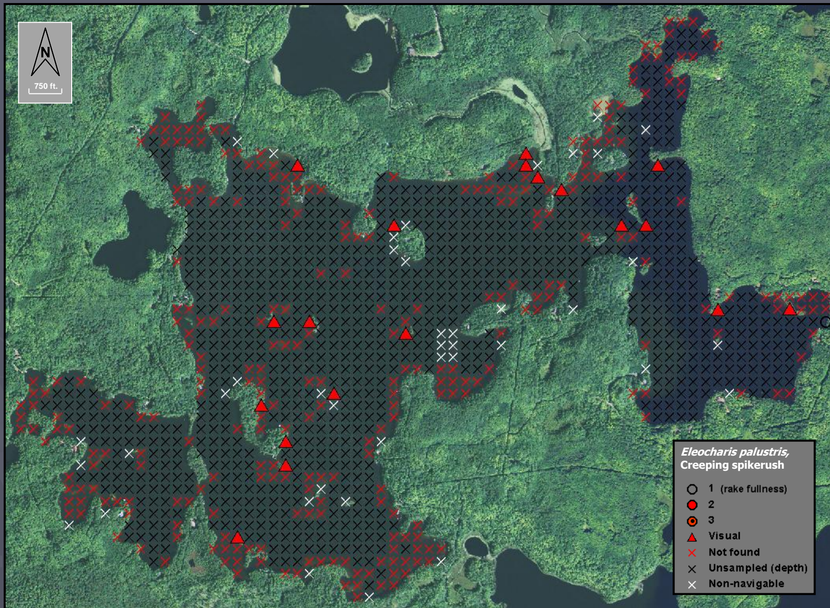
Figure 11. Distribution of plant species, Crab Lake (2014).
