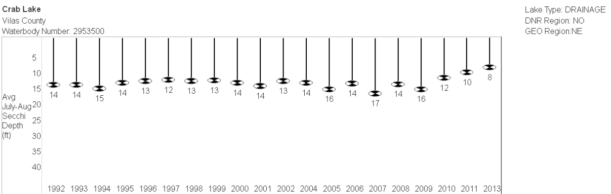
Figure 12. Crab Lake Secchi depth averages (July and August only).
