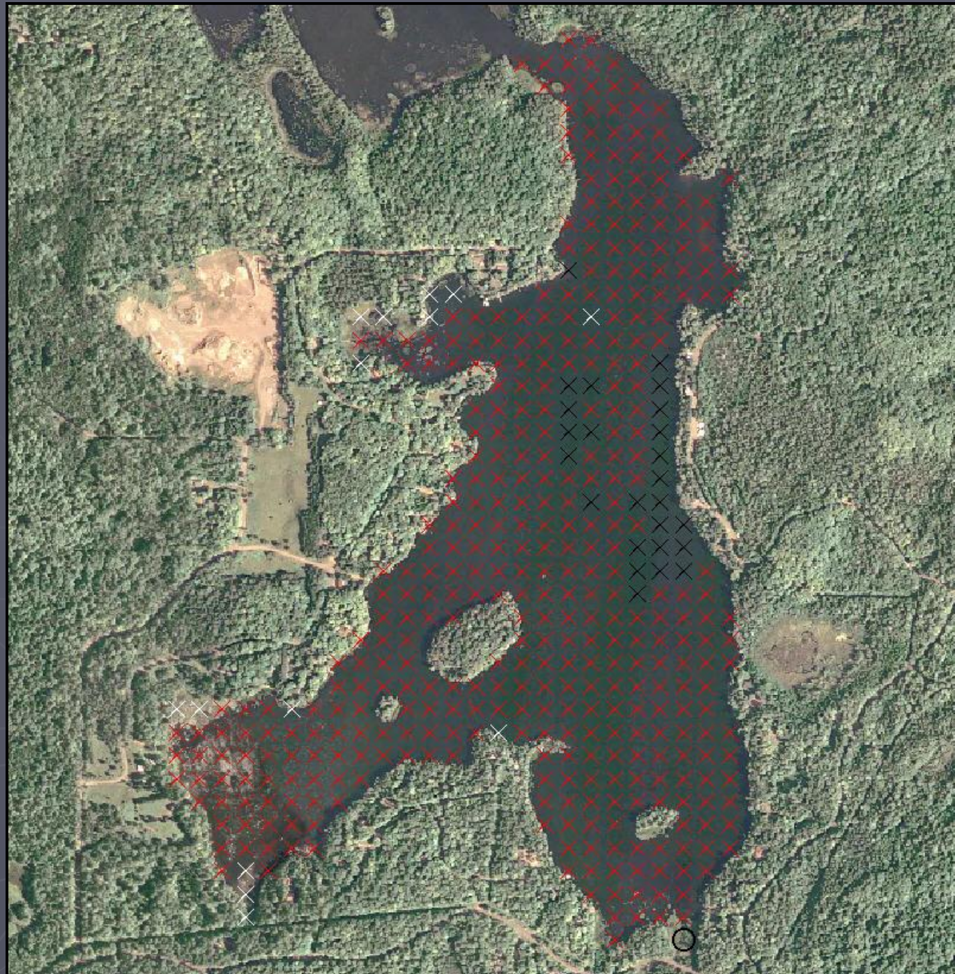
Figure 15. Distribution of plant species, Van Vliet Lake (2013).
