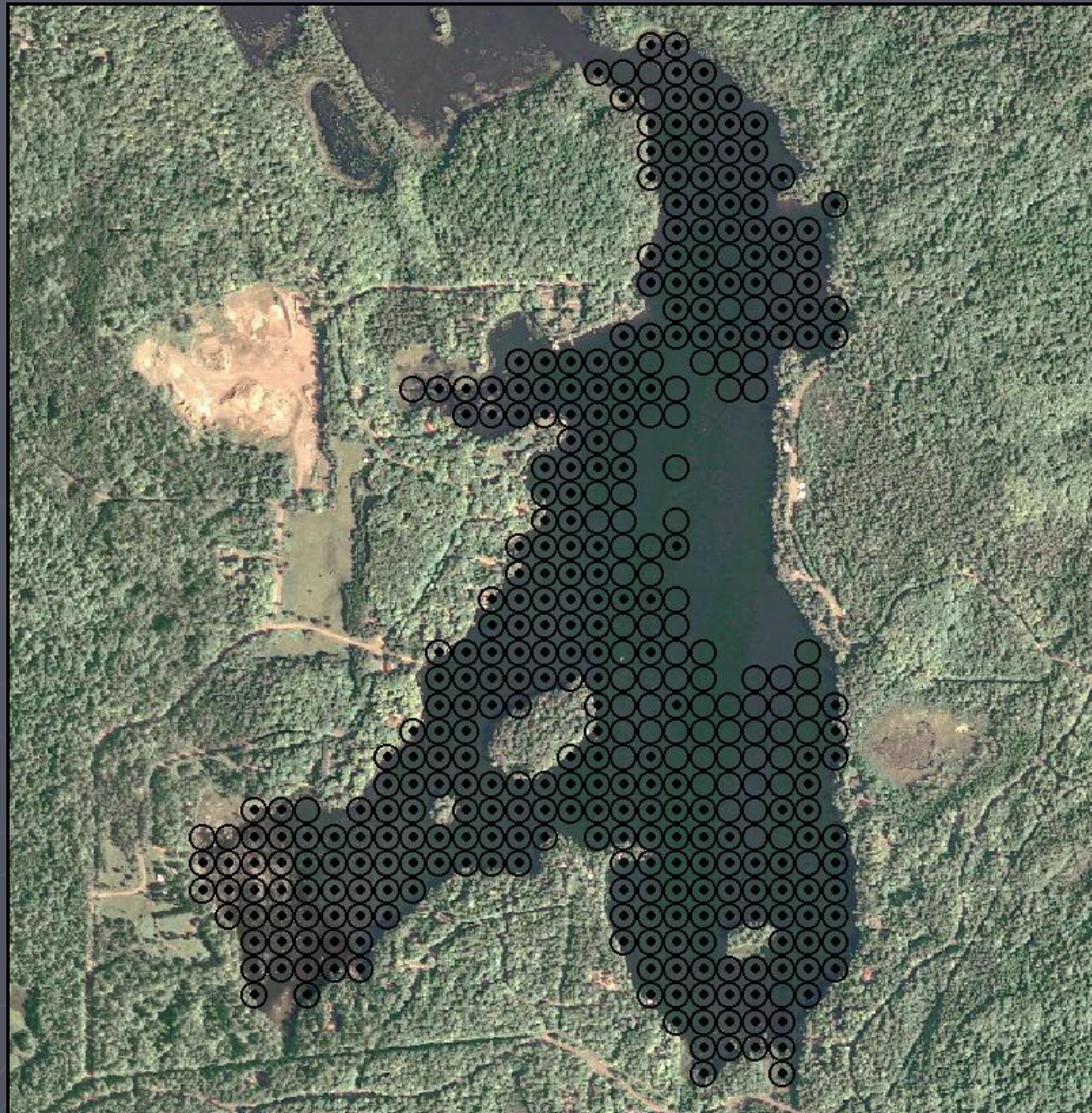
Figure 4. Van Vliet Lake sampling sites less than or equal to maximum depth of rooted vegetation (2013).
