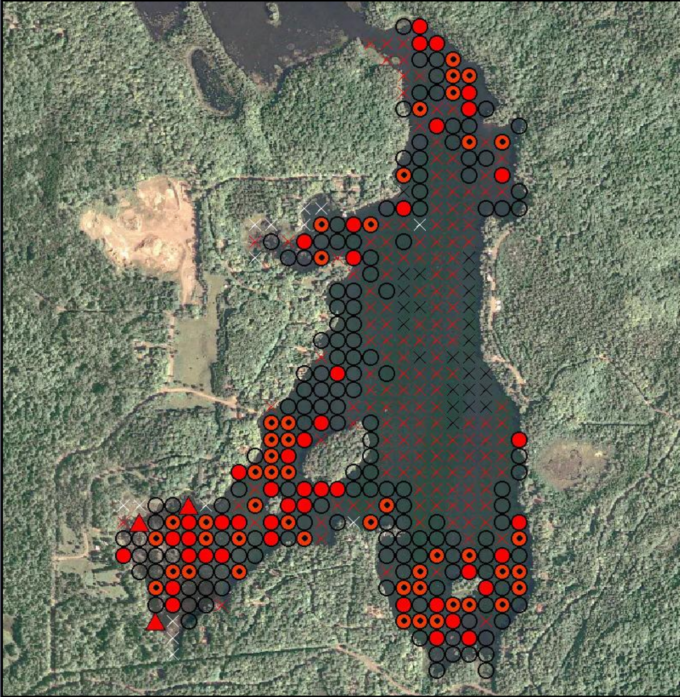
Figure 8. Distribution of plant species, Van Vliet Lake (2013).
