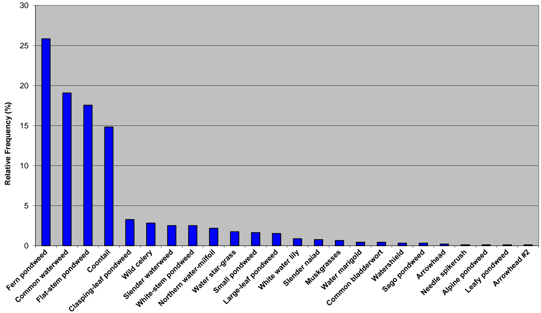
Figure 6. Van Vliet Lake aquatic plant occurrences for 2013 point-intercept survey data.
