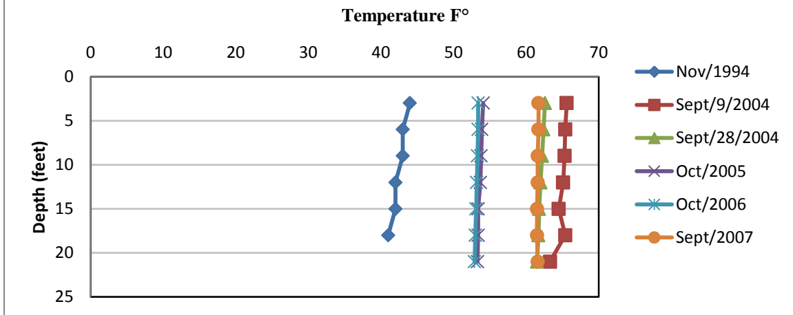
Figure 6. Van Vliet temperature profile September, October, November.
