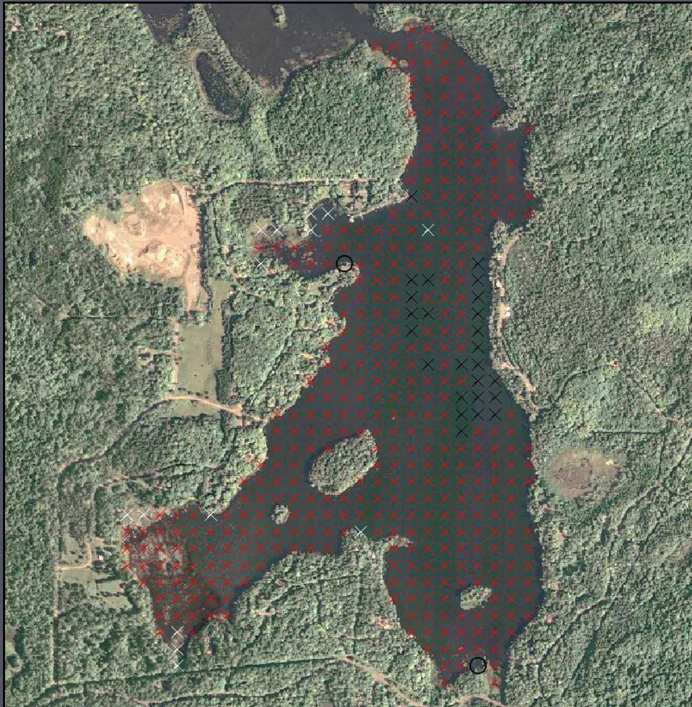
Figure 12. Distribution of plant species, Van Vliet Lake (2013).
