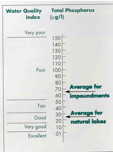
Figure 19. Total phosphorus concentrations for Wisconsin’s natural lakes and impoundments (Shaw et al., 2004).
