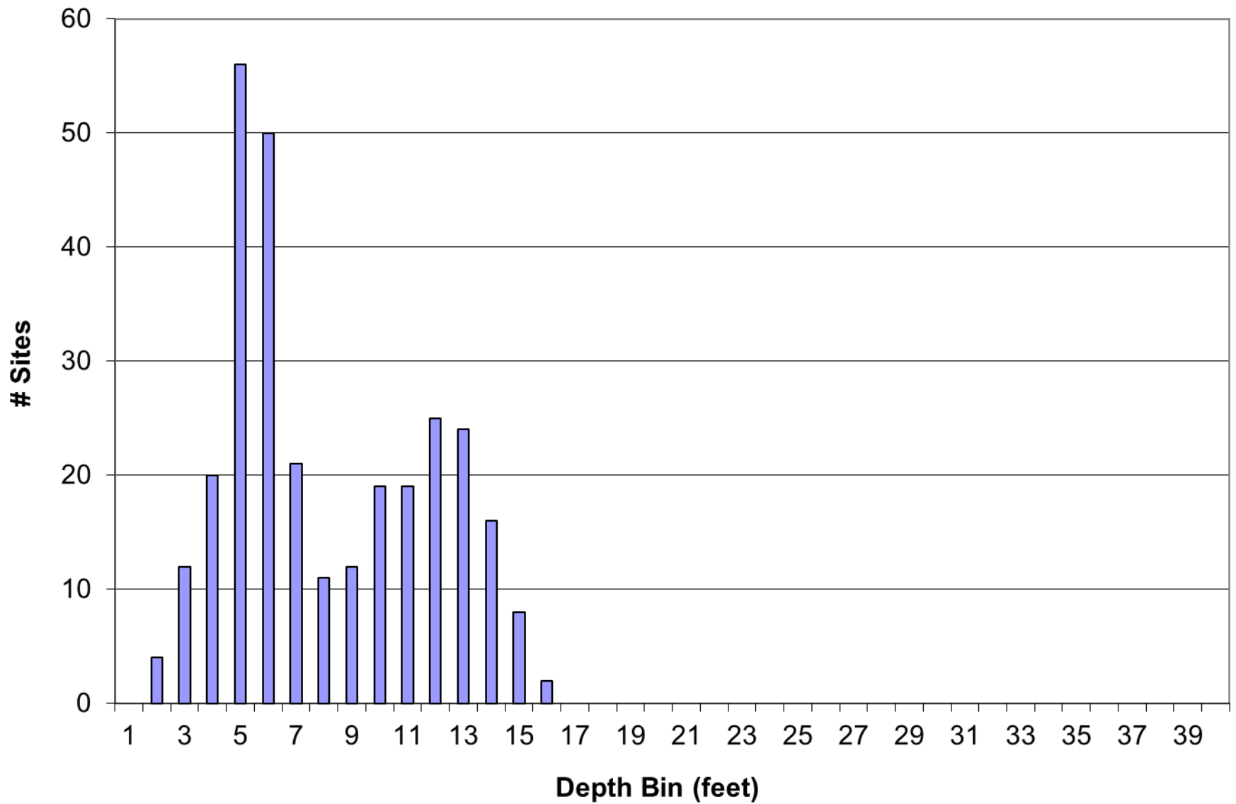
Figure 3. Maximum Depth of Plant Colonization in Van Vliet Lake.
