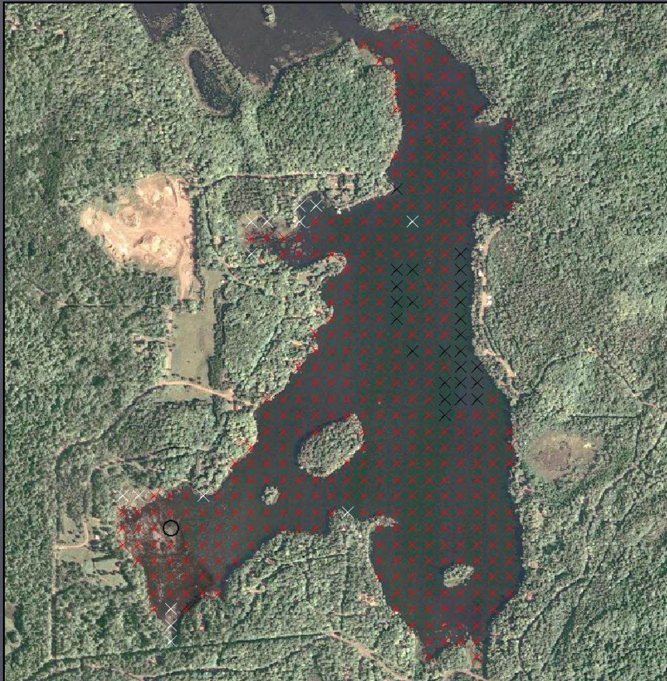
Figure 13. Distribution of plant species, Van Vliet Lake (2013).
