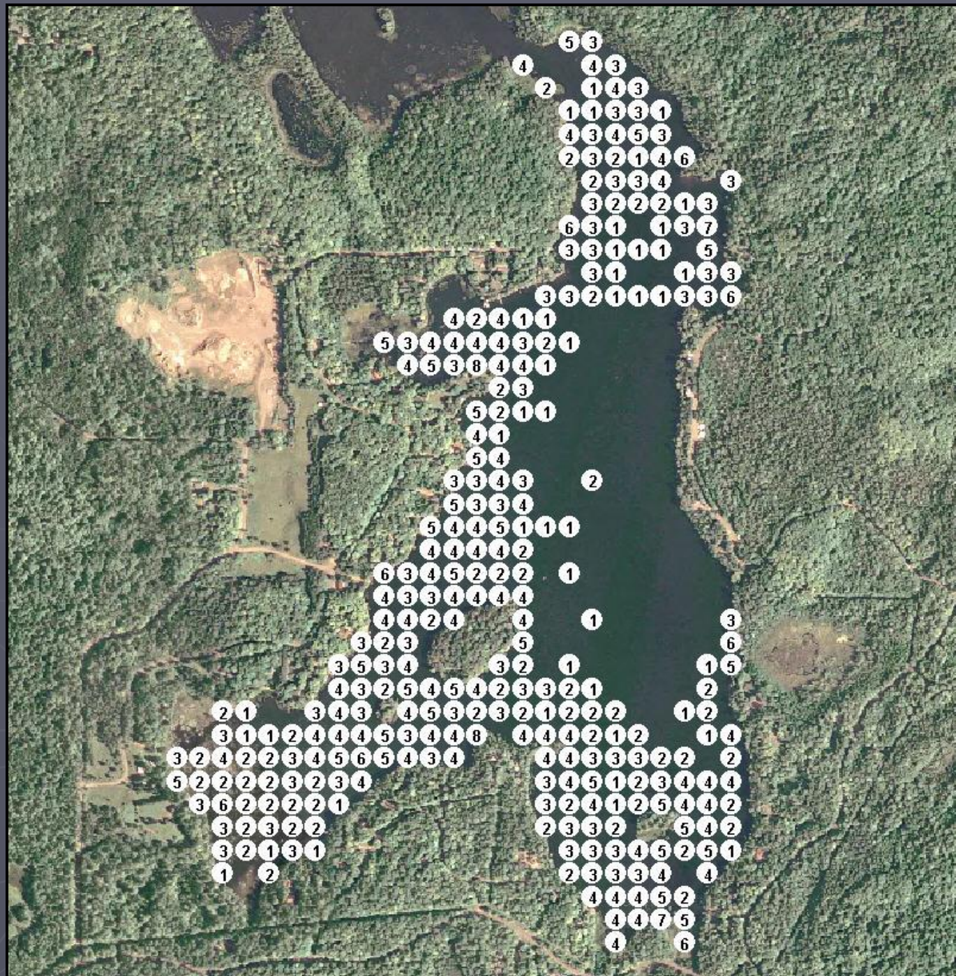
Figure 1. Number of plant species recorded at Van Vliet Lake sample sites (2013).
