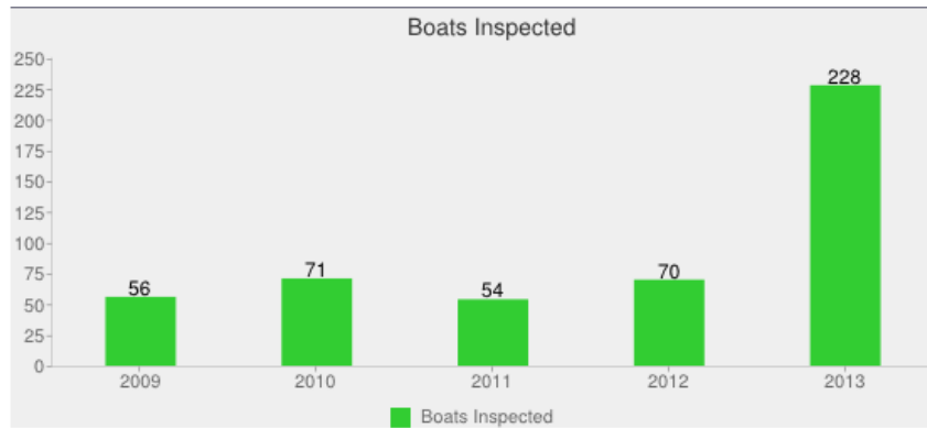
Figure 21. Van Vliet Lake Clean Boats Clean Waters data (WDNR, 2014a).
