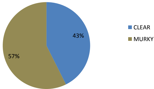
Figure 13. Van Vliet water appearance, 2002-2013.
