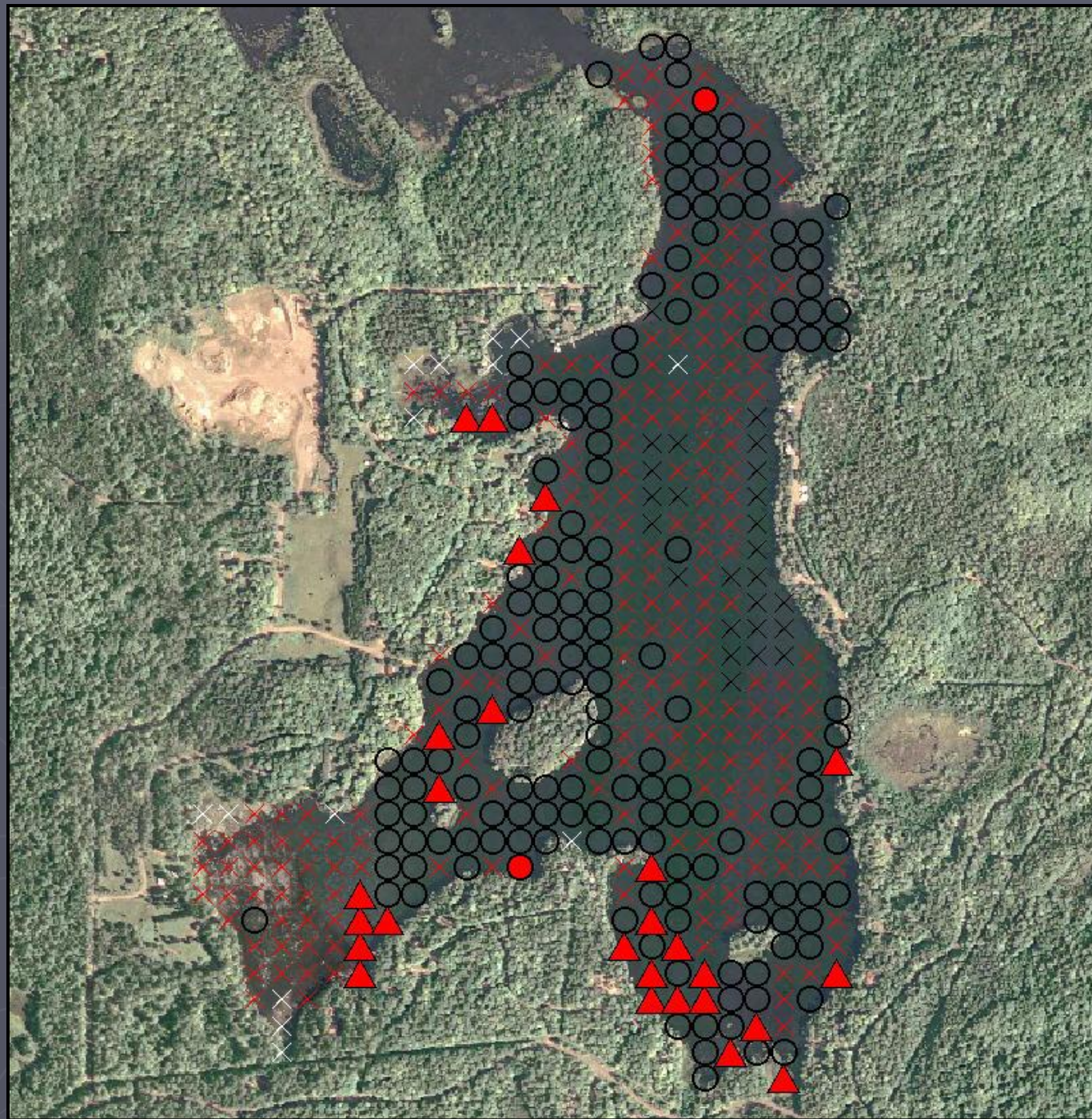
Figure 10. Distribution of plant species, Van Vliet Lake (2013).
