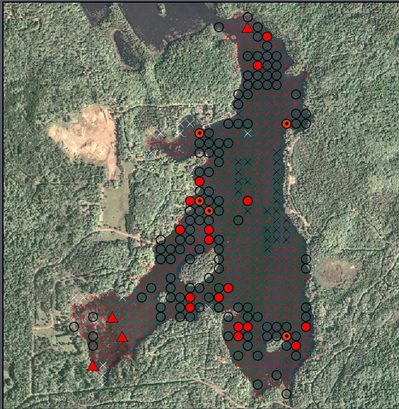
Figure 11. Distribution of plant species, Van Vliet Lake (2013).
