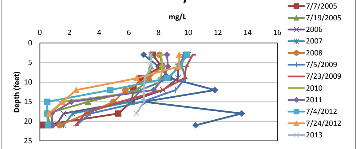
Figure 8. Van Vliet dissolved oxygen profile July.
