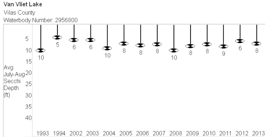
Figure 11. Van Vliet Lake Secchi depth averages (July and August only).
