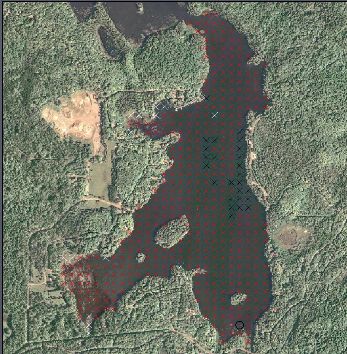
Figure 14. Distribution of plant species, Van Vliet Lake (2013).
