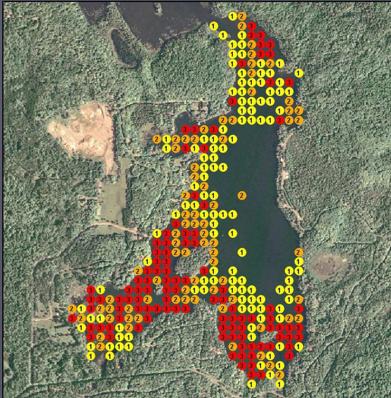
Figure 2. Rake fullness ratings for Van Vliet Lake sample sites (2013).
