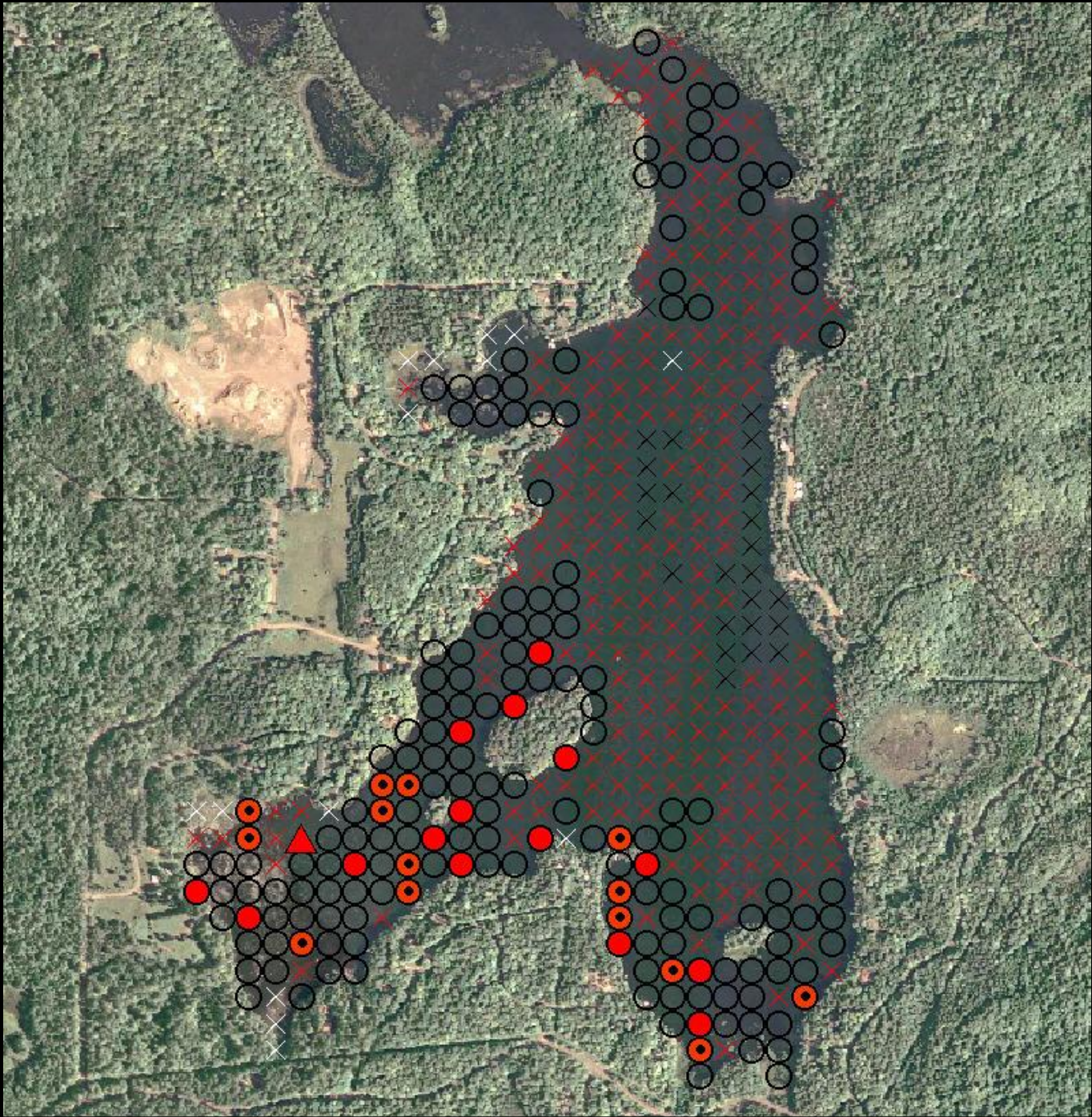
Figure 9. Distribution of plant species, Van Vliet Lake (2013).
