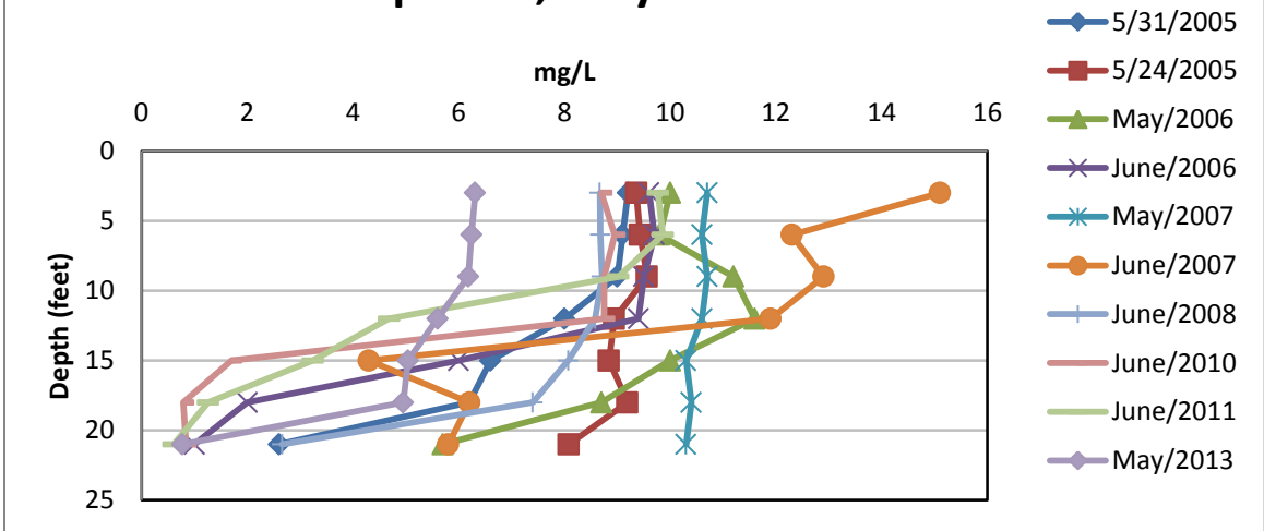
Figure 7. Van Vliet Lake dissolved oxygen profile, May and June.
