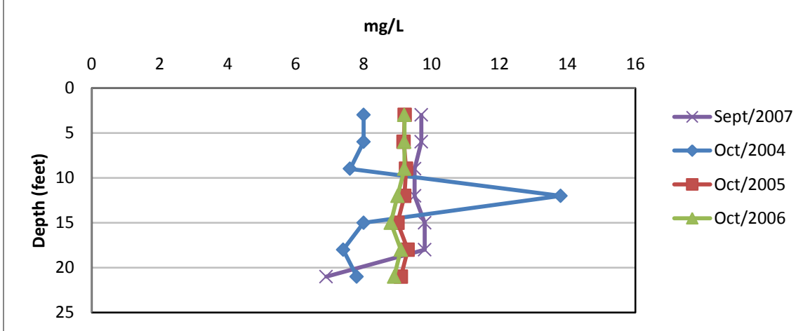
Figure 10. Van Vliet dissolved oxygen profile Septebmer and October.
