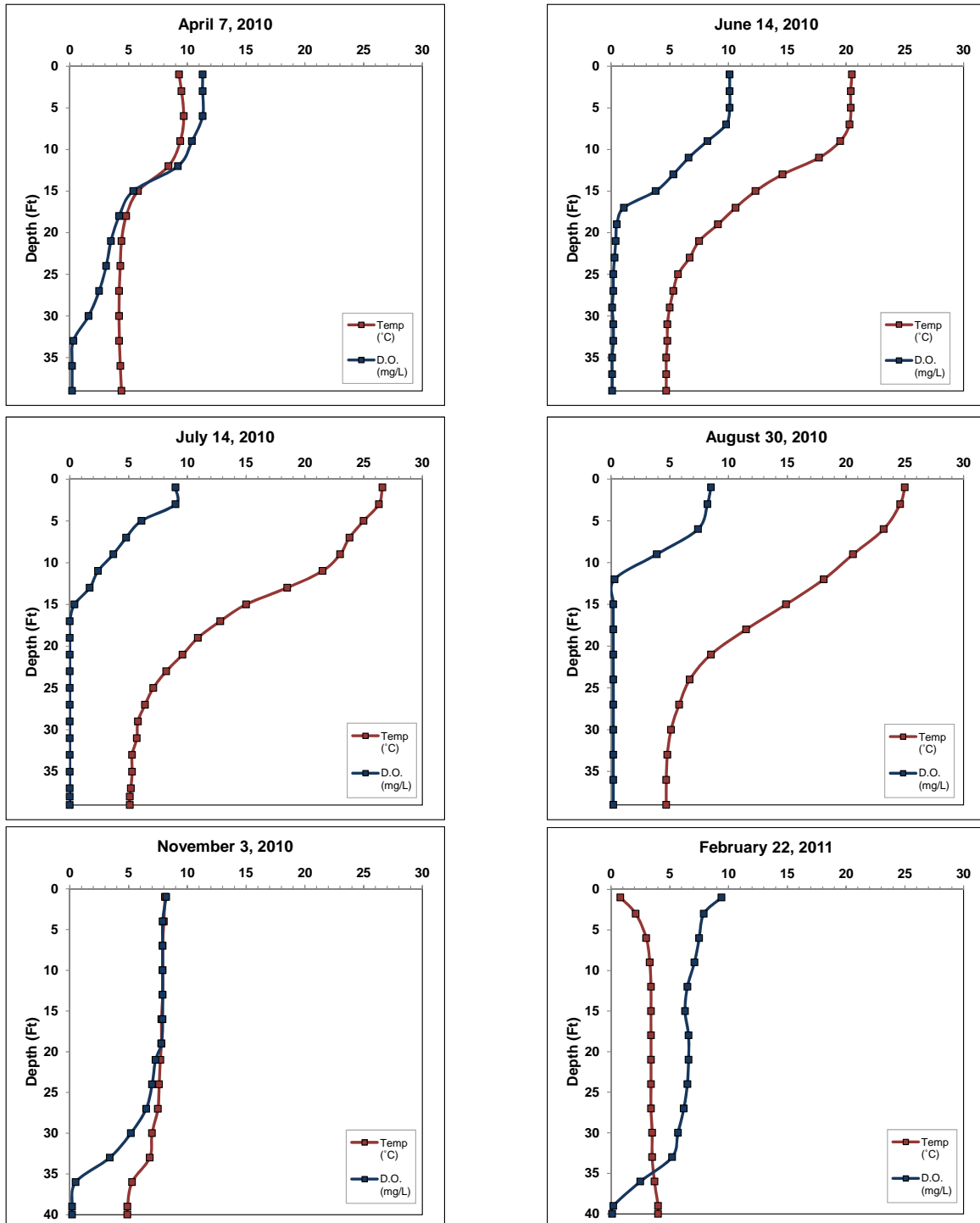
Figure 3.1-24. Mount Morris Lake D dissolved oxygen and temperature profiles.
