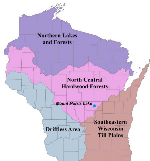
Figure 3.1-2. Location of Mount Morris Lake within the ecoregions of Wisconsin. After Nichols 1999.
