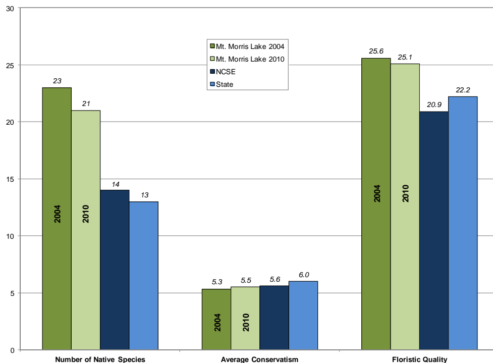
Figure 3.3-4 Mount Morris Lake Floristic Quality Assessment. Created using data from 2004 and 2010 aquatic plant point-intercept surveys. Analysis follows Nichols (1999).
