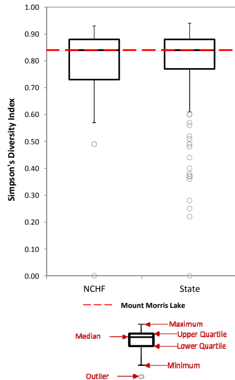
Figure 3.3-5. Mount Morris Lake species diversity index. Created using data from 2010 point-intercept surveys.
