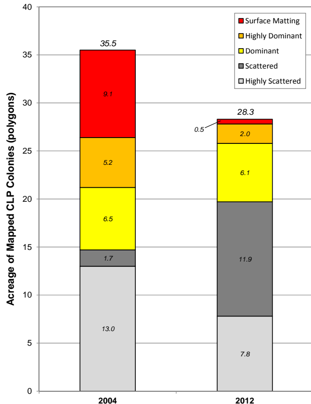
Figure 3.3-9. Acreage of mapped CLP colonies on Mount Morris Lake from 2004 and 2012.
