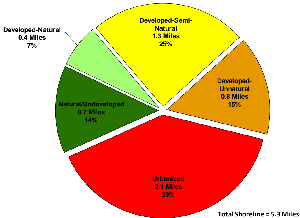
Figure 3.2-6. Mount Morris Lake shoreland categories and total lengths. Based upon a fall 2010 survey. Locations of these categorized shorelands can be found on Map 3.
