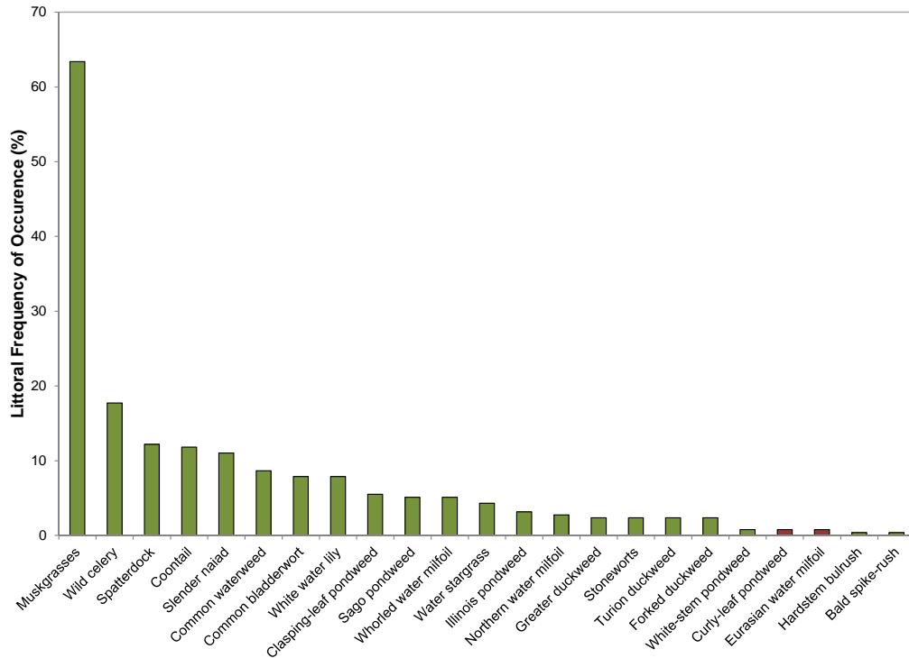
Figure 3.3-3. Mount Morris Lake aquatic plant littoral occurrence analysis. Created using data from 2010 aquatic plant point-intercept survey. Exotic species indicated with red.
