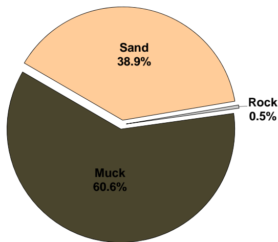
Figure 3.3-2. Mount Morris Lake proportion of substrate types within littoral areas. Created using data from 2010 aquatic plant point-intercept survey.
