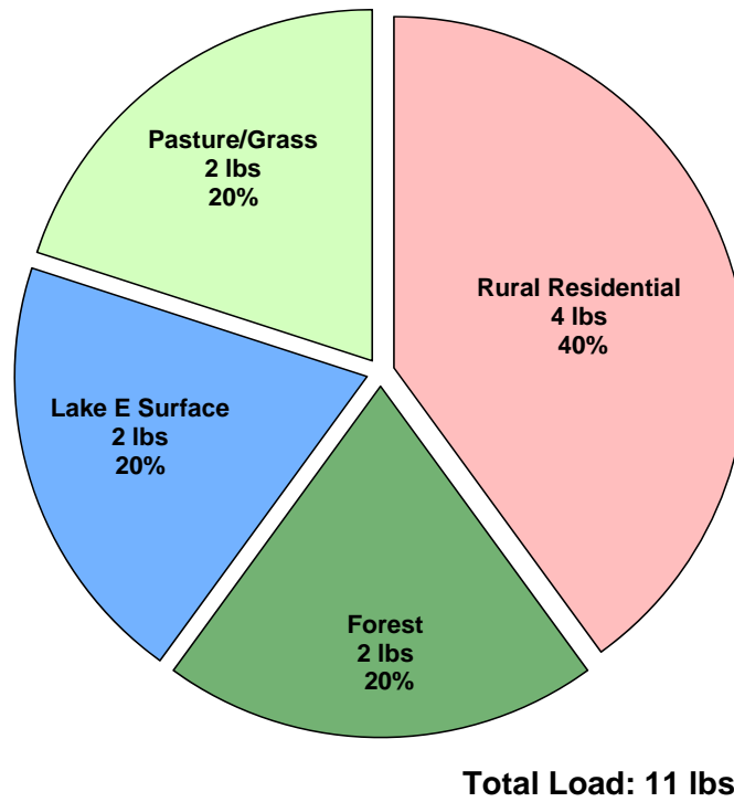
Figure 3.2-4. Lake E watershed phosphorus loading in pounds. Based upon Wisconsin Lake Modeling Suite (WiLMS) estimates.
