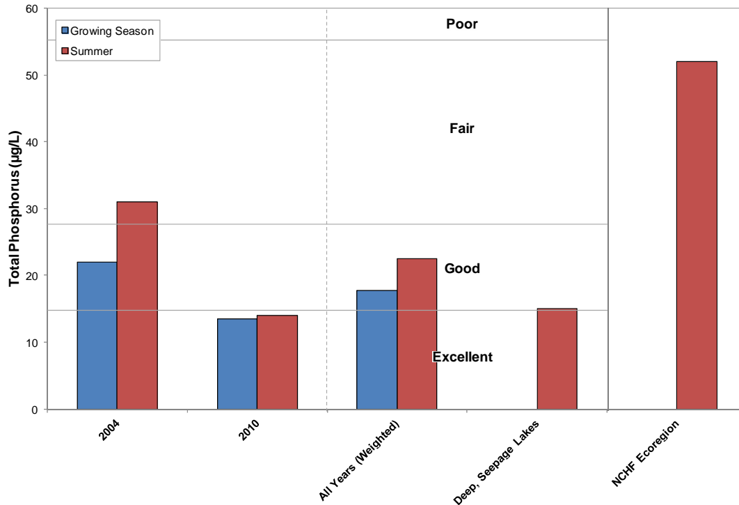
Figure 3.1-15. Mount Morris Lake E, state-wide class 3 lakes, and regional total phosphorus concentrations. Mean values calculated with summer month surface sample data. Water Quality Index values adapted from WDNR PUB WT-913.
