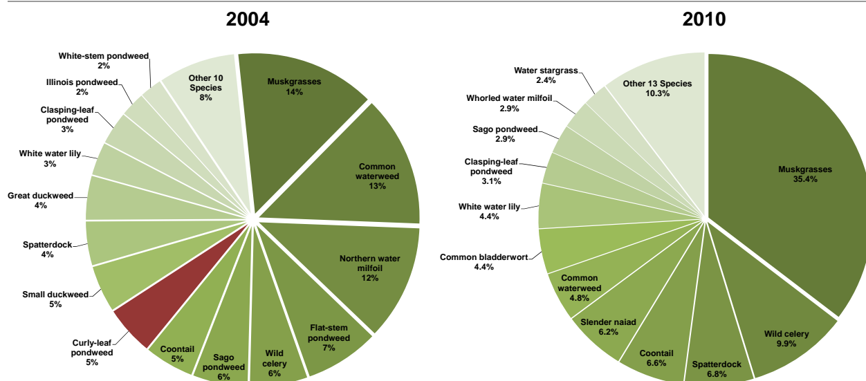
Figure 3.3-6. Mount Morris Lake aquatic plant relative occurrence analysis. Created using data from 2004 and 2010 aquatic plant point-intercept surveys. Exotic species indicated with red.
