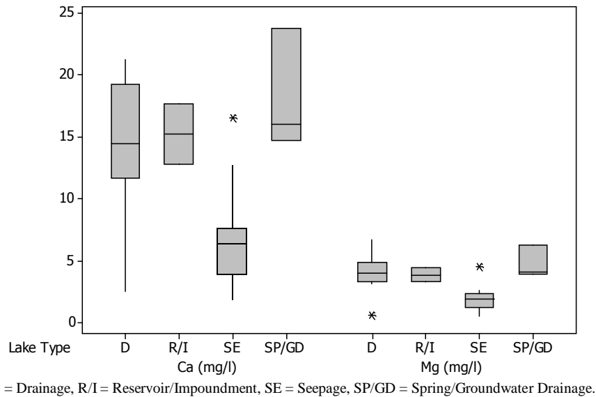
FIGURE 44. Calcium and magnesium concentrations ( \text{mg}\cdot\text{l}^{-1} ) in study lakes by lake type during overturn periods, 1979-2009.
