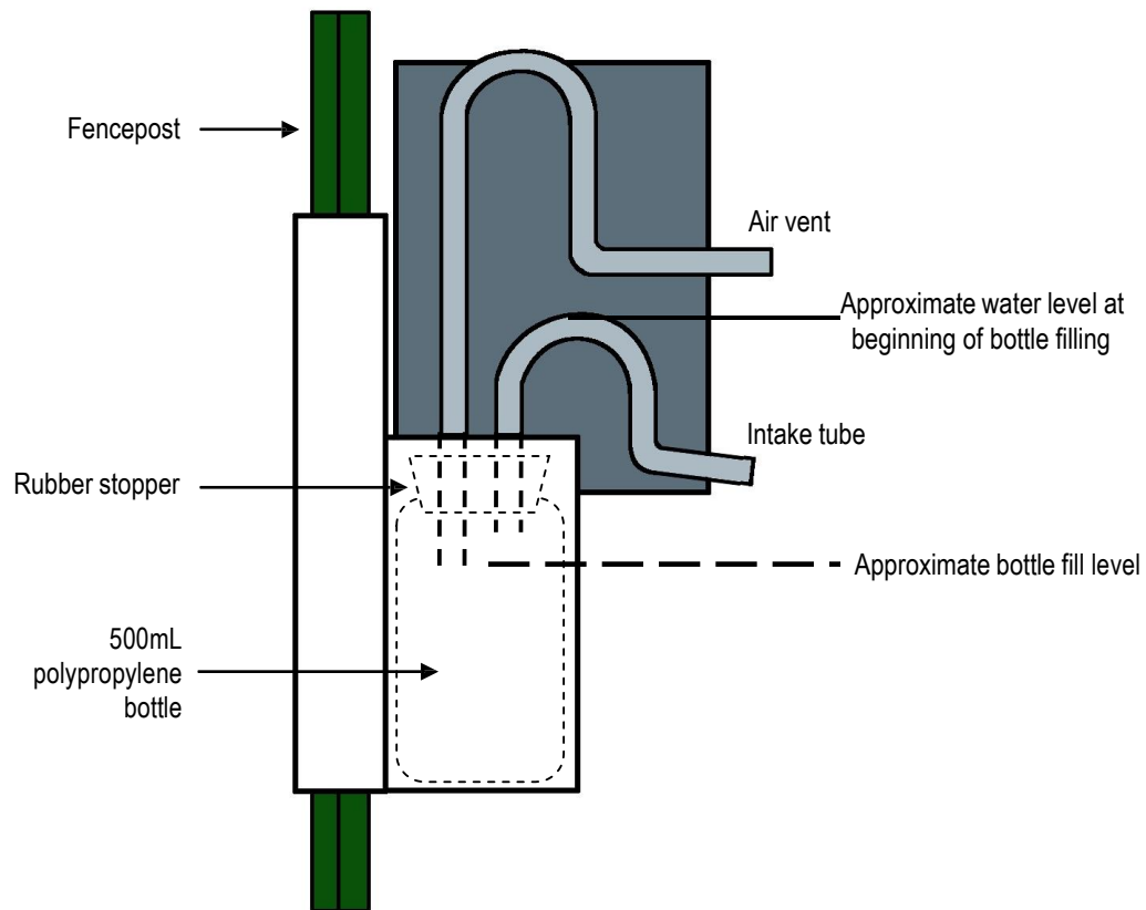
FIGURE 4. A schematic of the siphon sampler devices used in this study.
