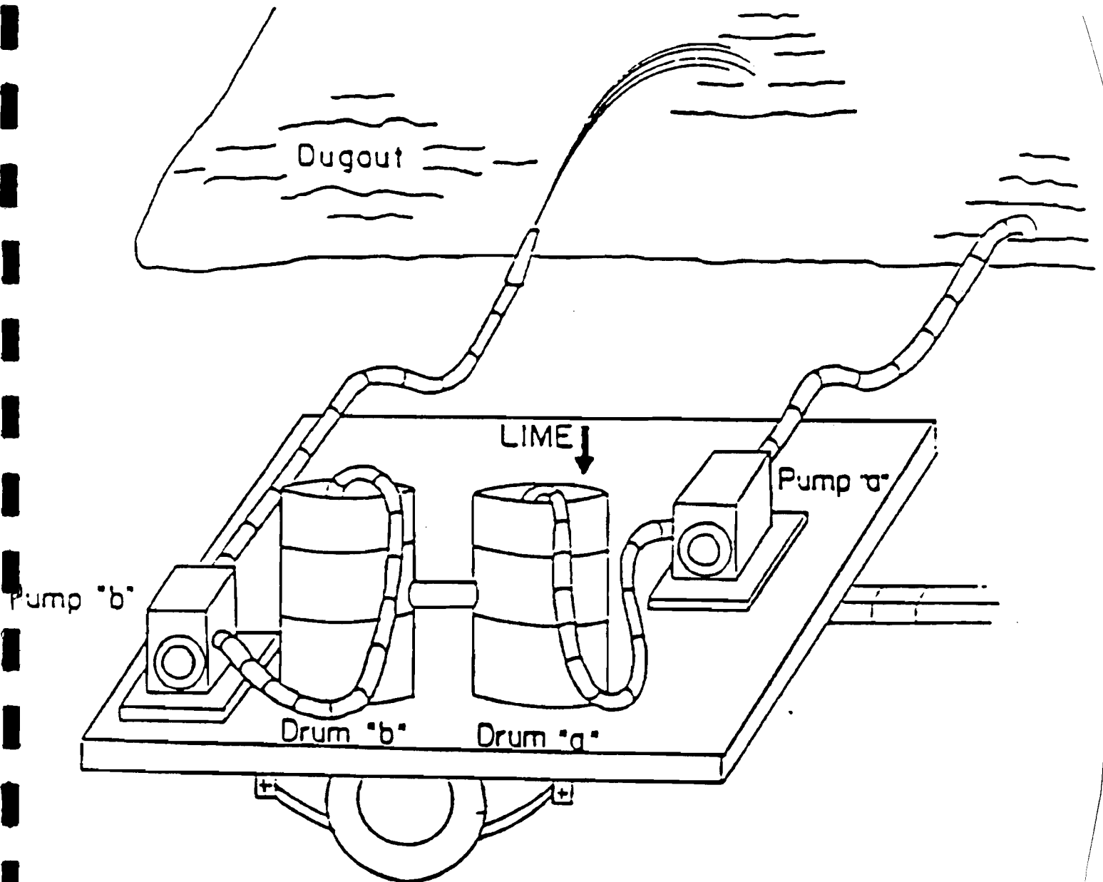
Slurry maker and trailer.
