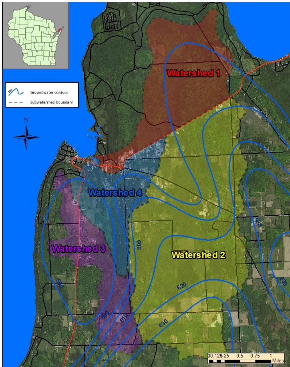
Figure 2. Fish Creek subwatersheds and groundwater contour map.
