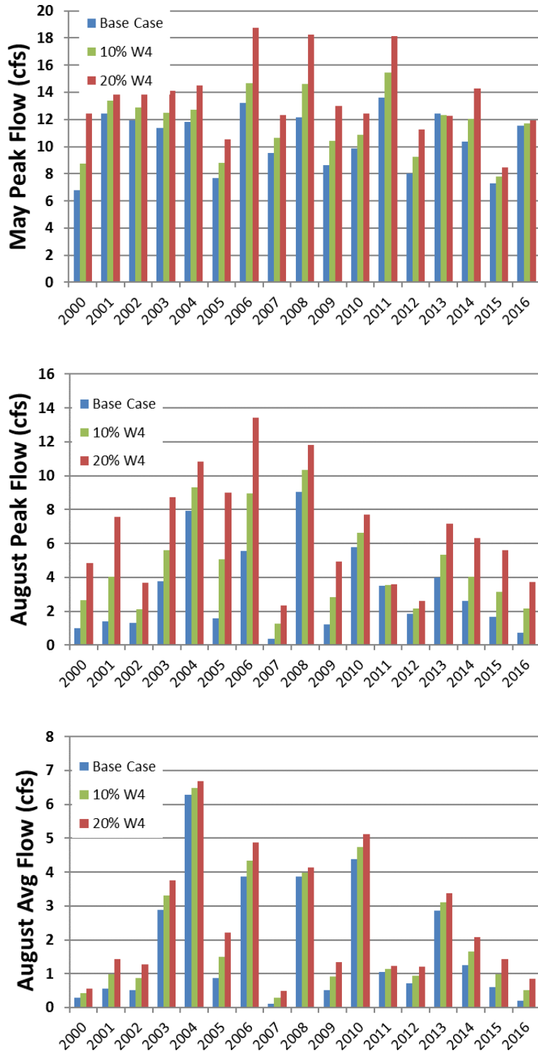
Figure 9. Simulated impact of changes in impervious surface of downstream watershed 4 on peak and average streamflow in Fish Creek.
