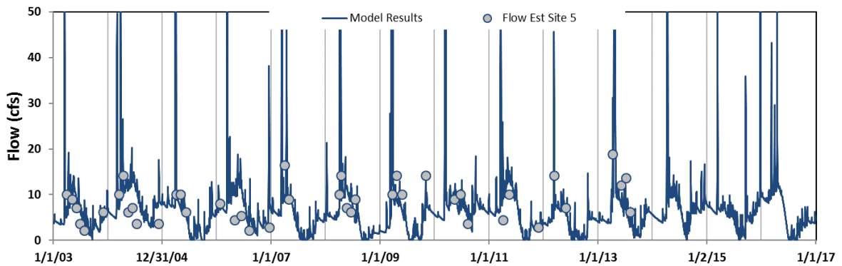
Figure 8. Simulated flow with 20% of the downstream watershed 4 as directly connected impervious area.
