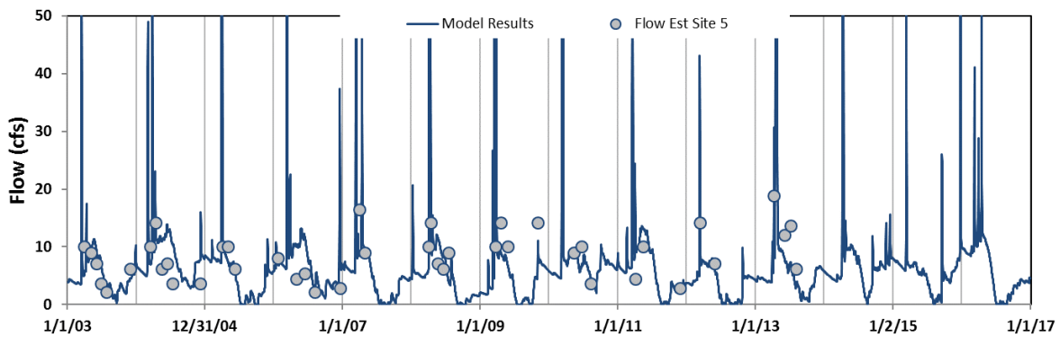
Figure 4. Comparison of estimated measured flows and model results for flow in Fish Creek at Hwy 42.
