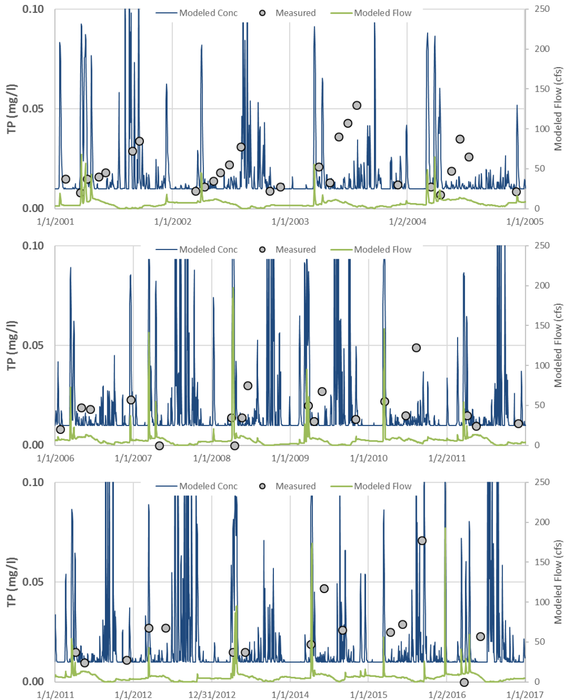
Figure 7. Comparison of measured and modeled total phosphorus concentrations in Fish Creek (left axis) shown with modeled flow (right axis).
