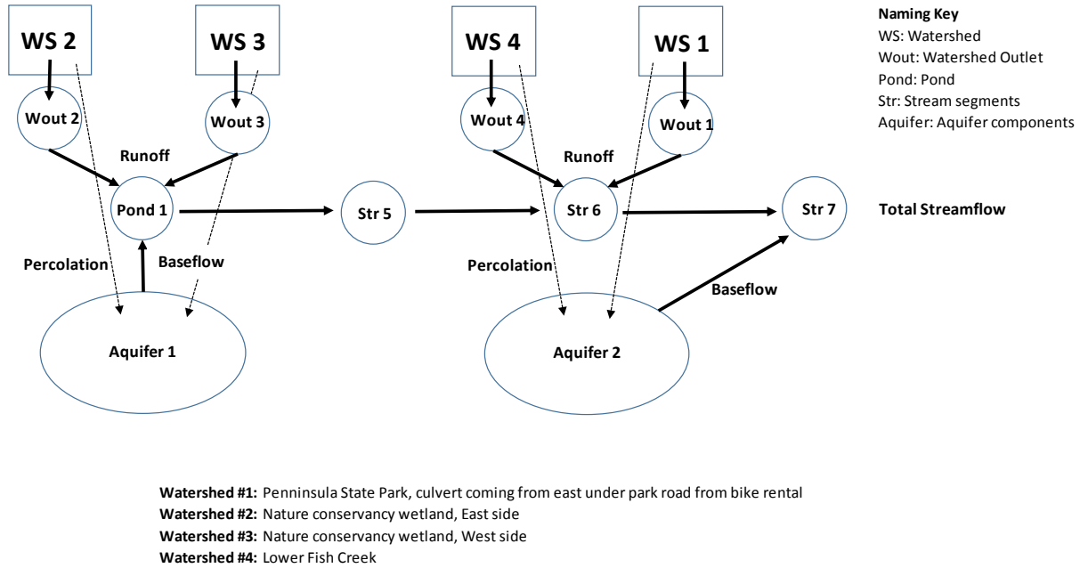
Figure 3. Schematic of the P8 model configuration for Fish Creek for streamflow at monitoring point #5. Model component types identified in the Naming Key to the right.
