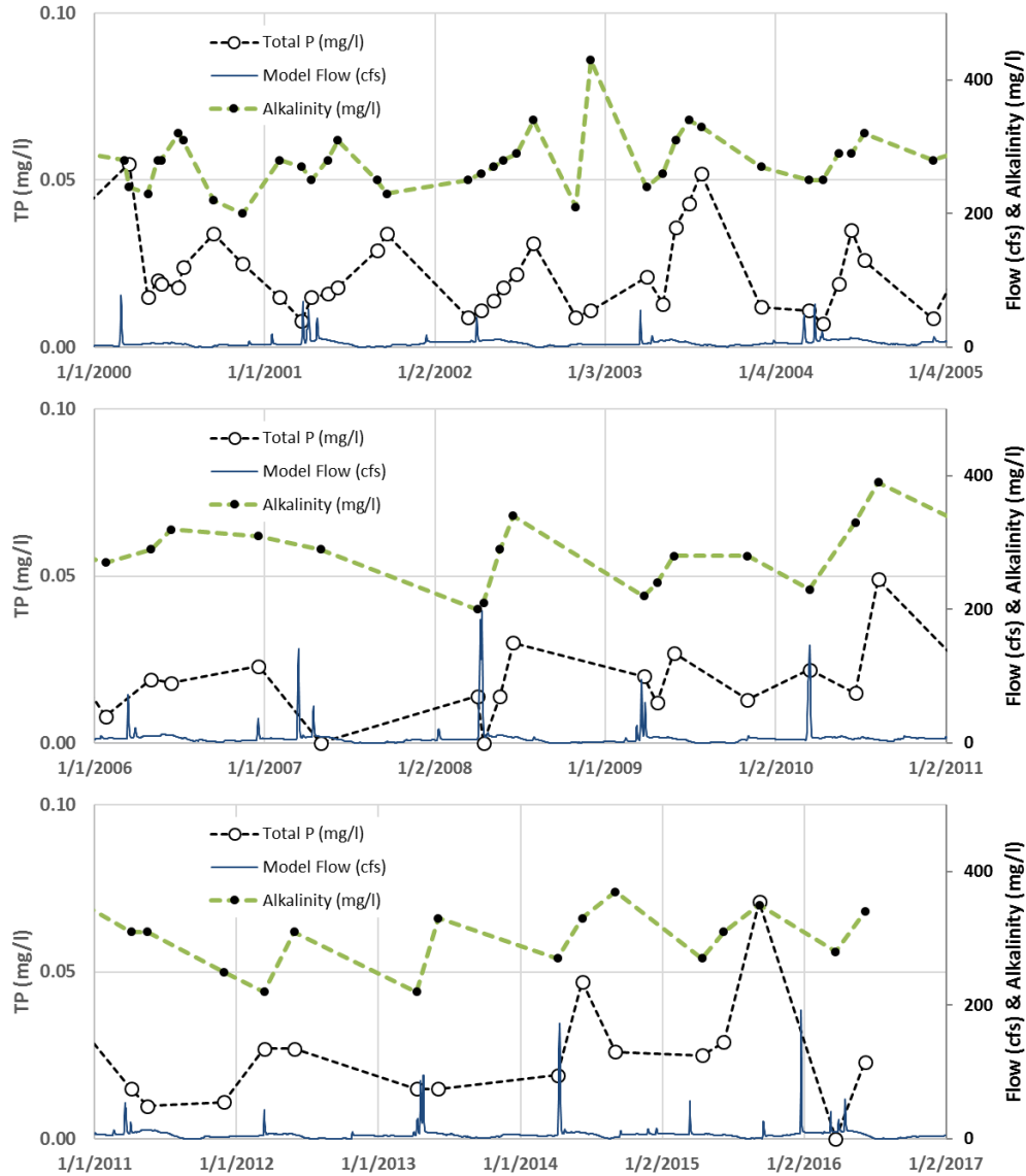
Figure 6. Measured total phosphorus concentrations over time in Fish Creek shown with measured alkalinity and simulated flow. Dotted lines added to demonstrate connection between points, and do not imply those are the concentrations between.
