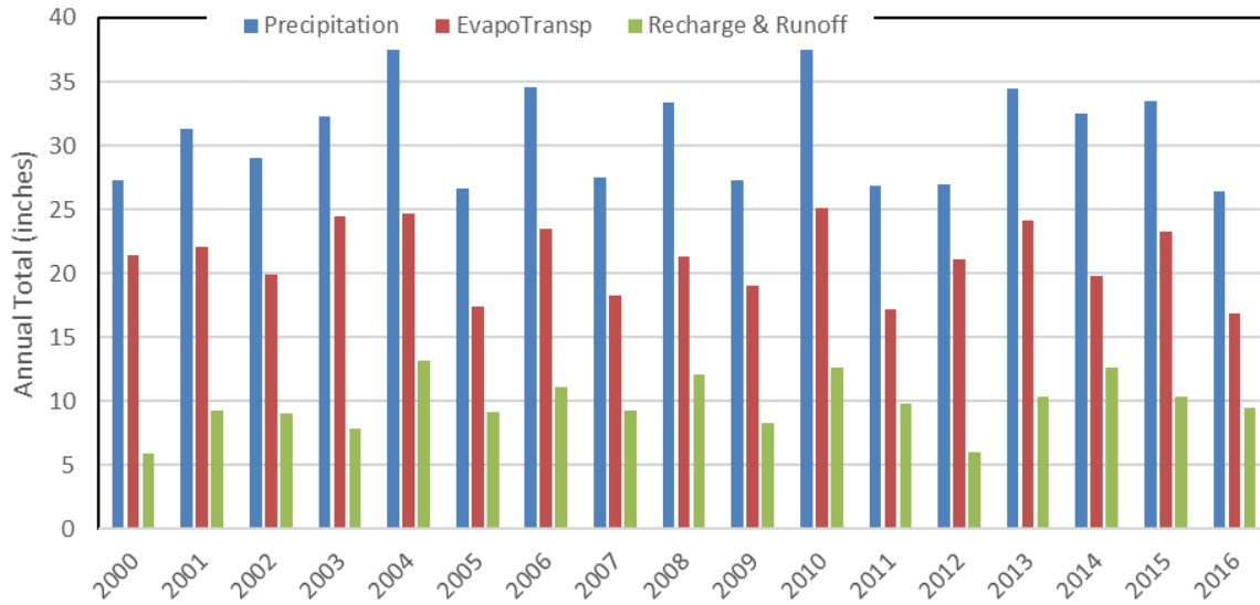
Figure 5. Simulated hydrologic budget for the Fish Creek watershed expressed as depth of water per calendar year.
