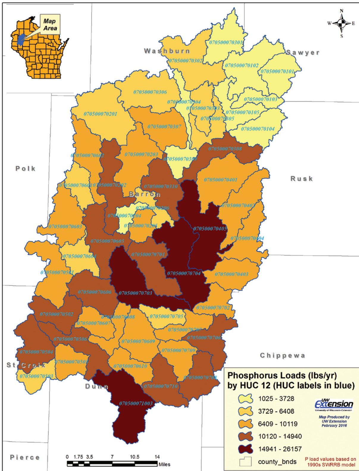
FIGURE 3.2: Red Cedar River Watershed showing HUC 12 sub-watersheds and their respective total phosphorus load estimations based on the 1990s SWRRB model
