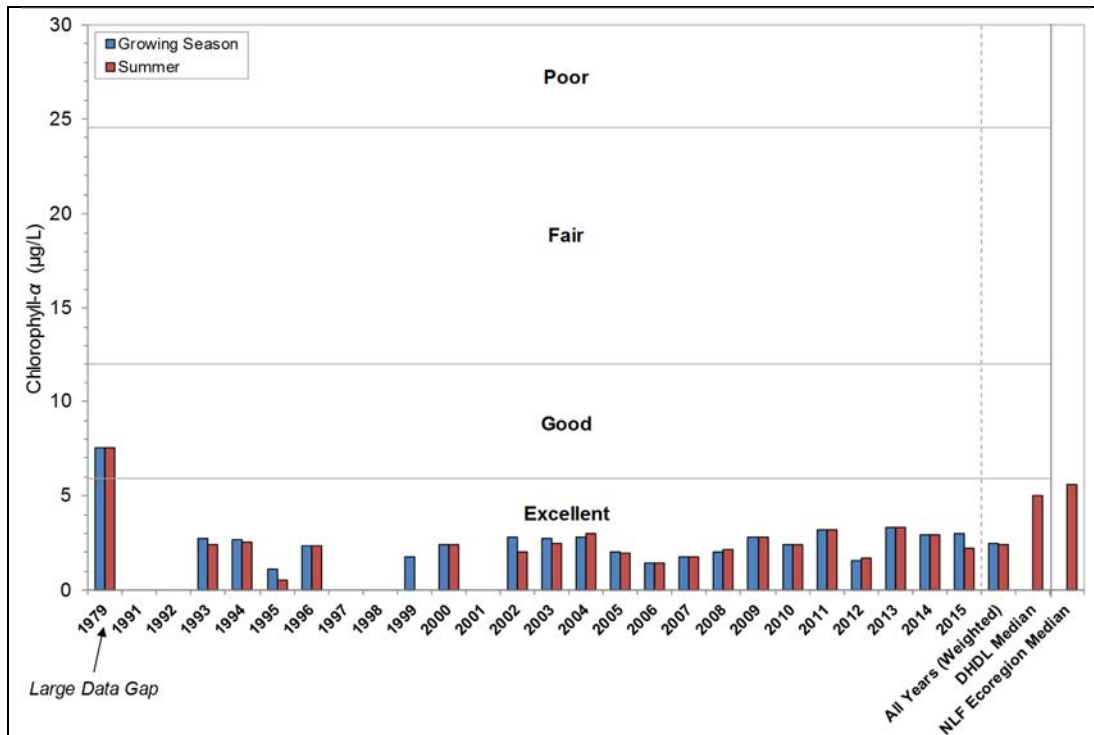
Figure 8.1.1-3. Harris Lake average annual chlorophyll- a concentrations and median chlorophyll- a concentrations for state-wide deep, headwater drainage lakes (DHDL) and Northern Lakes and Forests (NLF) ecoregion lakes. Water Quality Index values adapted from WDNR PUB WT-913.
