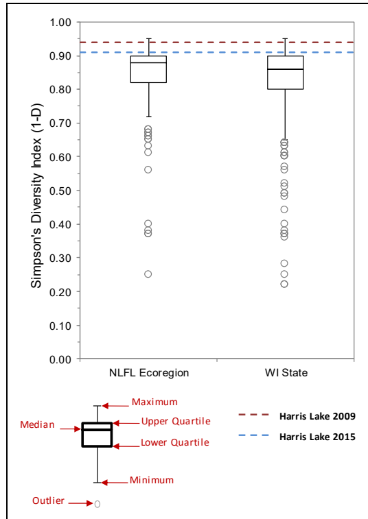
Figure 8.1.4-9. Harris Lake species diversity index. Created using data from WDNR 2009 and Onterra 2015 point-intercept surveys.
