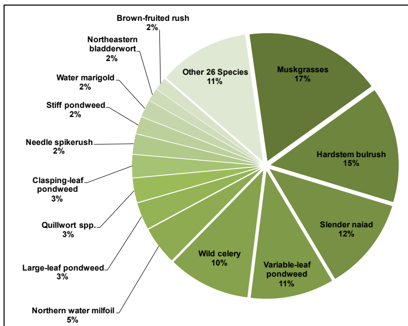
Figure 8.1.4-10. Harris Lake 2015 relative frequency of occurrence of aquatic plant species. Created using data from 2015 point-intercept survey.
