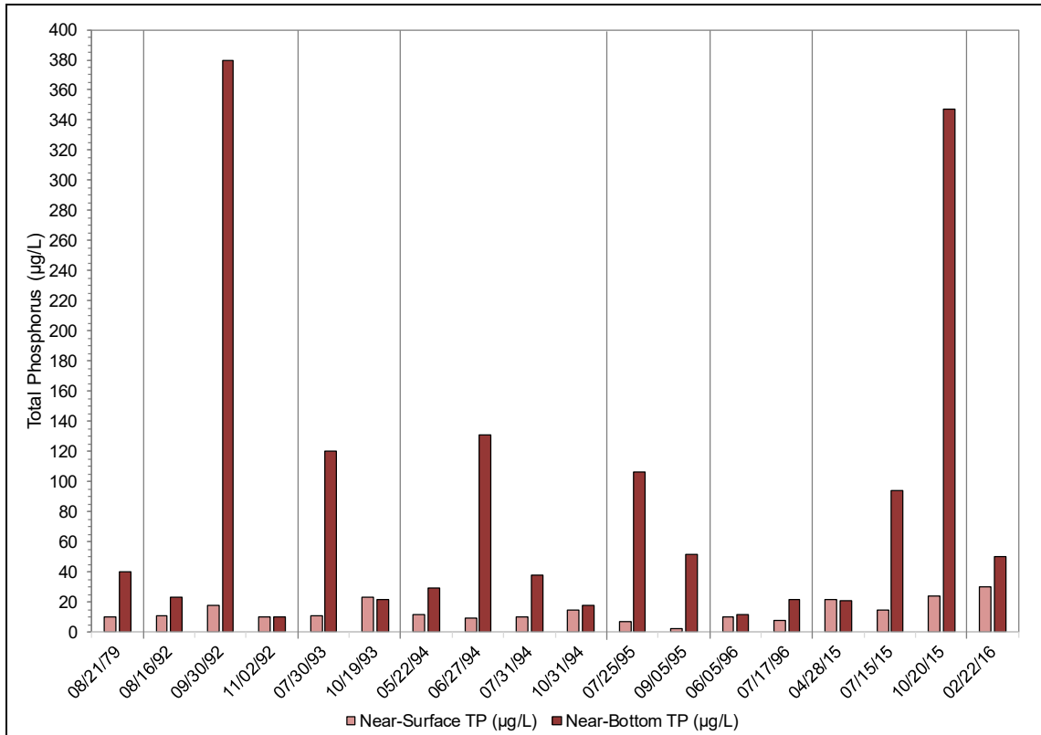
Figure 8.1.1-6. Harris Lake available near-bottom total phosphorus concentrations and corresponding near-surface total phosphorus concentrations.
