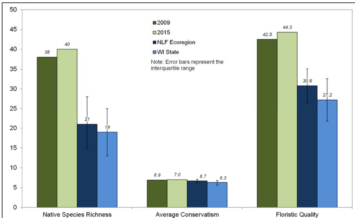
Figure 8.1.4-8. Harris Lake Floristic Quality Assessment. Created using data from WDNR 2009 and Onterra 2015 whole-lake point-intercept surveys. Analysis follows Nichols (1999).
