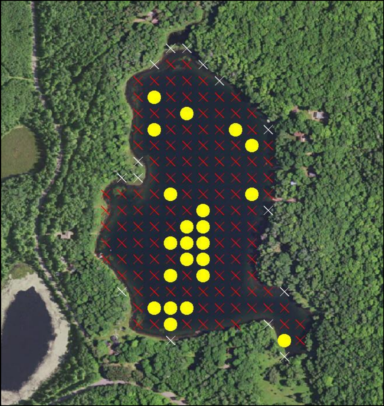
Figure 8. Distribution of plant species, Cathaline Lake (2017).
