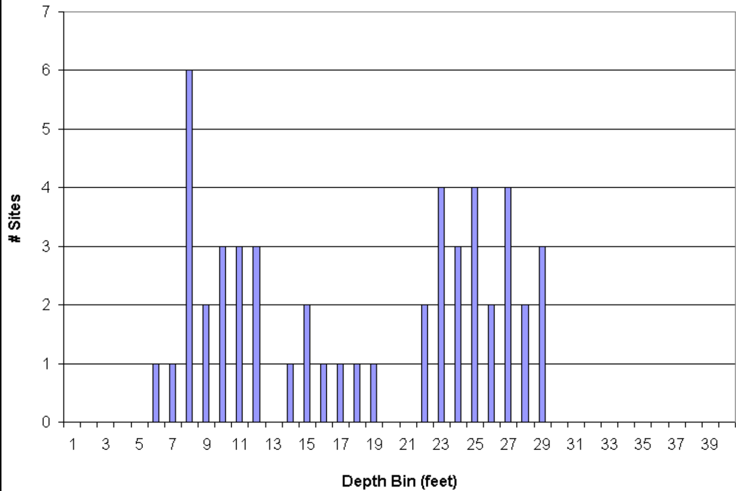
Figure 3. Maximum Depth of Plant Colonization, Cathaline Lake
