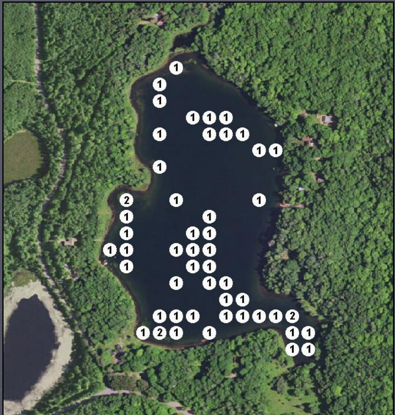
Figure 1. Number of plant species recorded at Cathaline Lake sample sites (2017).
