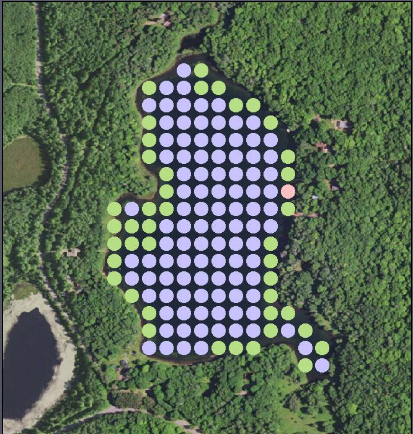
Figure 5. Cathaline Lake substrate encountered at point-intercept plant sampling sites (2017).
