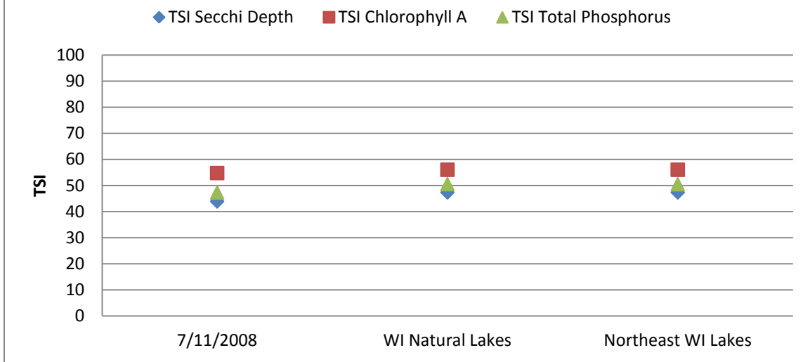
Figure 5. Cathaline Lake Trophic State Index.
