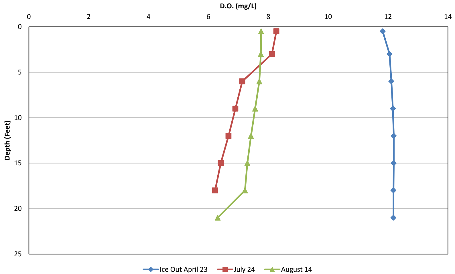
Figure 3. Pixley - FERC #2395 2019 Dissolved Oxygen Profiles
