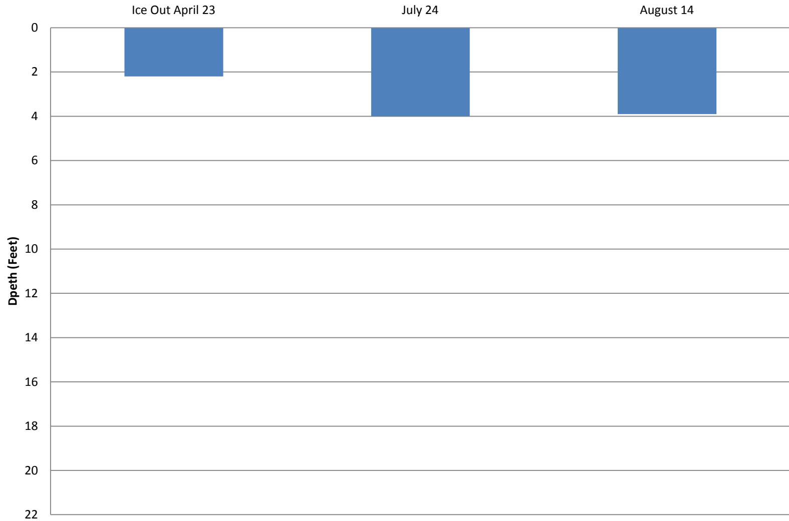
Figure 4. Flambeau Pixley - FERC# 2395 Secchi Depths 2019
