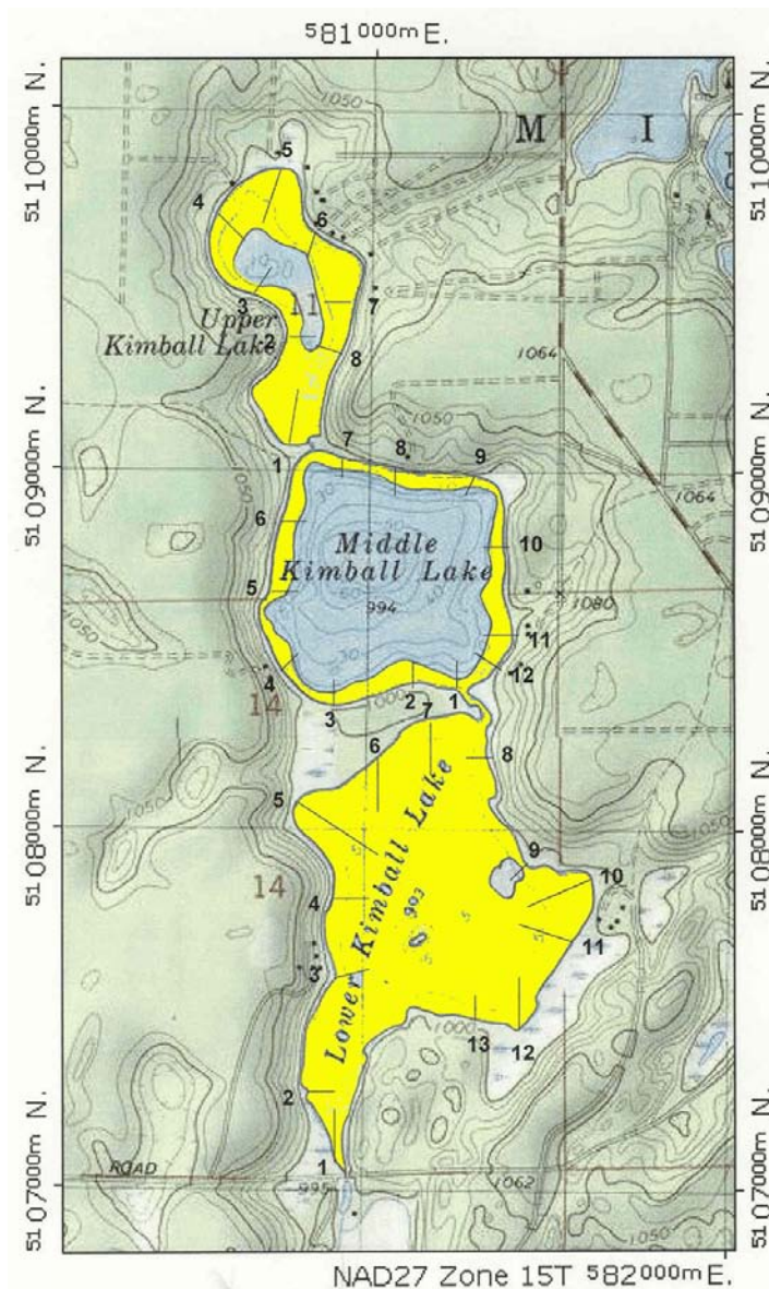
Figure 17. Aquatic plant coverage in the Kimball Lake on July and August, 2004 is shown in yellow.
