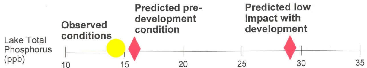
Figure 21. Predicted lake phosphorus concentrations based on modeling are shown with red diamonds. Actual lake phosphorus concentrations are shown with the solid circles.
