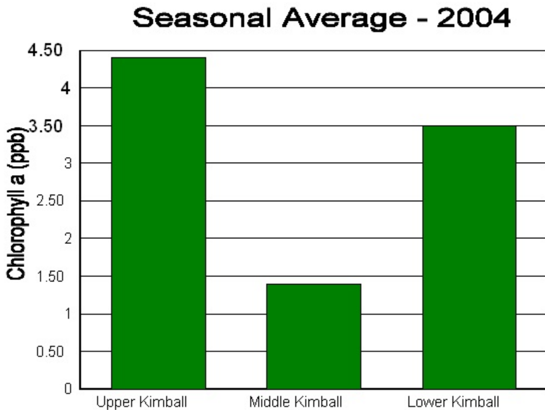
Figure 14. Seasonal average chlorophyll concentrations for Kimball Lakes in 2004.
