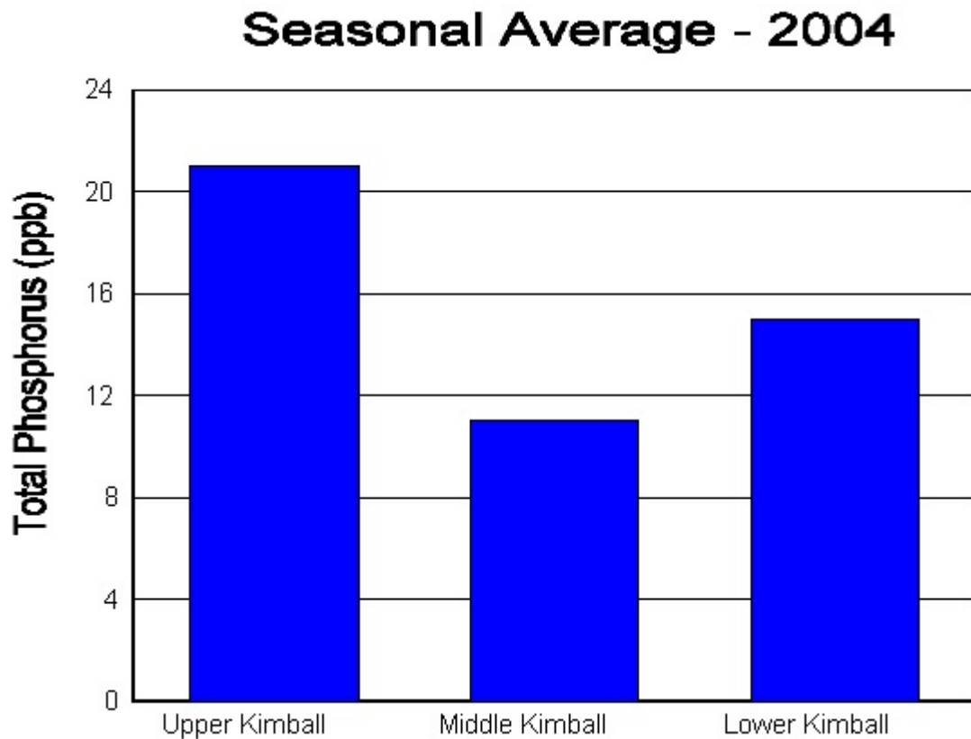
Figure 13. Seasonal average total phosphorus for Kimball Lakes in 2004.
