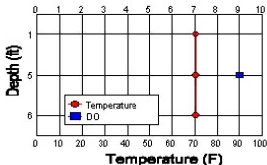
Figure 11. Dissolved oxygen (DO)/temperature profiles for June 21, 2004. Dissolved oxygen data are shown with squares and temperature with circles.
