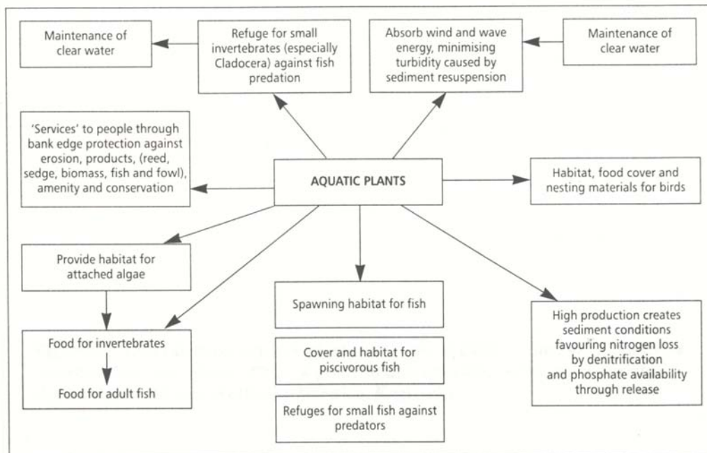
Figure 26. Links between aquatic plants and other organisms, including ourselves (source: Moss and others. 1996. A guide to the restoration of nutrient-enriched shallow lakes. Broads Authority Norwich, England).
