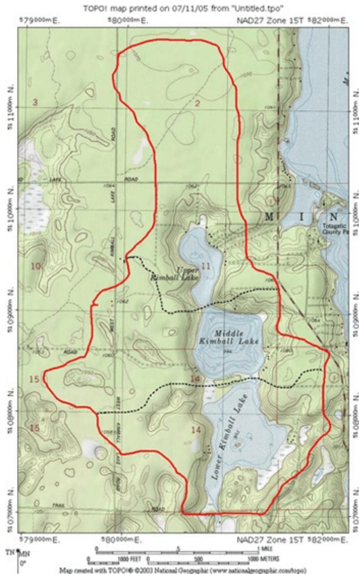
Figure 4. Drainage area to all three of the Kimball Lakes is 1,314 acres (does not include lake area).
