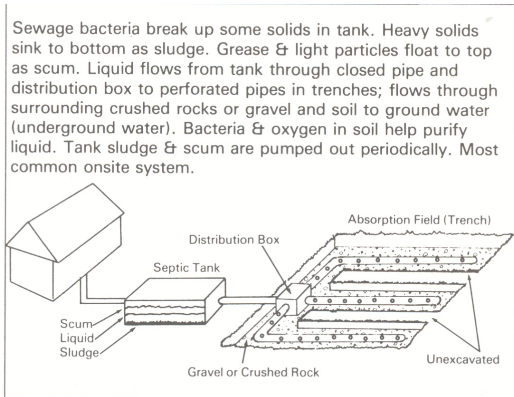
Figure 8. Typical onsite wastewater treatment system found in the Kimball Lakes watershed.
