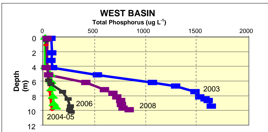
Figure 16. Phosphorus profiles in both basins showing the effectiveness of the alum treatment. The alum treatment was very effective at reducing P concentrations in the bottom waters until the flooding in 2008.
