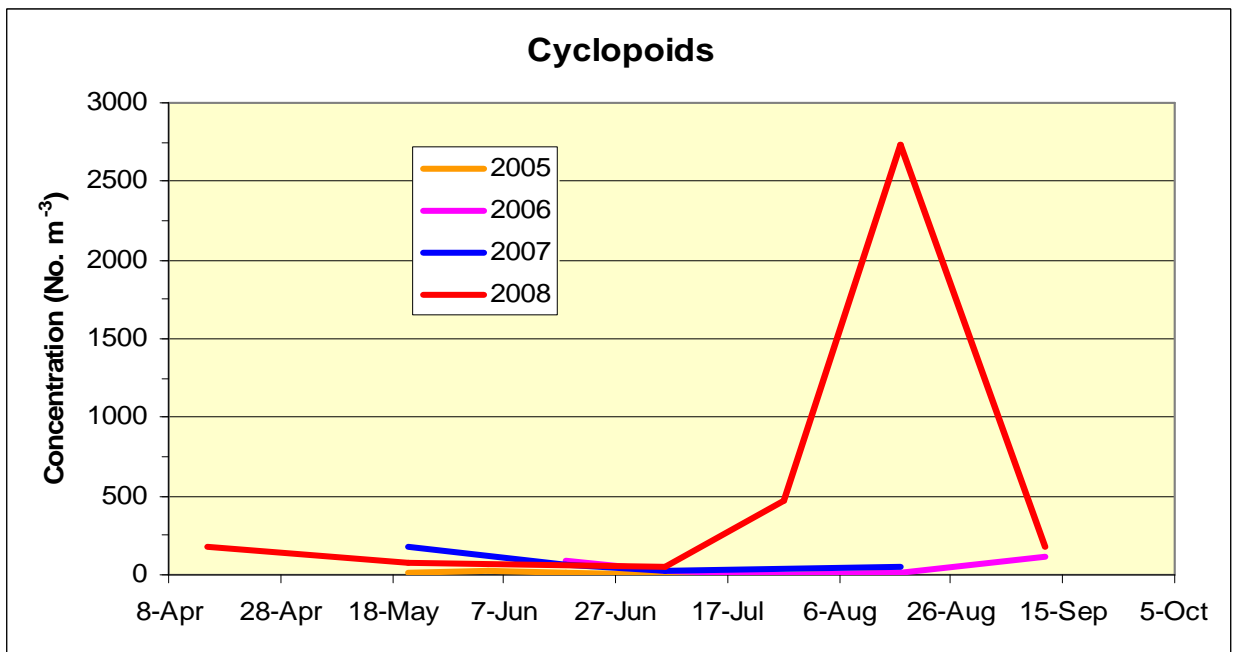
Figure 20. Copepods in Silver Lake after the completion of the restoration steps. The increased levels of the herbivorous Calanoids in the 2006 and 2007 are considered good they help reduce the amount of algae. Although the cyclopoid that was dominant following the flood in 2008 is herbivorous, Tropocyclops prasinus are small in size and thus do not consume large amounts of algae.
