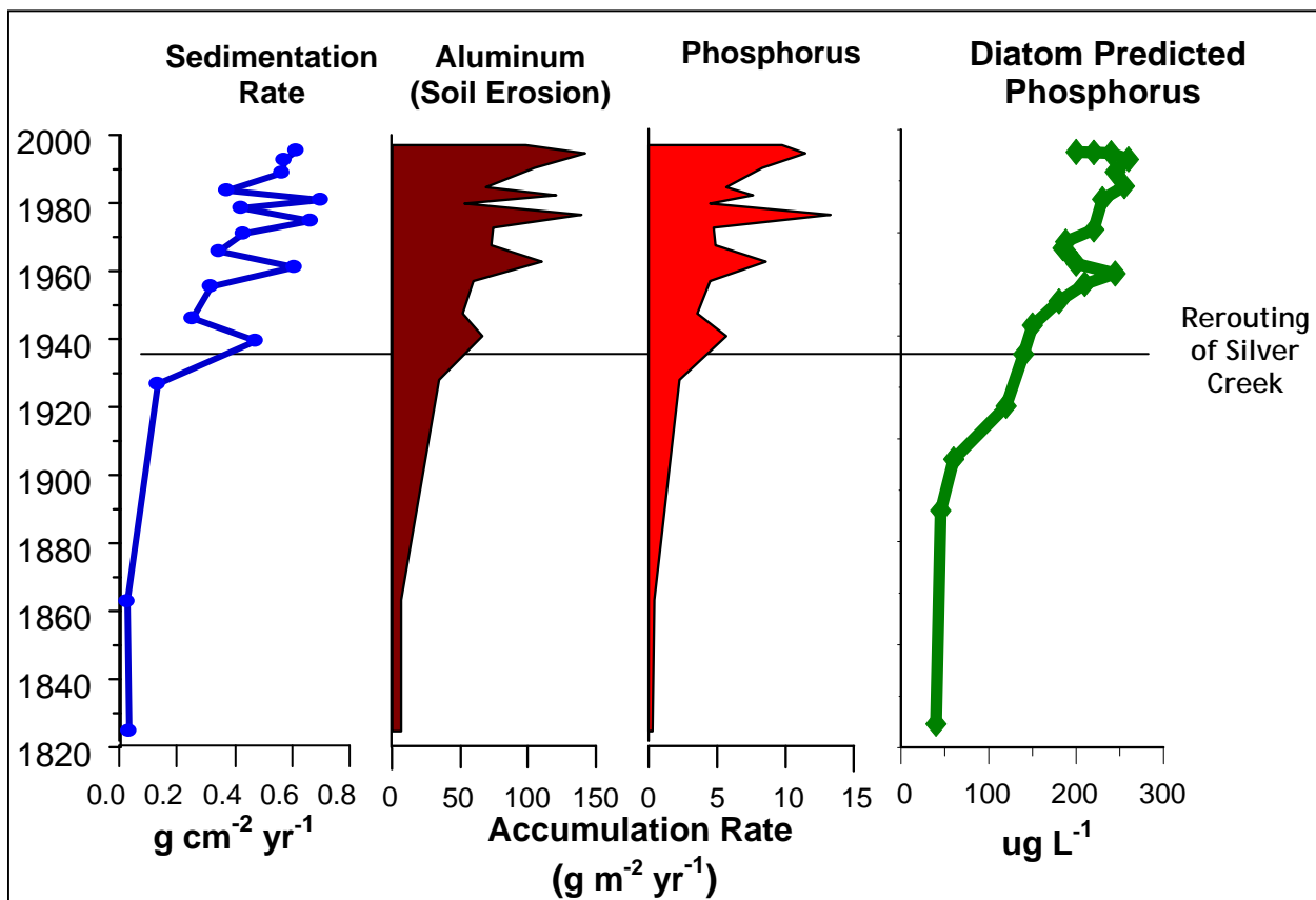
Figure 5. Results from sediment core collected in the East Basin showing the adverse impact of rerouting Silver Creek into the lake in 1936. This resulted in a large increase in sediment and phosphorus entering the lake.
