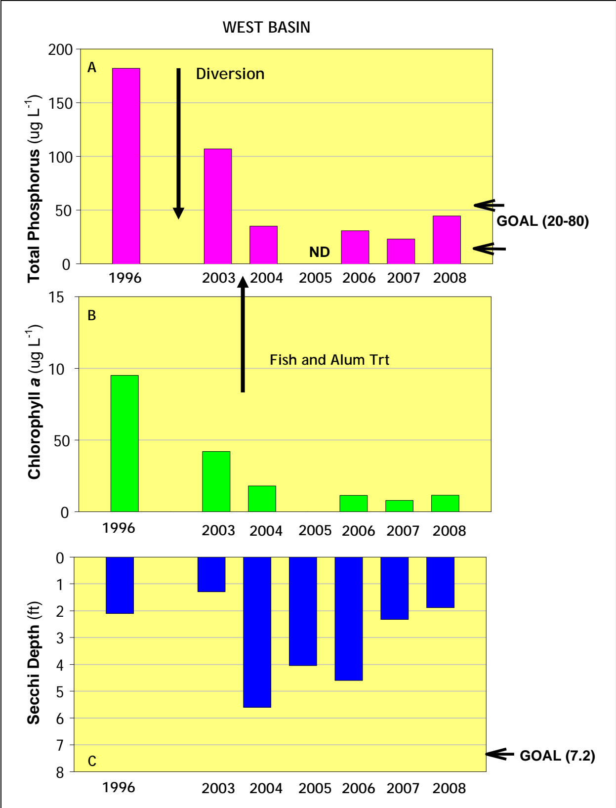
Figure 14. Summer mean values for the trophic variables in the West Basin. Phosphorus concentrations meet the project goals while water clarity has not met the goal.
