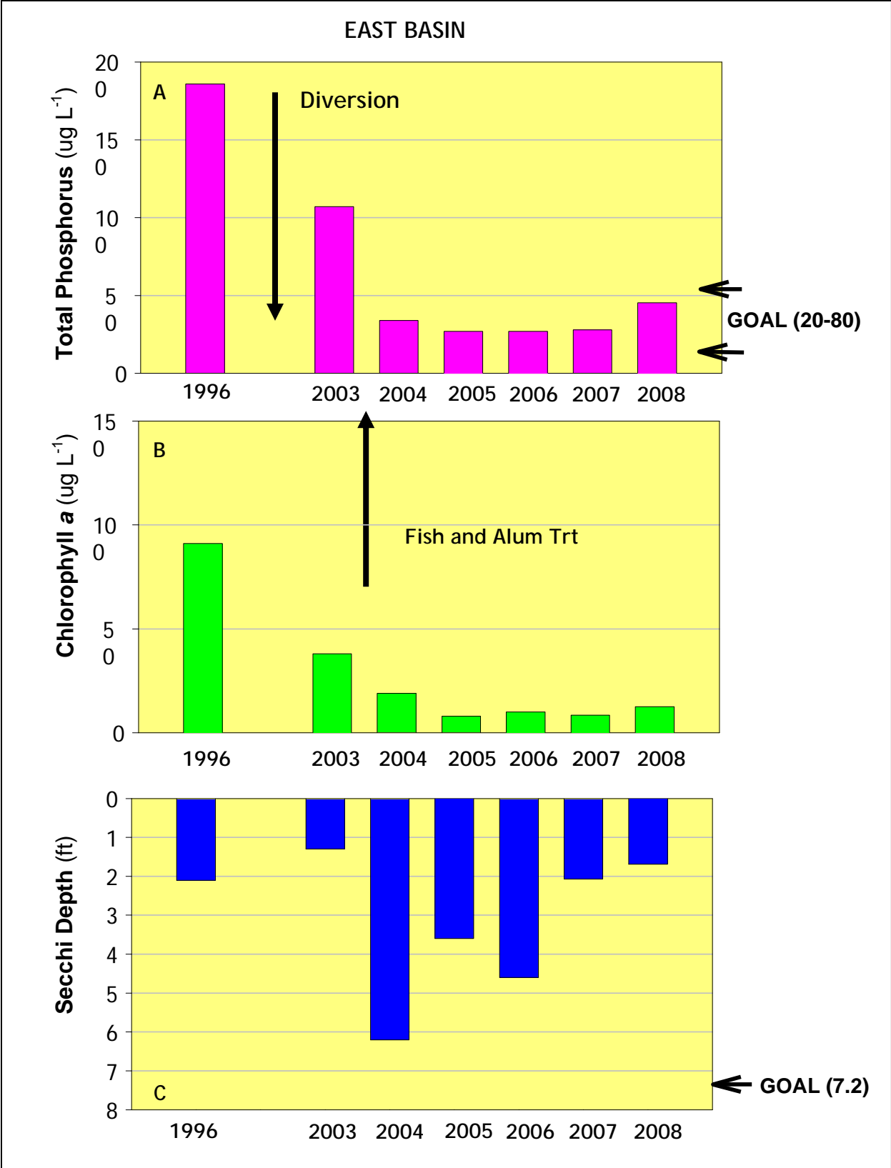
Figure 13. Summer mean values for the trophic variables in the East Basin. Phosphorus concentrations meet the project goals while water clarity has not met the goal.
