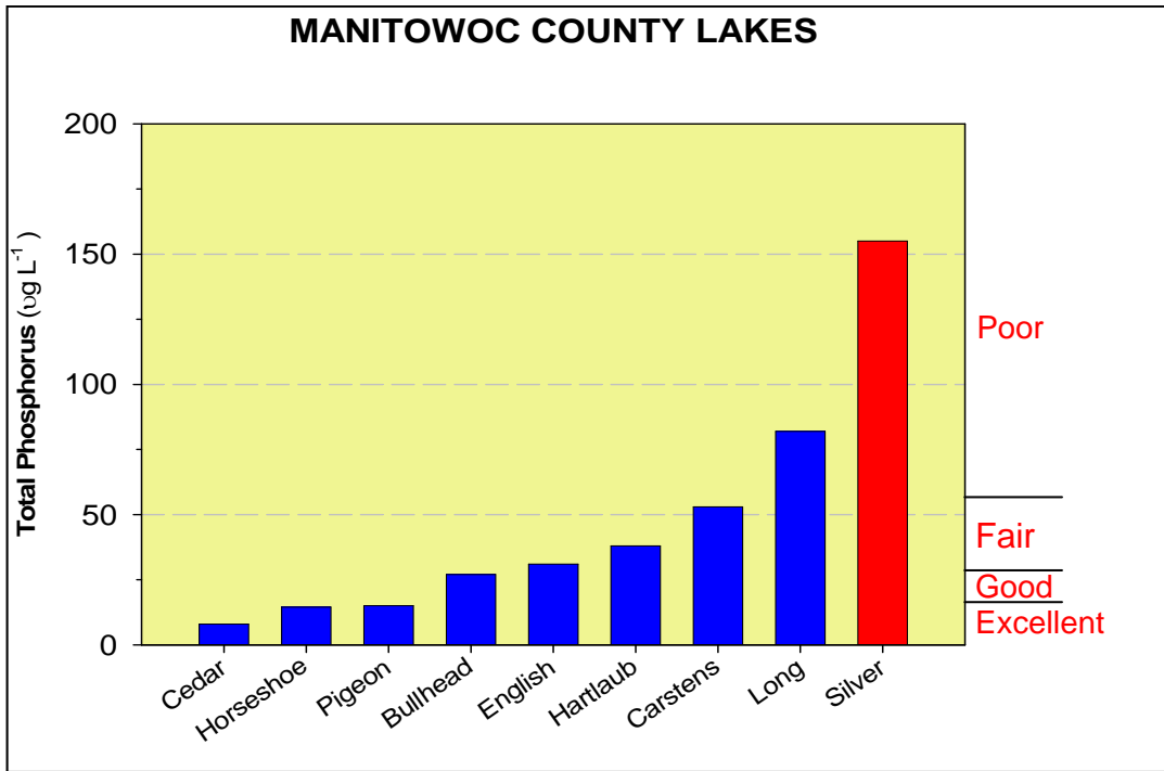
Figure 3. A comparison of phosphorus values in Silver Lake to concentrations in other Manitowoc lakes during the 1990s. Phosphorus levels in Silver Lake placed the lake in the poor category.
