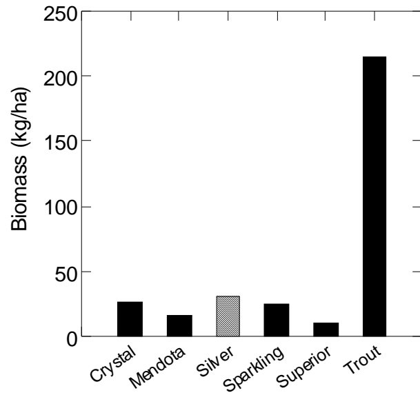
Figure 5. The biomass density estimated using hydroacoustics in various lakes. The hatched bar indicates Silver Lake.
