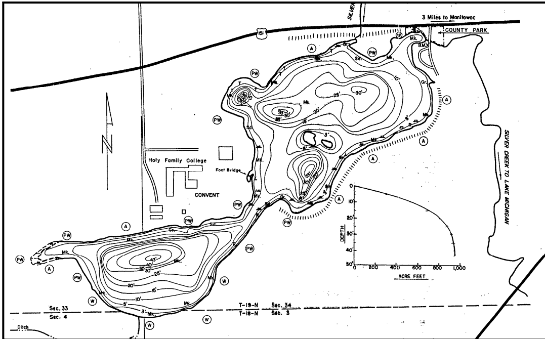
Figure 1. Morphometric map of Silver Lake showing where Silver Creek entered the lake prior to the partial diversion in the mid-1990s. The partial diversion directed the inlet towards to the outlet. (See Figure 7 for more detail.)
