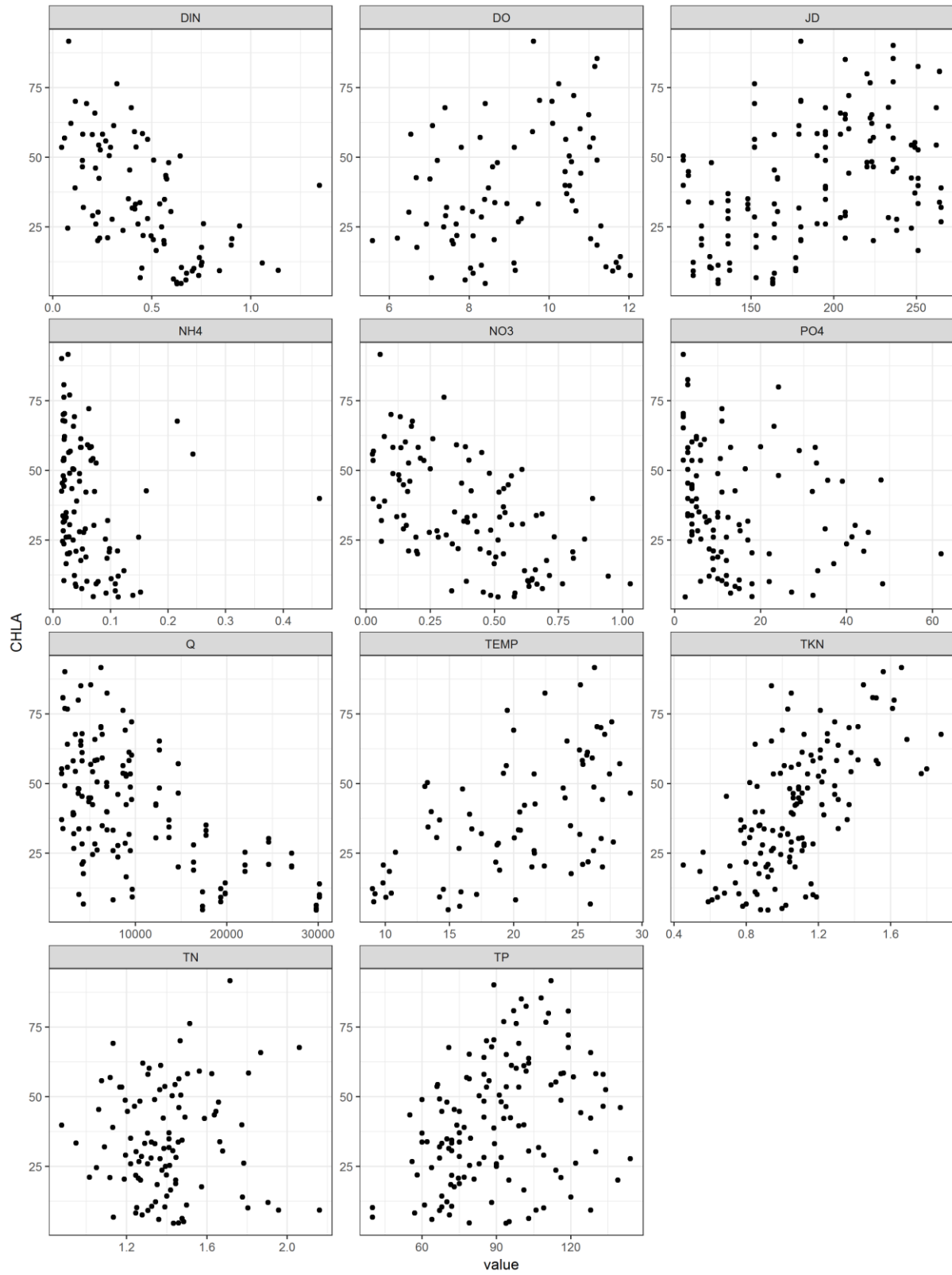
Figure 4. Scatter plots of chlorophyll a versus other parameters in Lake Wisconsin, 2010-13.
