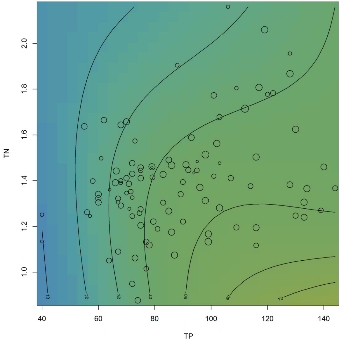
Figure 11. Contour plot of estimated CHL concentration ( \mu\text{g/L} ) as a function of TP ( \mu\text{g/L} ) and TN ( \text{mg/L} ) in Lake Wisconsin from Model #3 (Table 6). Circles are observations (diameter proportional to \log(\text{CHL}) concentration).
