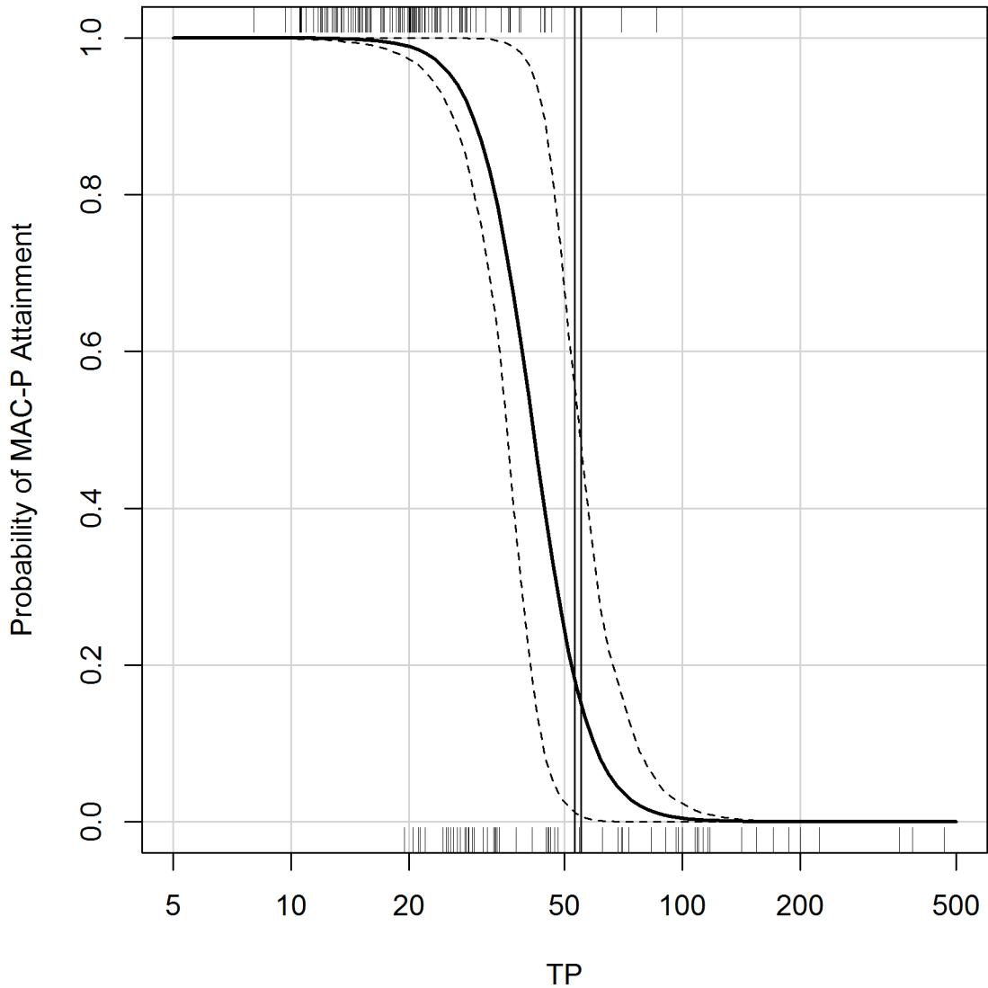
Figure 25. Regression relationship between TP and probability of MAC-P attainment for southern Wisconsin drainage lakes and reservoirs. Dashed lines are 90% confidence interval. The “rugs” of tick marks on the top and bottom of the plot are the TP values where the MAC-P threshold was attained and not attained, respectively. Vertical lines at 55 and 53 \mu\text{g/L} TP are expected geometric mean TP in Castle Rock and Petenwell Lakes, respectively, when recreational criteria are met. Note log TP scale.
