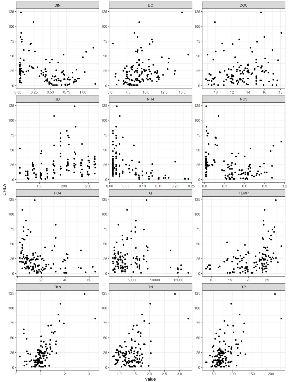
Figure 3. Scatter plots of chlorophyll a versus other parameters in Castle Rock Lake, 2010-13.
