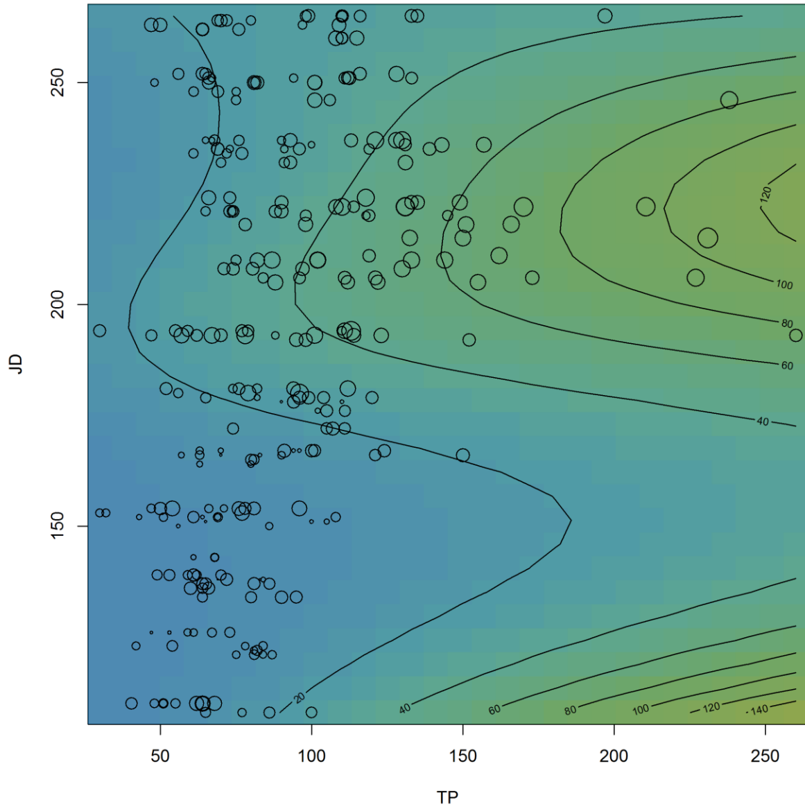
Figure 7. Contour plot of estimated CHL concentration ( \mu\text{g/L} ) as a function of TP ( \mu\text{g/L} ) and JD in Petenwell/Castle Rock Lakes from Model #1 (Table 5). Circles are observations (diameter proportional to \log(\text{CHL}) concentration).
