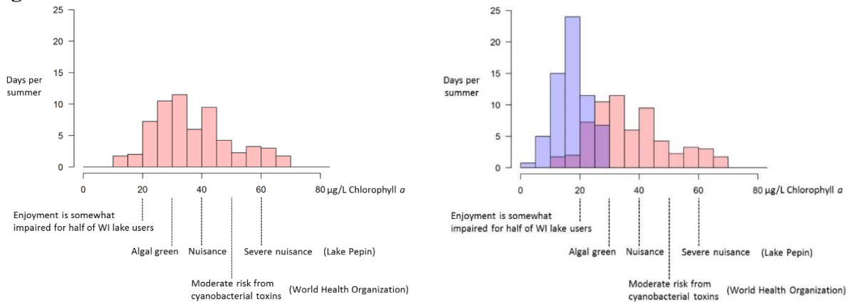
Figure 1. CHL-a under current conditions and recommended SSC
