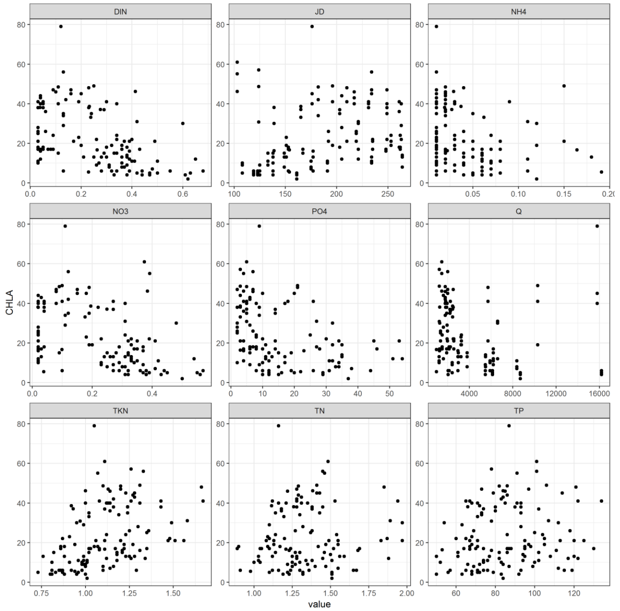
Figure 5. Scatter plots of chlorophyll a versus other parameters in Lake Du Bay, 2010-13.
