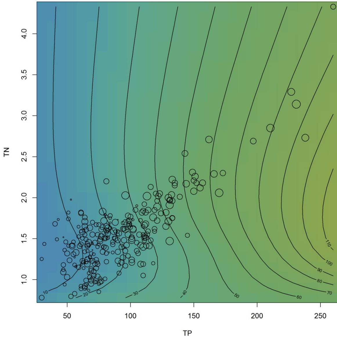
Figure 9. Contour plot of estimated CHL concentration ( \mu\text{g/L} ) as a function of TP ( \mu\text{g/L} ) and TN (mg/L) in Petenwell/Castle Rock Lakes from Model #6 (Table 5). Circles are observations (diameter proportional to \log(\text{CHL}) concentration).
