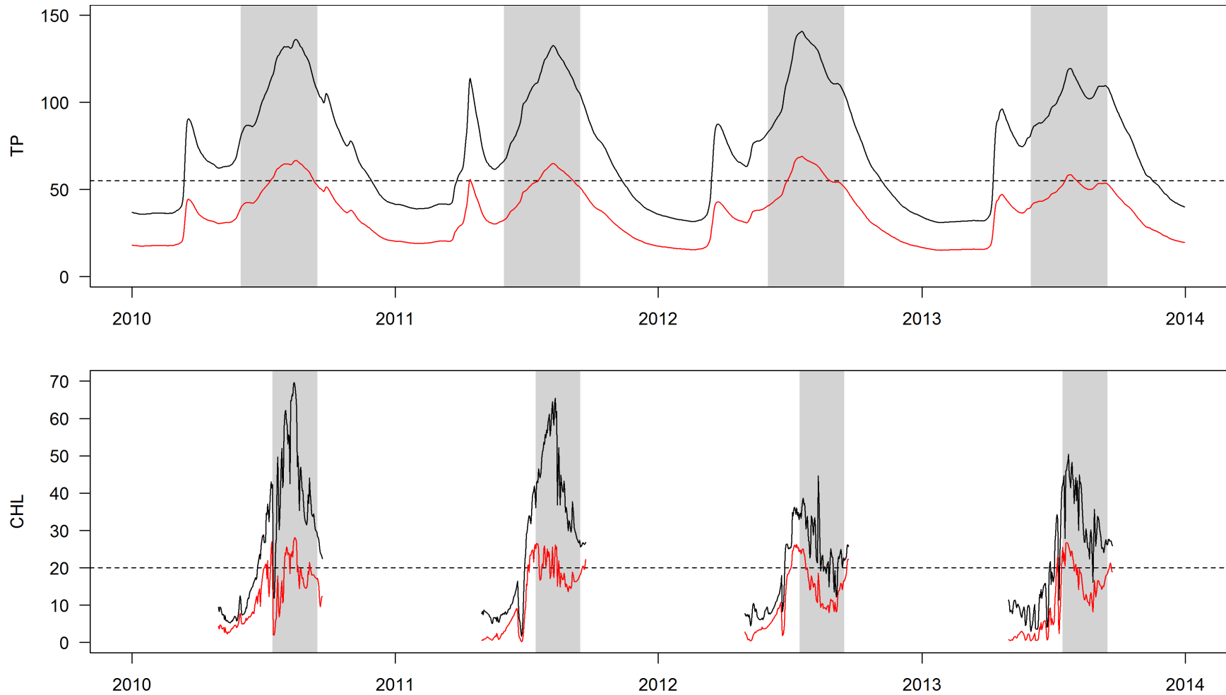
Figure 21. Current condition (black) and site-specific criterion (red) scenarios for total phosphorus (TP; \mu\text{g/L} ) and chlorophyll a (CHL; \mu\text{g/L} ) in Petenwell Lake. Dashed lines are recommended TP site-specific criteria (53 \mu\text{g/L} ) and recreational chlorophyll a target (70 th percentile = 20 \mu\text{g/L} ). Shaded areas are assessment periods for each parameter.
