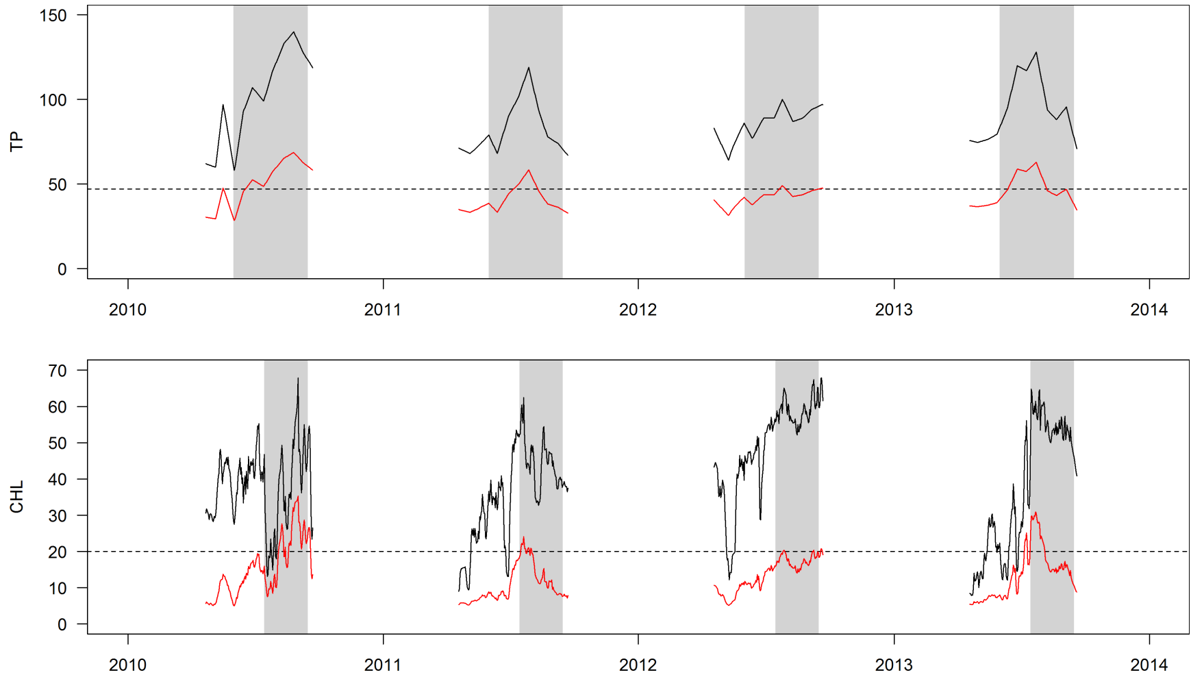
Figure 23. Current condition (black) and site-specific criterion (red) for total phosphorus (TP; \mu\text{g/L} ) and chlorophyll a (CHL; \mu\text{g/L} ) in Lake Wisconsin. Dashed lines are recommended TP site-specific criteria ( 47 \mu\text{g/L} ) and recreational chlorophyll a target ( 70^{\text{th}} percentile = 20 \mu\text{g/L} ). Shaded areas are assessment periods for each parameter.
