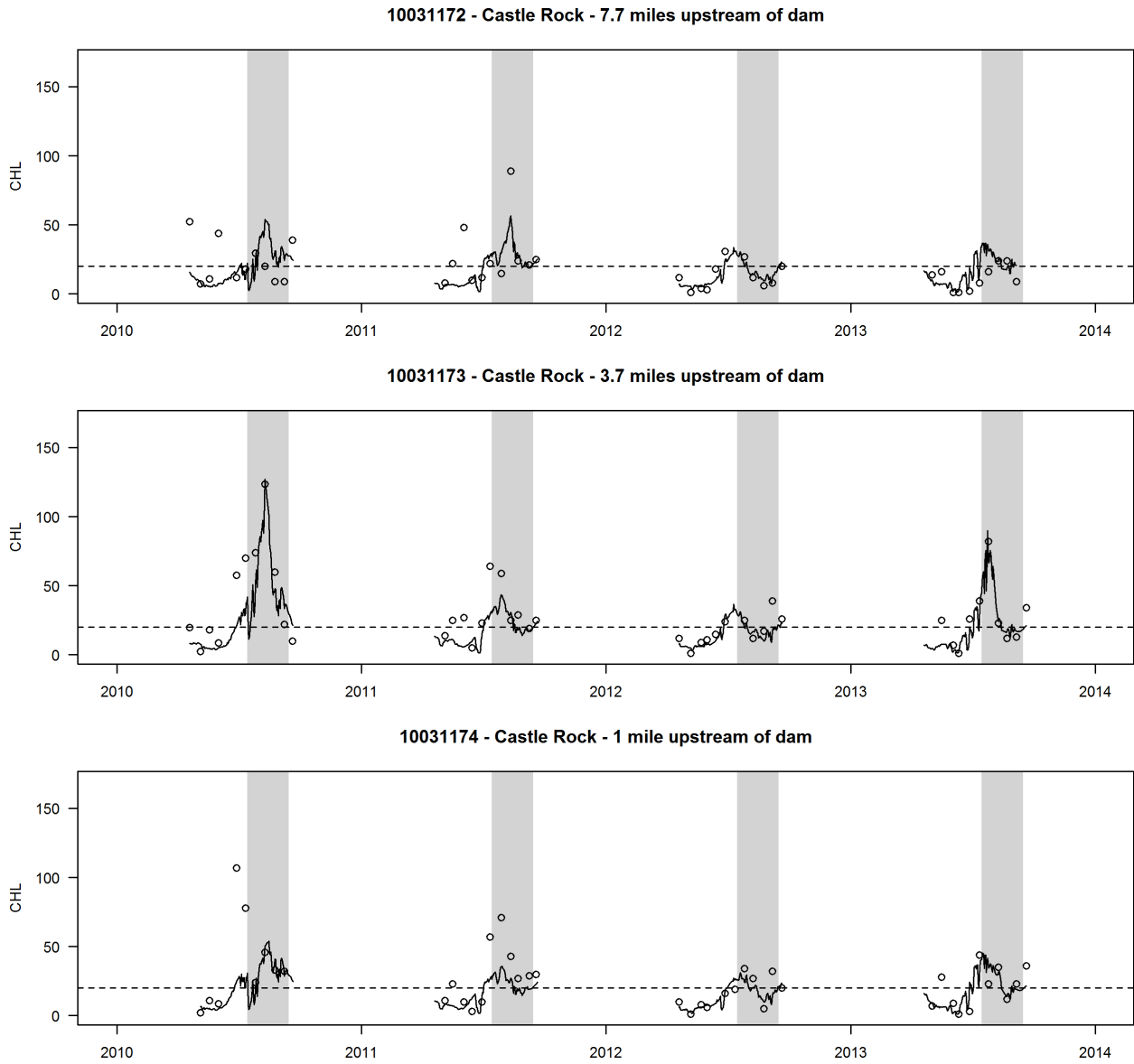
Figure 19. Observed (circles) and simulated (lines) chlorophyll a ( \mu\text{g/L} ) in Castle Rock Lake. Dashed line is recreational chlorophyll a target ( 20 \mu\text{g/L} ). Shaded areas are chlorophyll a assessment periods.
