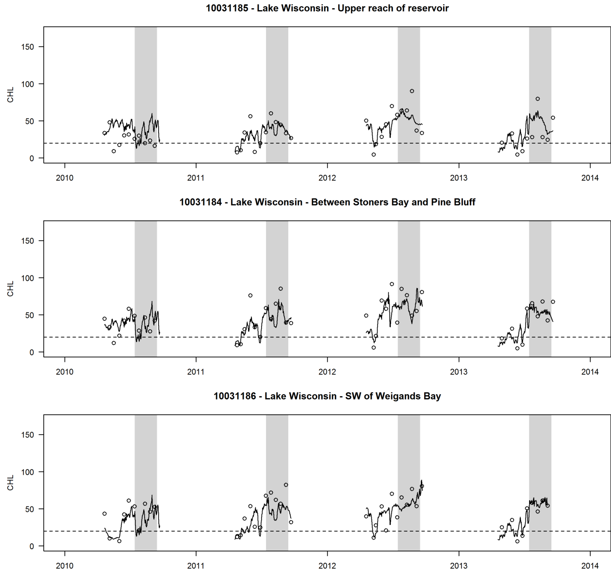
Figure 20. Observed (circles) and simulated (lines) chlorophyll a ( \mu\text{g/L} ) in Lake Wisconsin. Dashed line is recreational chlorophyll a target ( 20 \mu\text{g/L} ). Shaded areas are chlorophyll a assessment periods.
