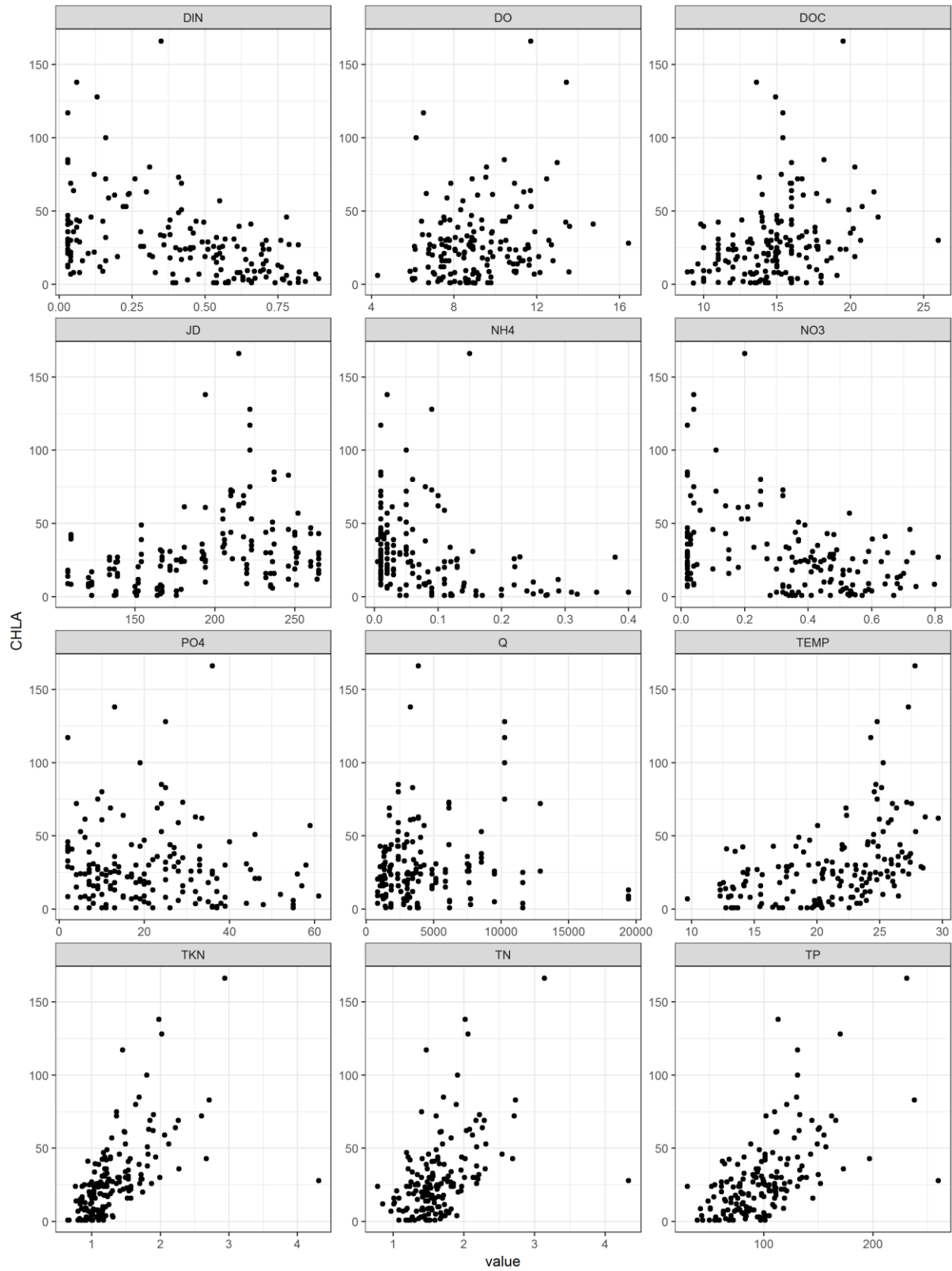
Figure 2. Scatter plots of chlorophyll a versus other parameters in Petenwell Lake, 2010-13.
