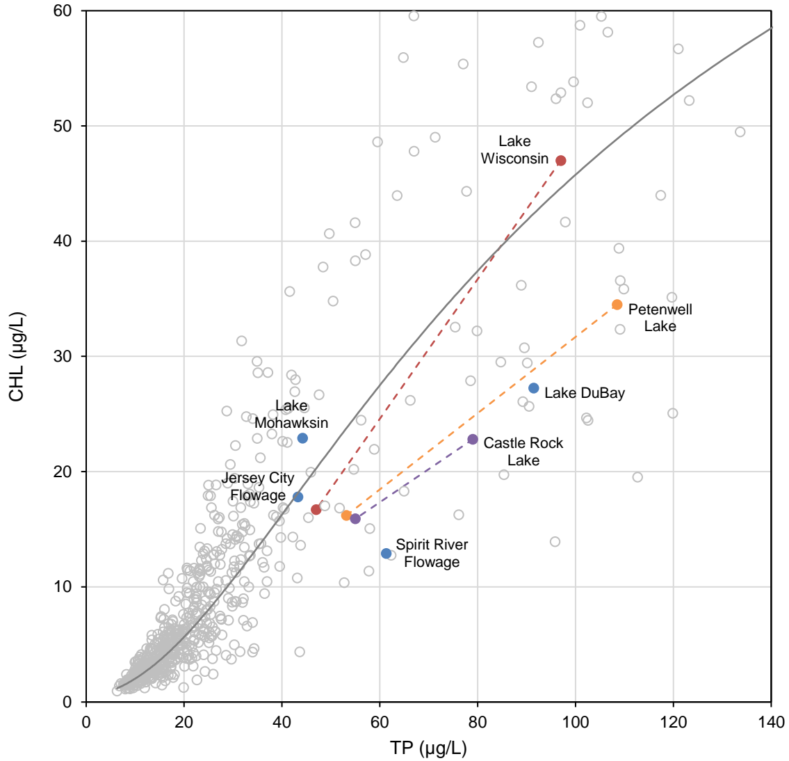
Figure 24. TP:CHL relationships for Wisconsin River reservoirs. All TP and CHL values are geometric mean values for assessment periods. Blue circles are reservoirs upstream of Petenwell Lake. Circles and dashed lines for Petenwell, Castle Rock, and Lake Wisconsin represent current conditions (high TP/CHL) and SSC conditions (low TP/CHL). Gray circles are all other Wisconsin lakes and reservoirs that had at least six concurrent TP and CHL samples. Gray line is a 3 rd -order polynomial regression fit to the log(CHL)~log(CHL) relationship for the gray circles.
