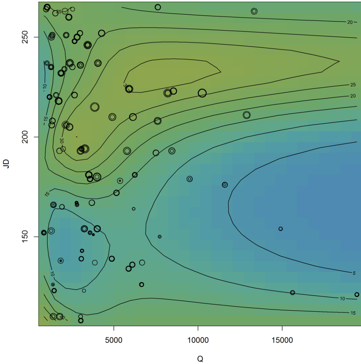
Figure 8. Contour plot of estimated CHL concentration ( \mu\text{g/L} ) as a function of Q (cfs) and JD in Petenwell/Castle Rock Lakes from Model #1 (Table 5). Circles are observations (diameter proportional to \log(\text{CHL}) concentration).
