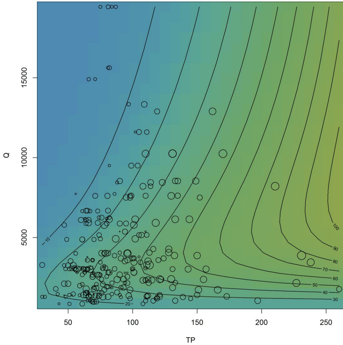
Figure 6. Contour plot of estimated CHL concentration ( \mu\text{g/L} ) as a function of TP ( \mu\text{g/L} ) and Q (cfs) in Petenwell/Castle Rock Lakes from Model #1 (Table 5). Circles are observations (diameter proportional to \log(\text{CHL}) concentration).
