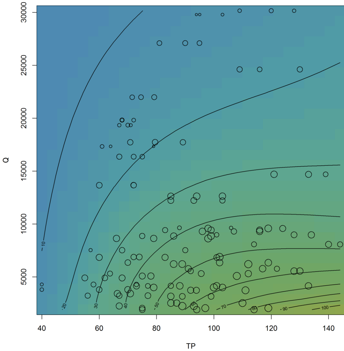
Figure 10. Contour plot of estimated CHL concentration ( \mu\text{g/L} ) as a function of TP ( \mu\text{g/L} ) and Q (cfs) in Lake Wisconsin from Model #2 (Table 6). Circles are observations (diameter proportional to \log(\text{CHL}) concentration).
