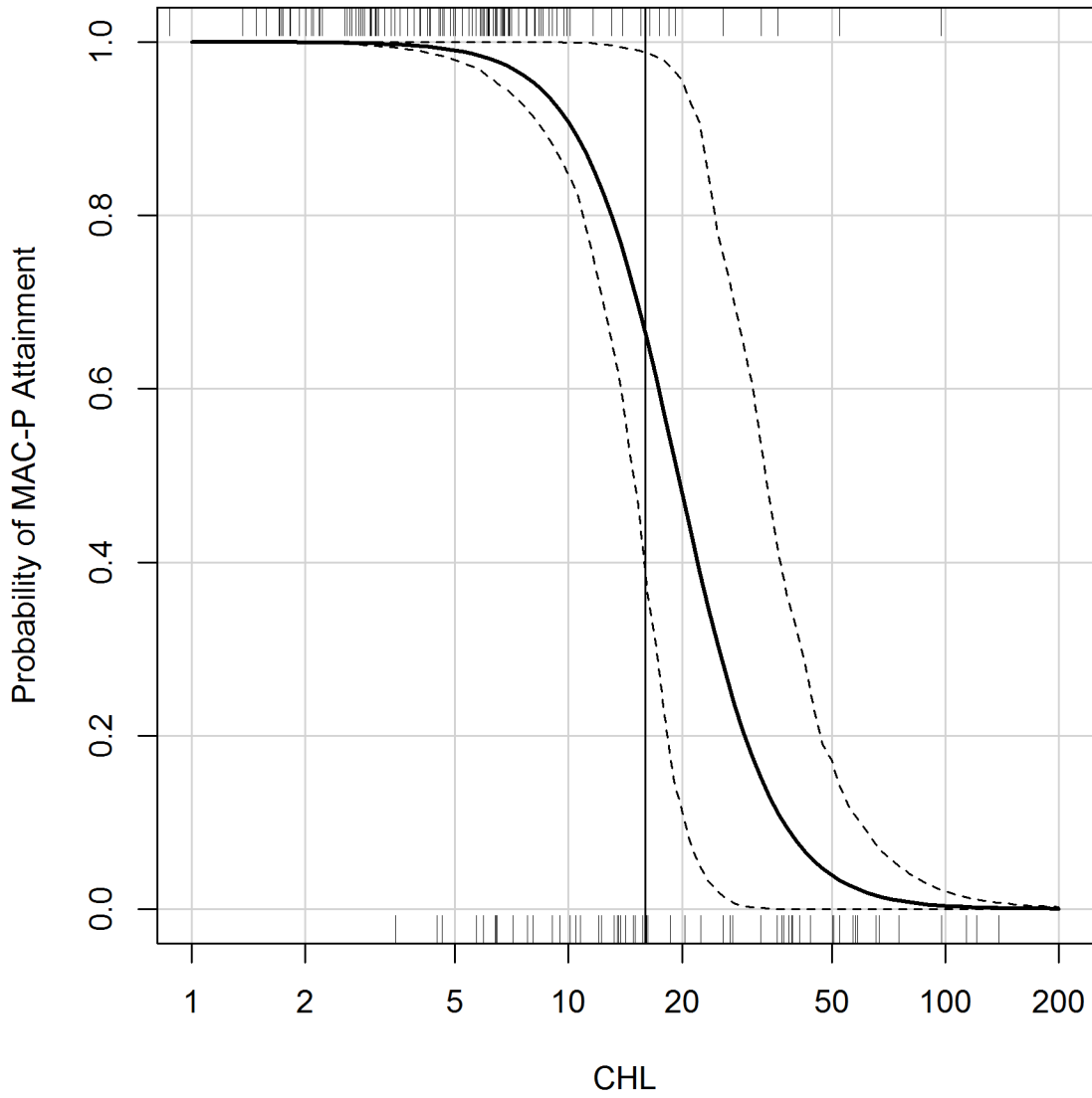
Figure 26. Regression relationship between CHL and probability of MAC-P attainment for southern Wisconsin drainage lakes and reservoirs. Dashed lines are 90% confidence interval. The “rugs” of tick marks on the top and bottom of the plot are the CHL values where the MAC-P threshold was attained and not attained, respectively. Vertical line at 16 \mu\text{g/L} CHL is expected geometric mean CHL in Castle Rock and Petenwell Lakes when recreational criteria are met. Note log CHL scale.
