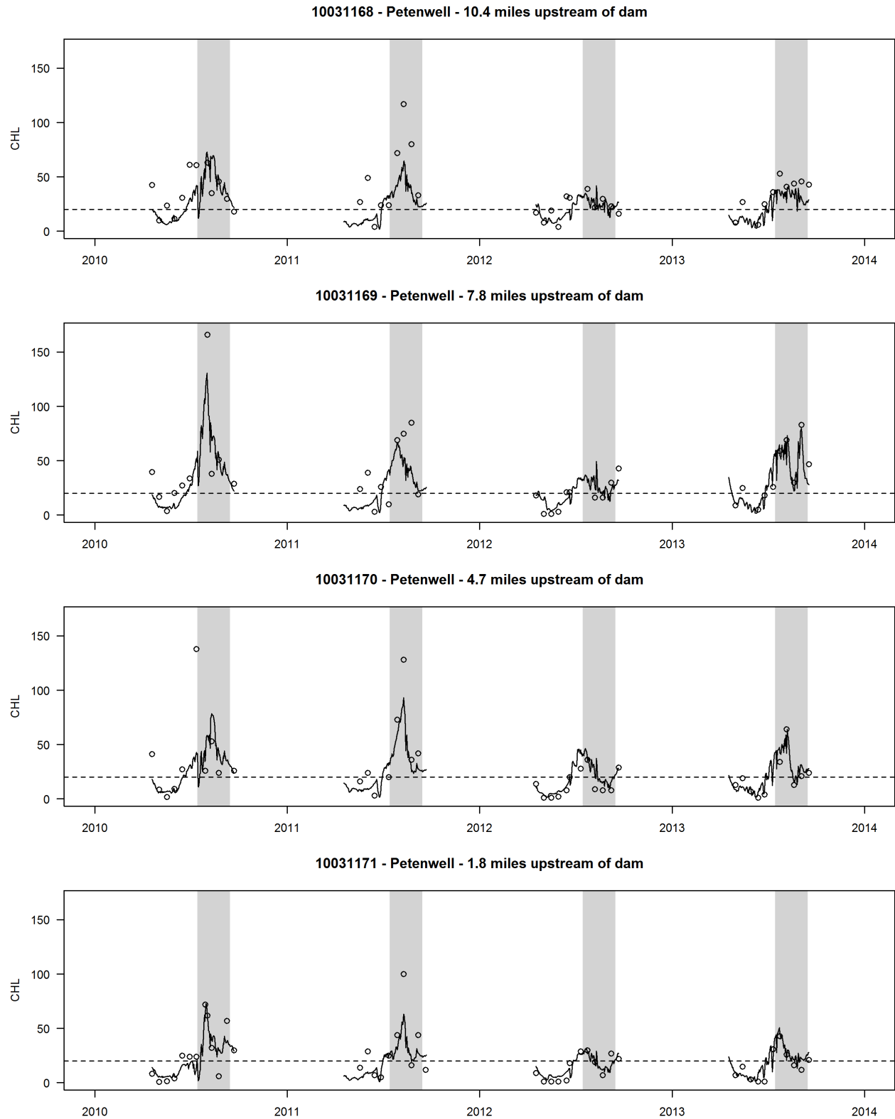
Figure 18. Observed (circles) and simulated (lines) chlorophyll a ( \mu\text{g/L} ) in Petenwell Lake. Dashed line is recreational chlorophyll a target ( 20 \mu\text{g/L} ). Shaded areas are chlorophyll a assessment periods.
