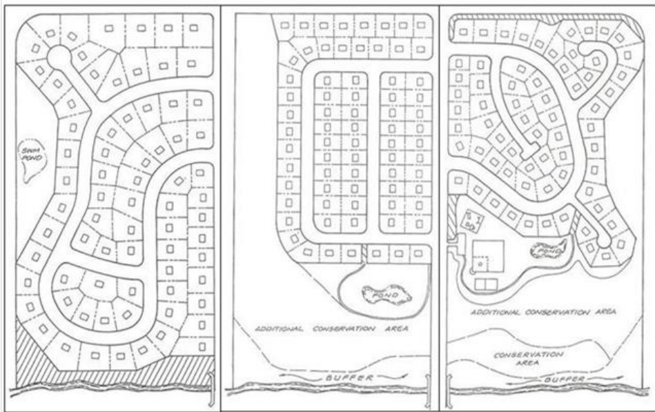
Figure 12: A conventional subdivision (left - 72 lots) with alternative layouts (center - 72 lots; right - 66 lots) implementing open space design.
