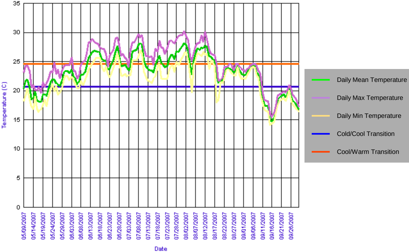
Mean/Min/Max Daily Temperatures
