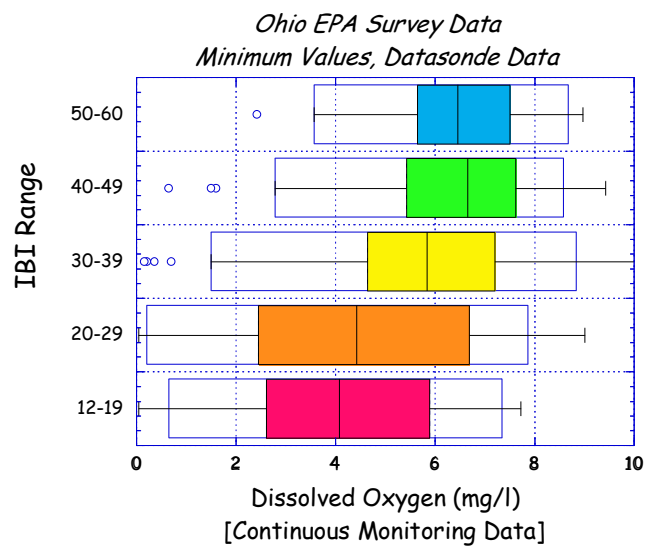
FIGURE 6-2. Box plots of minimum dissolved oxygen concentrations by IBI ranges for continuous monitoring data at all locations monitored in 1988 and 1994. IBI ranges are: 50-60 (exceptional, EWH); 40-49 (good, WWH), 30-39 (fair); 20-29 (poor); 12-19 (very poor).
