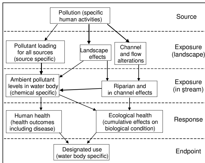
FIGURE 1-4. Modification of the NRC “position of the criterion” concept (Figure F-1) showing the causal sequence from indicators of stress, exposure, and response in relation to point and nonpoint source impacts, specific types of criteria, and designated uses that define the endpoints of interest to society (after Karr and Yoder 2004).
