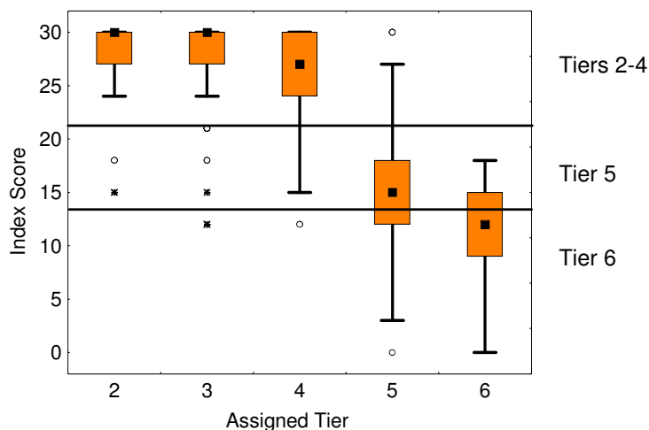
FIGURE 3-5. Hypothetical example of biotic index scores of sites assigned to BCG tiers, where the index is unable to discriminate tiers.
