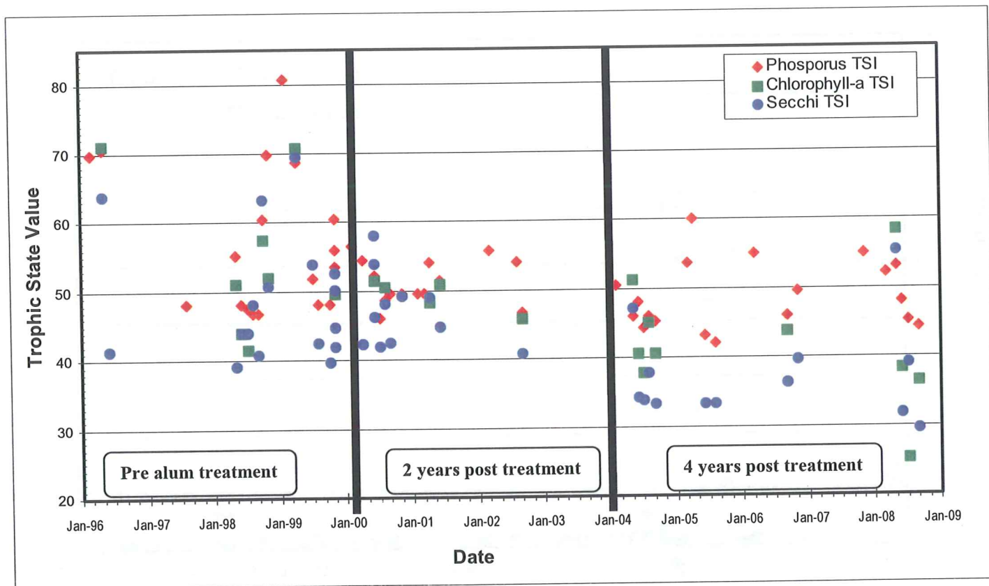
Figure 5. Bass Lake trophic state index values
