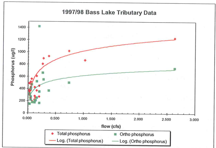
Figure 2. Relationship between phosphorus concentration and flow for the Bass Lake inlet.
